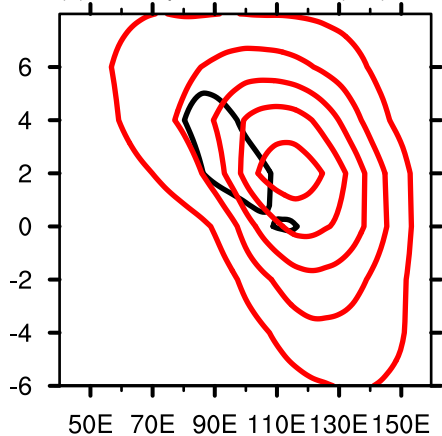
(c) Rossby and IG wave (SH)-EK
