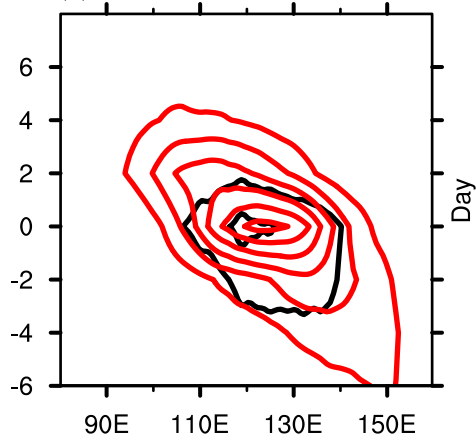
(b) IG and MRG wave- V^2
