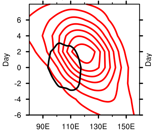
(a) Rossby and Kelvin wave- U^2
