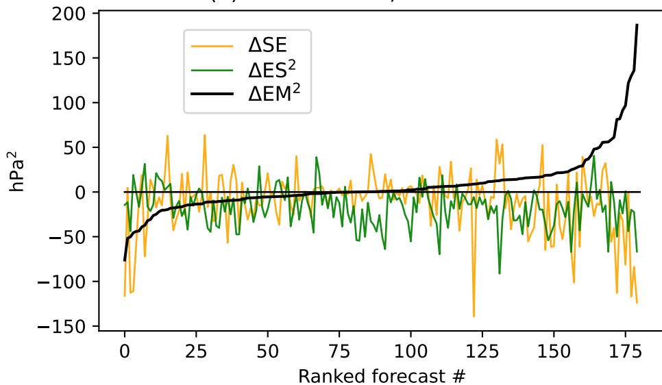
(c) Europe: \Delta EM^2 , \Delta ES^2 and \Delta SE
