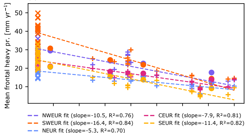
(a) Cold fronts
