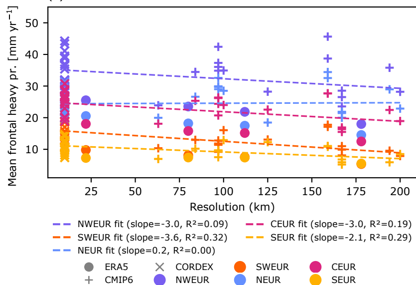
(b) Warm fronts
