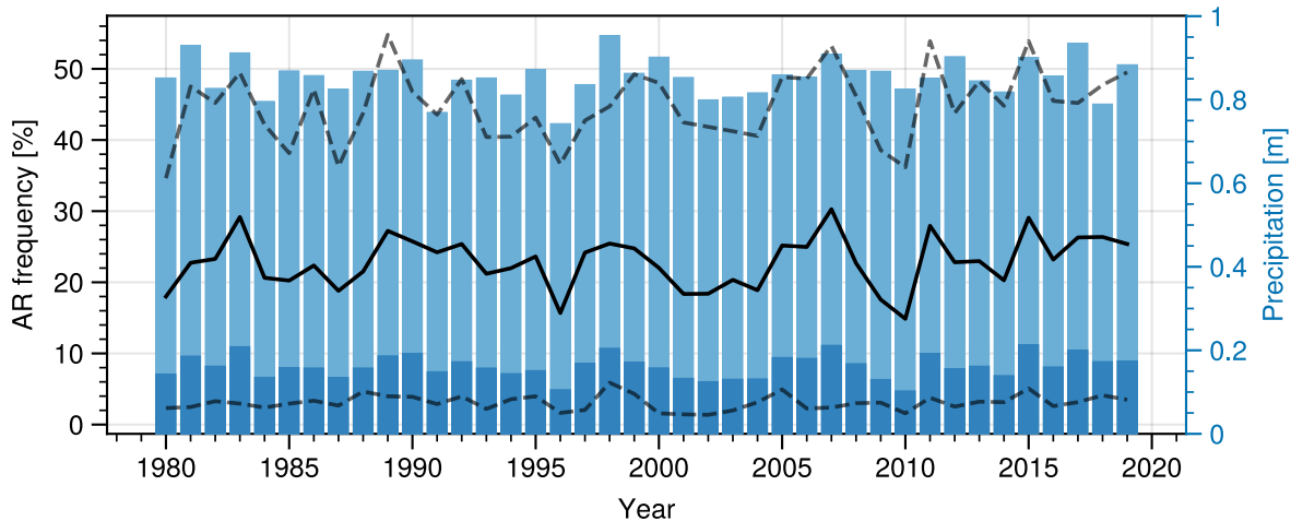
Total annual AR frequency and average annual precipitation over Scandinavia
