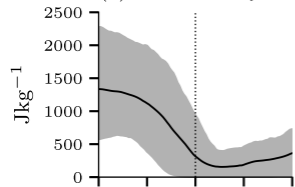
(c) Adiabatic
