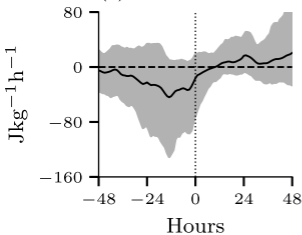
(c) Adiabatic
