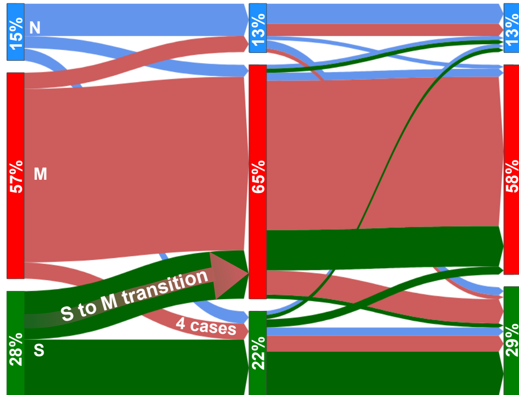
(b) Extreme jet streaks (92 cases)
