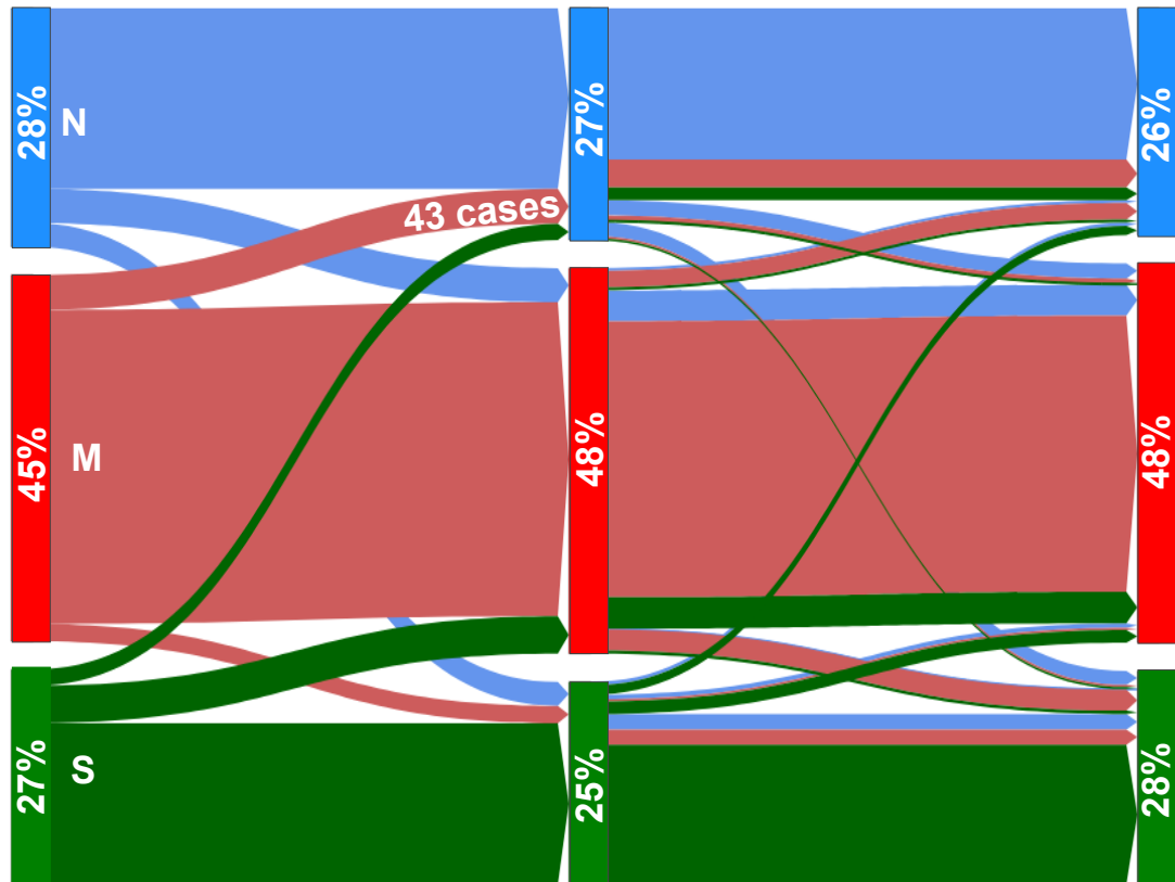
(a) All jet streaks (1050 cases)
