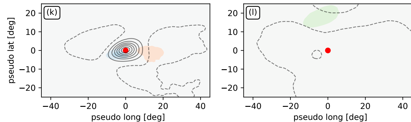
Wet perturbation & none/suppressed
