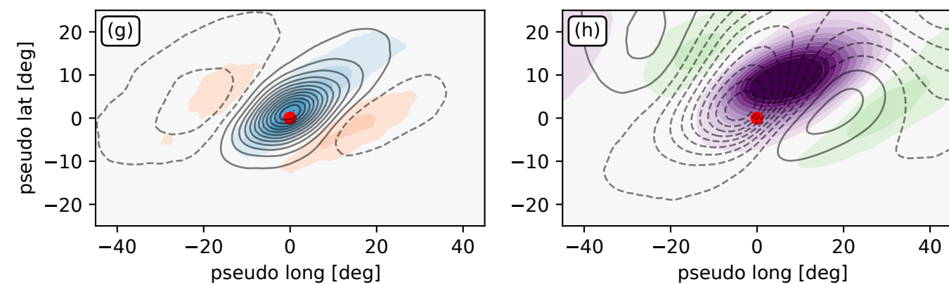
Wet perturbation & PV anticyclonic
