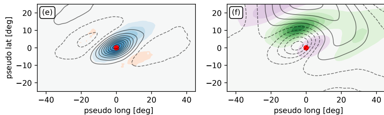
Wet perturbation & PV cyclonic
