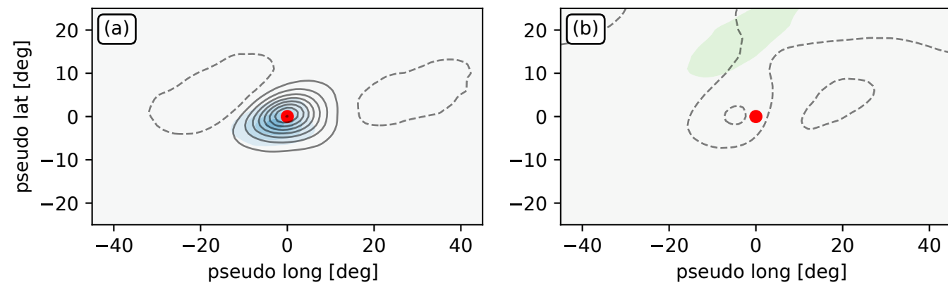
All wet perturbations
