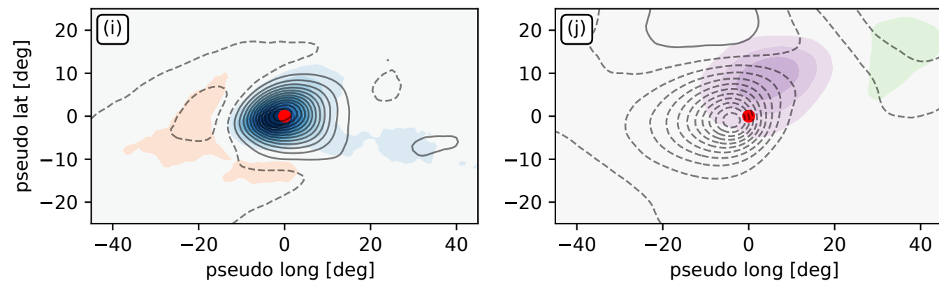
Wet perturbation & monsoon LPS
