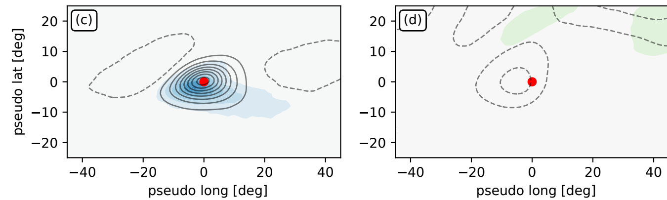
Wet perturbation & CCTW active
