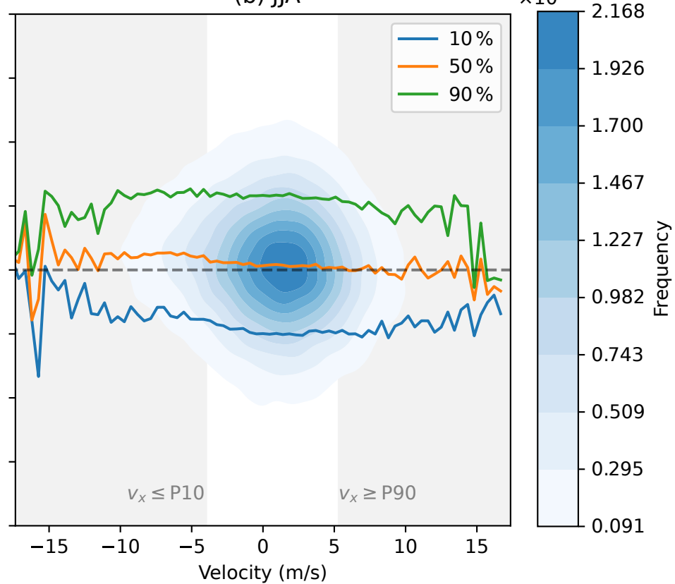
(b) JJA
