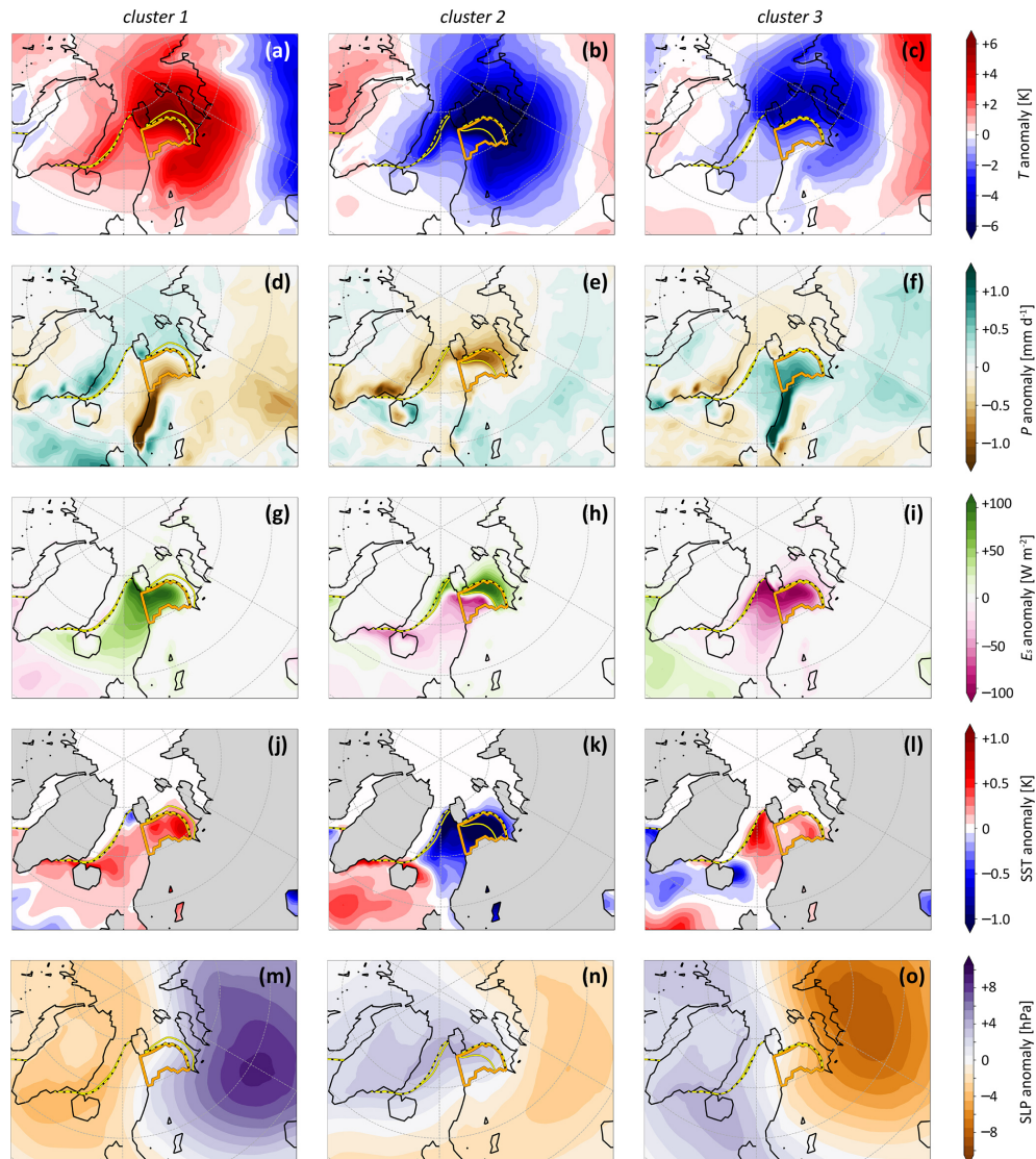
Figure 2. Seasonal anomalies of (a–c) T ( T^* , in K), (d–f) P ( P^* , in \text{mm d}^{-1} ), (g–i) E_S ( E_S^* , in \text{W m}^{-2} ), (j–l) SST ( \text{SST}^* , in K), and (m–o) SLP ( \text{SLP}^* , in hPa) for extreme winters in cluster 1 (left column), cluster 2 (middle column), and cluster 3 (right column) in S2000. The solid yellow line shows the mean sea ice edge for the respective cluster, and the dashed yellow–black line shows the climatological sea ice edge. The BS region is shown by the orange contour.
