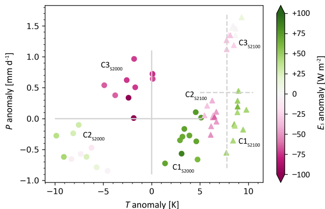
Figure 6. Seasonal anomalies with respect to S2000 of T (in K) along the x axis and P (in \text{mm d}^{-1} ) along the y axis for extreme winter clusters in S2000 (dots) and S2100 (triangles). Grey lines show climatological mean T and P values in this relative phase space for S2000 (solid) and S2100 (dashed). Markers are colored by seasonal anomalies of E_s (in \text{W m}^{-2} ). Note that for E_s shown anomalies are relative to the respective climatology.
