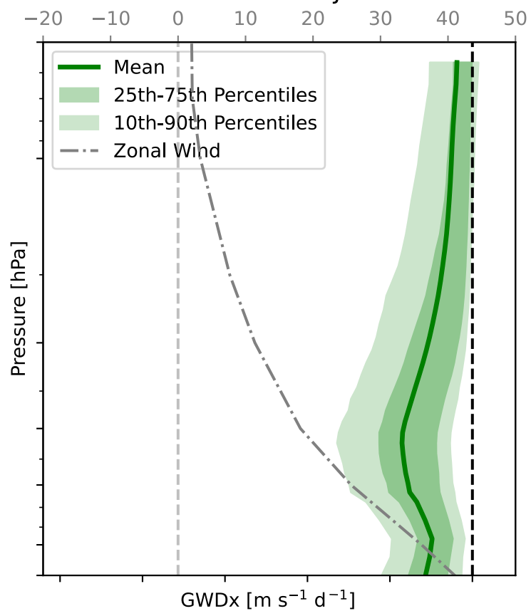
East Asia DJF
