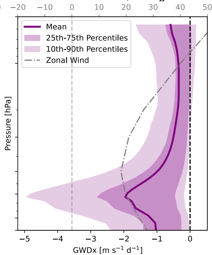
Southern Andes, north JJA
