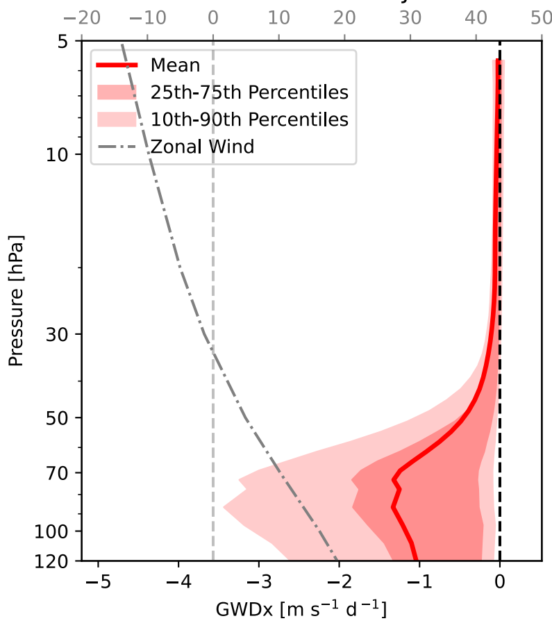
Southern Andes DJF
