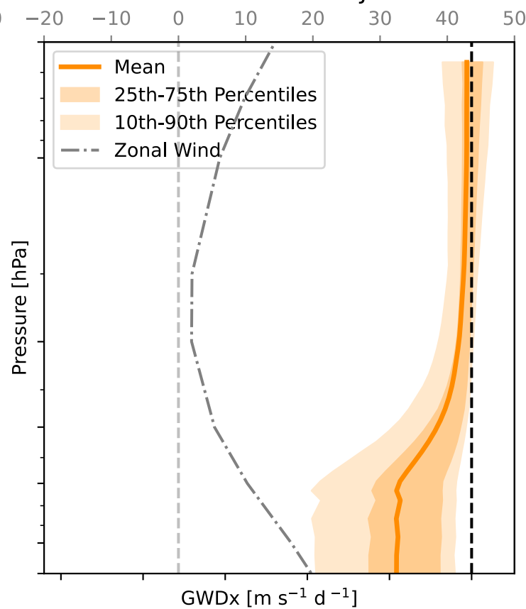
West America DJF
