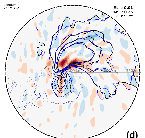
Kinematic frontogenesis (deformation + divergence)
