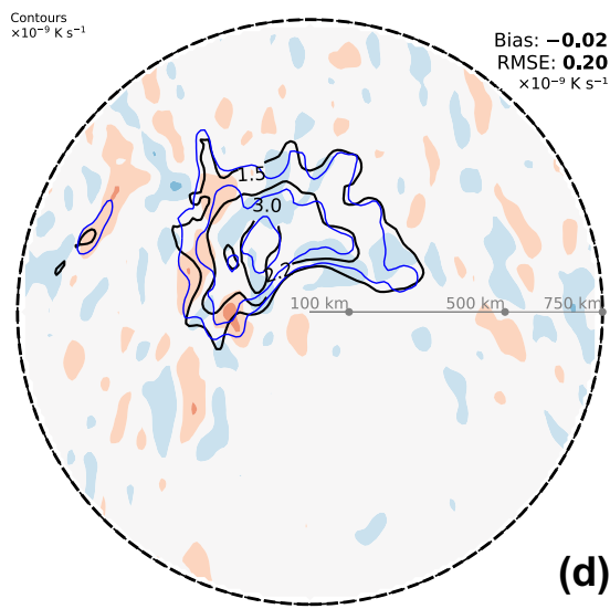
Kinematic frontogenesis (deformation + divergence)
