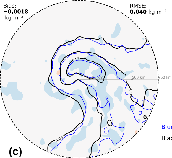
Composite TCLW Bias ( \text{kg m}^{-2} )
