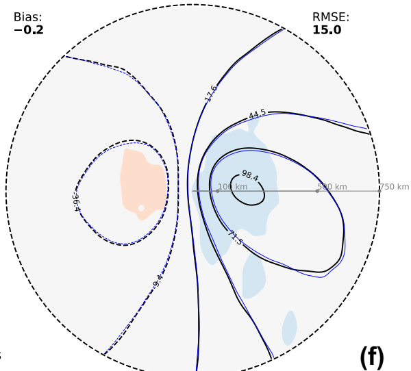
Composite cross-motion WVF Bias ( \text{kg m}^{-1} \text{ s}^{-1} )
