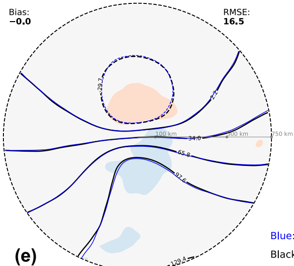
Composite along-motion WVF Bias ( \text{kg m}^{-1} \text{ s}^{-1} )
