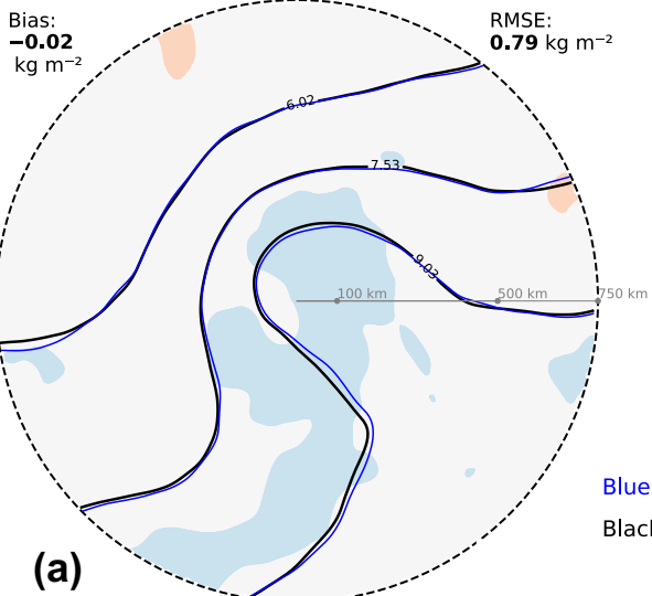
Composite TCWV Bias ( \text{kg m}^{-2} )
