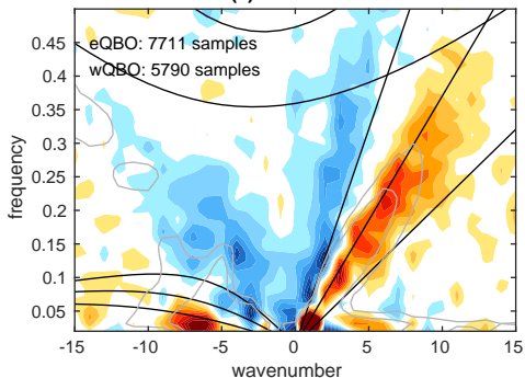
(c) MIROC6
