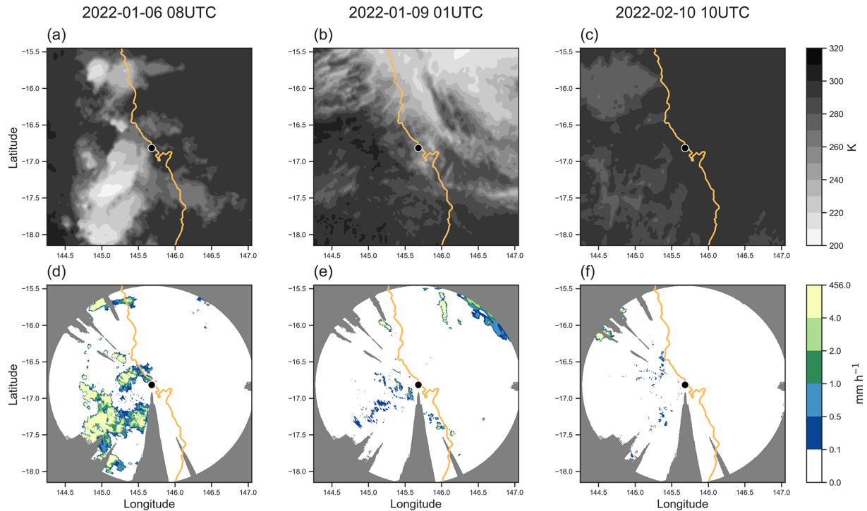
Figure 2. Snapshots of the cloud fields from satellite channel 13 BT and Cairns radar rain rate fields in UTC for: (a, d) 6 January 2022 08:00; (b, e) 9 January 2022 01:00; and (c, f) 10 February 2022 10:00. All plots show the Cairns radar domain, with the Queensland coastline shown in orange (land on left). Black markers indicate the Cairns radar site location. Cloud BT is shown in filled gray-scale contours where white indicates colder BTs, and black indicates warmer BTs. Rain rate in (d, e, f) is shaded in color, with dark gray shading indicating regions where no observations are taken (i.e. the corners of the Constant Altitude Plan Position Indicator radar retrieval grid) or masked (due to radar beam blockage).
