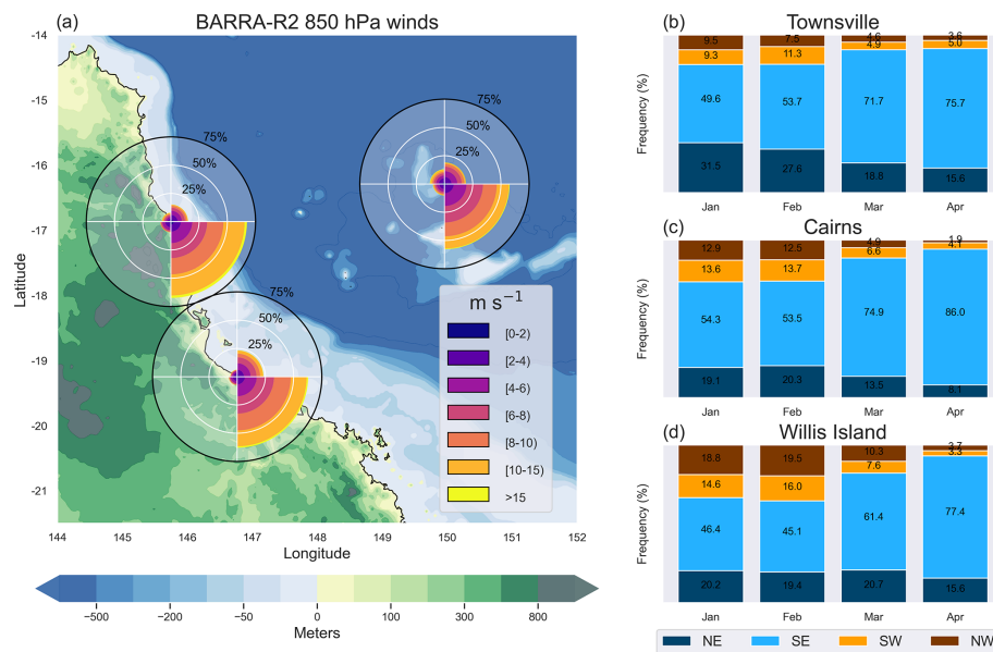
Figure 3. (a) Polar histograms over the CBS for BARRA-R2 850 hPa wind regimes defined in Sect. 2.2. Bar length indicates wind direction frequency, and colours indicate the corresponding wind speeds in \text{m s}^{-1} . (b, c, d) shows the monthly regime frequency for Townsville, Cairns and Willis Island. BARRA-R2 850 hPa winds are averaged over each site's radar domain (see Fig. 1) for the CBS over the period 1979–2024.
