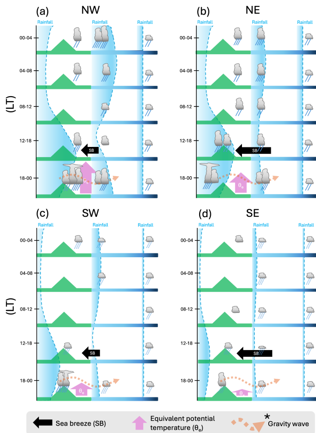
Figure 9. Hypothesized mechanisms for each wind regime (a, b, c, d) cloud BT and rainfall observations. Each panel shows time (Local Time) along the left column, corresponding to mean rainfall changes throughout the day (blue shading). Five distinct stages are shown (nighttime, early morning, morning, afternoon, and evening), with land and topographical features on the left (a general feature of the north-east Queensland coastline), the coastal ocean in the center, and the open ocean on the right. Upward pink arrows indicate the relative size of peak equivalent potential temperatures for each wind regime. The afternoon land sea breeze is shown by black arrows with relative maximum wind speeds indicated by arrow length (see Fig. A3). * Mechanism inferred from estimated propagation speeds consistent with gravity wave propagation in literature – dashed orange oscillating arrows indicate the nighttime offshore propagation of convection induced by gravity waves.
