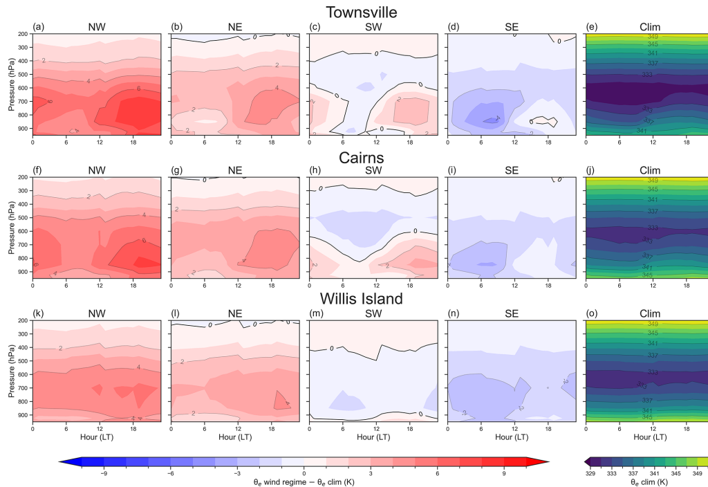
Figure 5. Diurnal \theta_e profile difference plots between wind regimes and a smoothed rolling mean climatology over the CBS for (a, b, c, d) Townsville, (f, g, h, i) Cairns, and (k, l, m, n) Willis Island. (e, j, o) show the CBS mean \theta_e diurnal profiles over the period 1979–2024 (January–April). Note that the “Clim” panels for each site (e, j, o) represent the CBS climatological mean for reference, and are not equivalent to the smoothed rolling mean used in the difference plots (which varies at daily time resolution).
