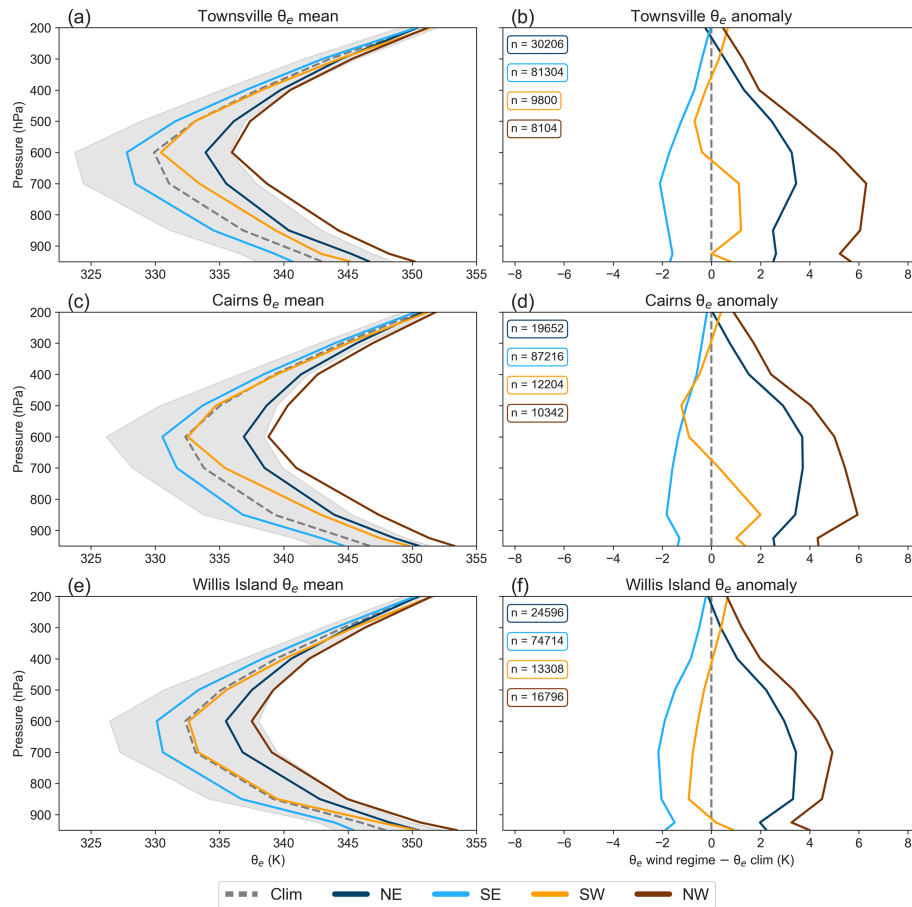
Figure 4. Mean and anomaly \theta_e profiles for Townsville (a, b), Cairns (c, d) and Willis Island (e, f) radar sites under each wind regime (north-easterly: NE, south-easterly: SE, south-westerly: SW, and north-westerly: NW) for the CBS over the period 1979–2024 from BARRA-R2. Anomaly plots are calculated by subtracting a smoothed rolling mean climatology from each timestep within the wind regime-classified periods, then averaging across all time steps within each regime to remove seasonal signals. Sample sizes for each site across all times are provided for each regime. Grey shading indicates the inter-quartile range of the \theta_e profile.
