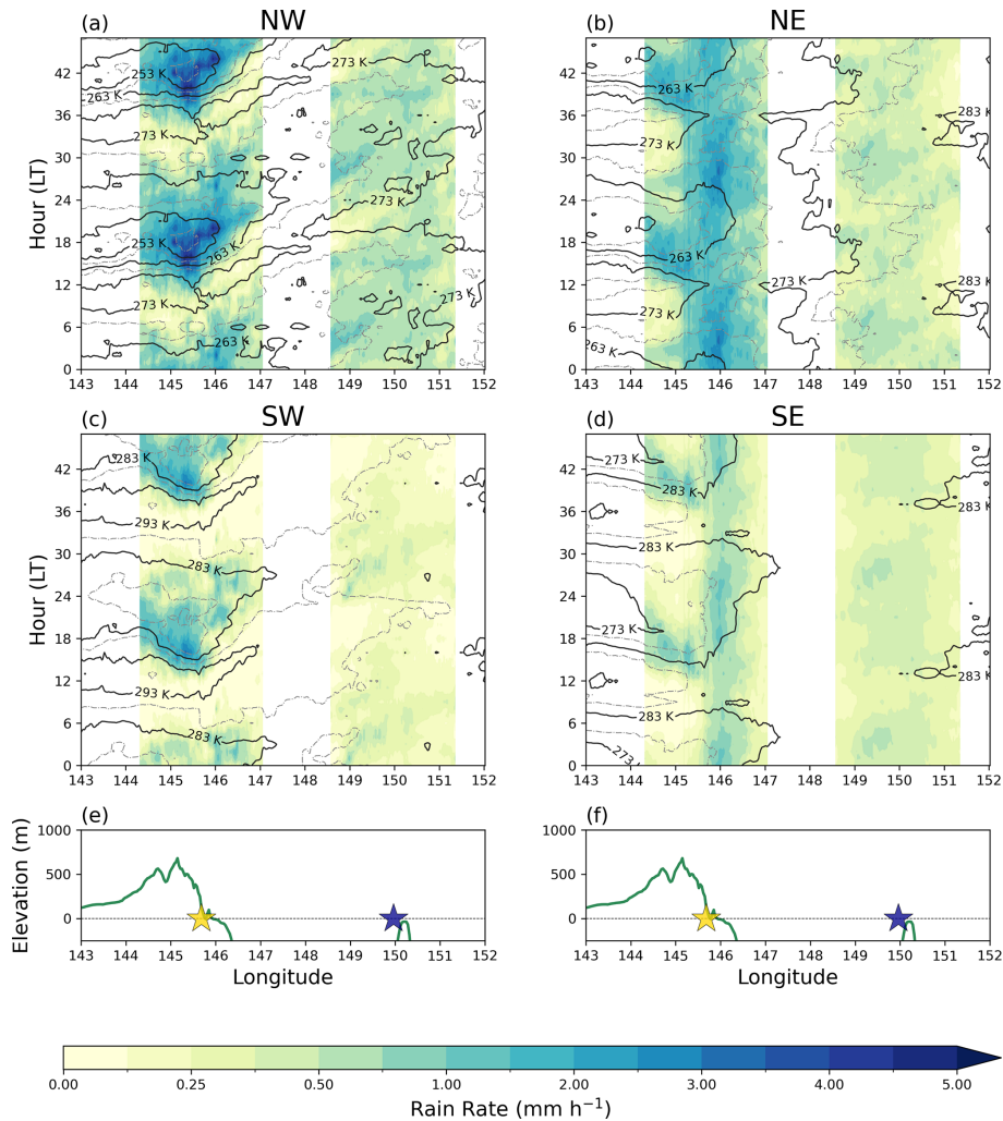
Figure 7. Hovmöller diagrams of cloud BT and rain intensity (including non-raining periods) for the longitudinal transect shown in Fig. 1. (a, b, c, d) show labeled cloud BT contours for 253, 263, 273, 283 and 293 K (with dashed gray contours every 5 K), along with rainfall data from the Cairns (left filled contours in each panel) and Willis Island radars (right filled contours) under each wind regime. The y axis (in LT) is repeated to show clear propagation of cloud BT and rainfall between the evening and morning. (e) shows elevation from NOAA National Geophysical Data Center (2006) averaged over the longitudinal transect, with this plot repeated in (f) for referral to the above panels. Yellow and blue stars indicate the longitude of the Cairns and Willis Island radar site respectively, with a black dashed line at 0 m elevation.
