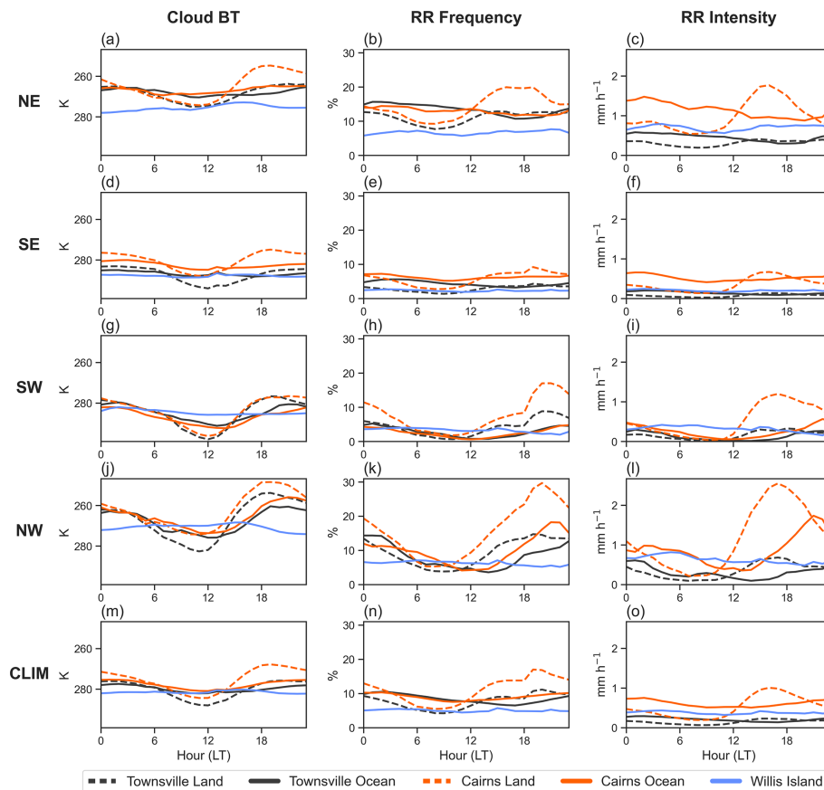
Figure 6. Diurnal cycle of Himawari-8 satellite BT ( 10.4\ \mu\text{m} infrared wavelength band; K), radar retrieved rainfall frequency (percentage of points greater than 0.1\ \text{mm h}^{-1} ) and intensity (mean rain rate \text{mm h}^{-1} ) calculated over the CBS for each wind regime and site. Each row shows the corresponding BT, rainfall frequency and rainfall intensity with consistent y-axes for each wind regime – with different colored lines for each site. Townsville and Cairns are separated into land (dashed) and ocean (solid) domains, associated with their radar coverage. The BT y-axis is inverted, so that peaks in the diurnal cycle indicate colder BTs. Rain intensity is calculated for all periods of valid data (not just raining periods).
