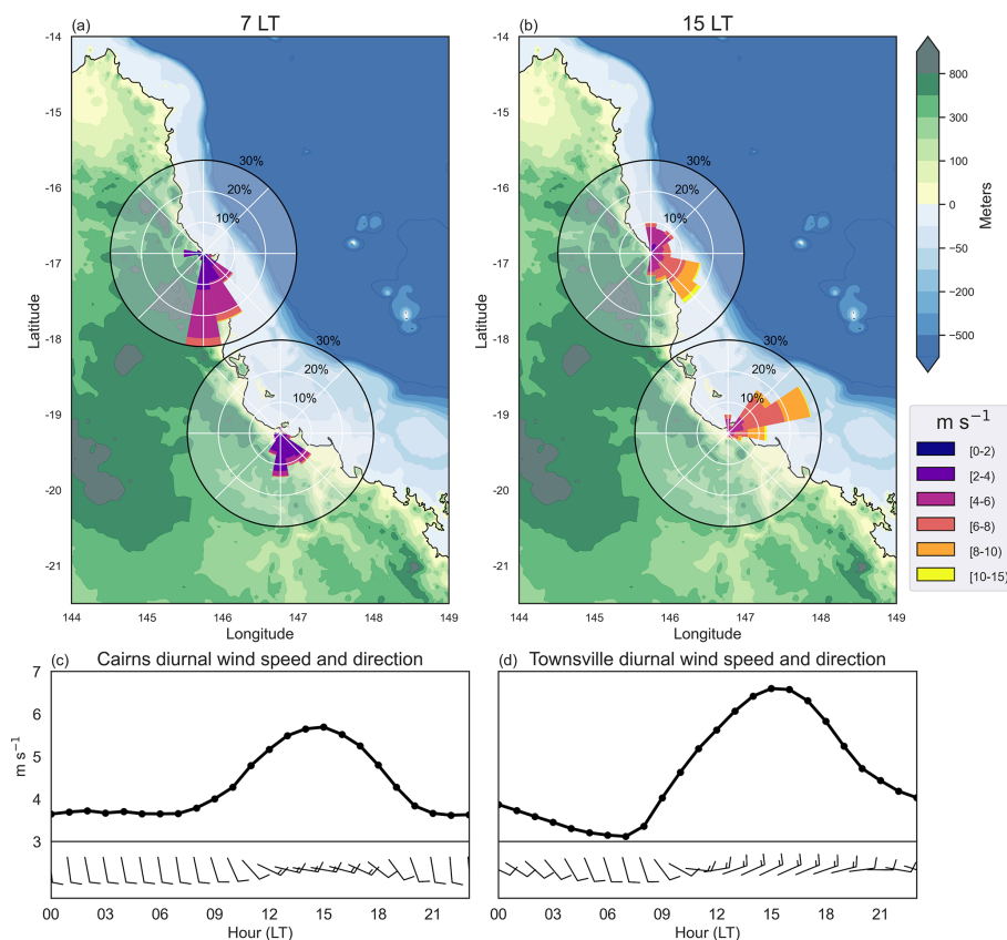
Figure 8. (a, b) Cairns and Townsville AWS surface winds. Wind roses show the surface wind frequency and magnitude at 07:00 and 15:00 LT. (c, d) show hourly averaged wind speed and direction (wind barbs; calculated using a circular mean) for each station.
