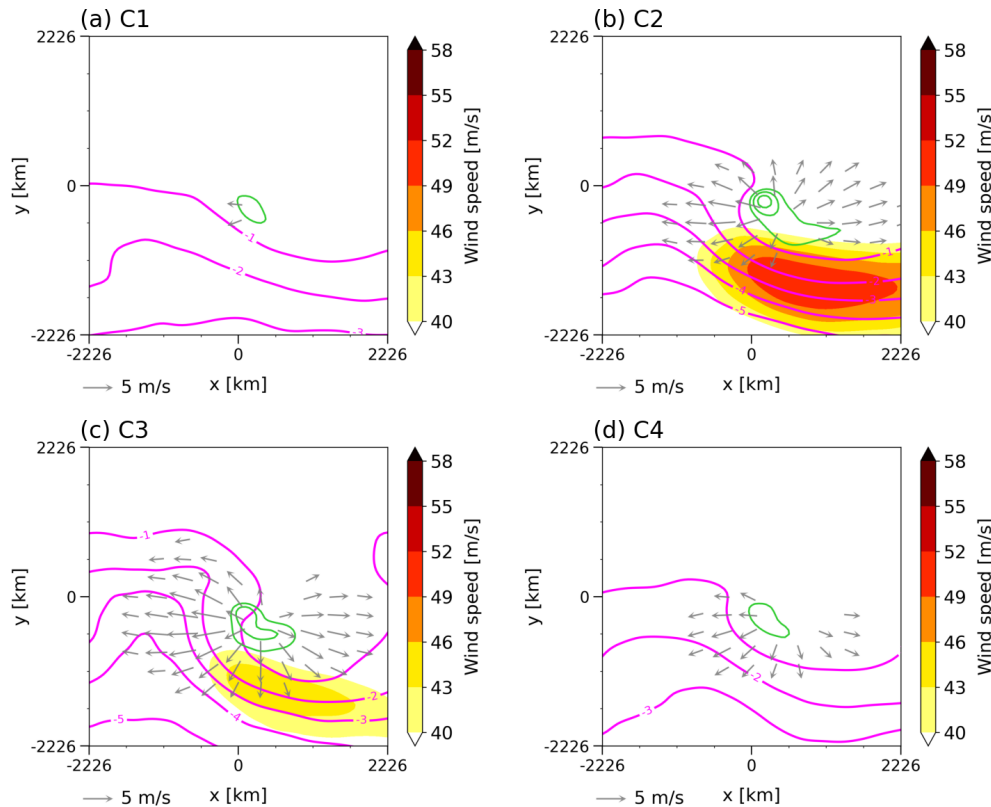
Figure 13. Composite fields at ET time for Clusters (a) 1, (b) 2, (c) 3, and (d) 4, showing PV (magenta contours every 1 PVU), wind speed (shaded as per the colourbar), divergent wind (arrows, only for vector > 2.5 \text{ m s}^{-1} ), and convergence of integrated water vapour transport on the condition of relative humidity greater than 80 % (as proxy for latent heat release, green contours every 10 \text{ kg m}^{-2} \text{ d}^{-1} ). The PV, wind speed, and divergent wind are vertically averaged between 200 and 300 hPa. The water vapour transport is integrated from 1000–500 hPa. Coordinates are in km relative to the cyclone centre. The bottom (right) of the composites aligns with south (east).
