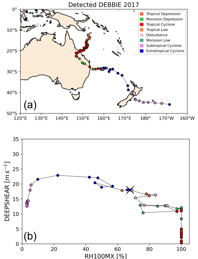
Figure 1. An example of ET identification in the SyCLOPS framework. (a) Objectively-detected TC Debbie 2017 and (b) its corresponding RH100MAX-DEEPSHEAR phase space. Types of cyclones are marked by various colours. In panel (b), the black cross marks the ET time, and the supersaturation of RH100MAX is converted to 100 %.
