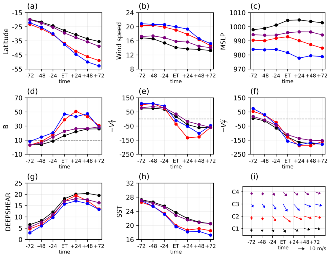
Figure 10. Evolution of (a) latitude, (b) wind speed (in \text{m s}^{-1} ), (c) central pressure (MSLP, in hPa), (d) B , (e) -V_T^L , (f) -V_T^U , (g) vertical wind shear (DEEPSHEAR, in \text{m s}^{-1} ), (h) SST (in ^{\circ}\text{C} ), and (i) cyclone speed (in \text{m s}^{-1} ) and direction from 72 h before to 72 h after ET for individual clusters. Dashed horizontal lines in (d–f) mark the thresholds for ET in the CPS framework. Clusters 1, 2, 3, and 4 are marked by various colors (black, red, blue, and purple). The bottom (right) aligns with south (east) in (g).
