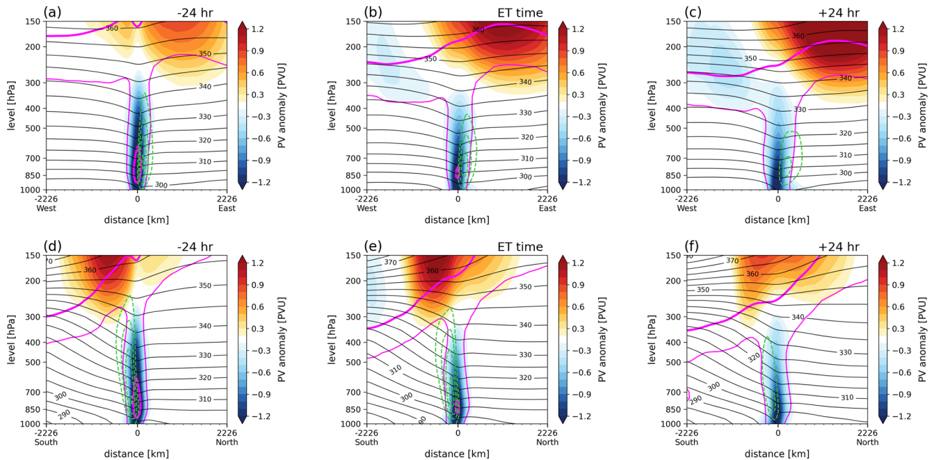
Figure 7. Lead-lag cross section composites in (a–c) west–east and (d–f) south–north direction for PV anomaly (shaded as per the colourbar), PV (magenta contours at -2 and -0.7 PVU), potential temperature (black contours every 5 K), and vertical velocity (dashed green contours every -0.1 \text{ Pa s}^{-1} , only negative values displayed). PV anomalies are calculated relative to the 30 d running mean. A thick magenta line highlights the -2 PVU contour. Coordinates are in km relative to the cyclone centre.
