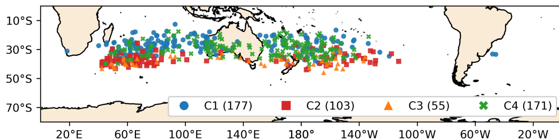
Figure 9. Geographic locations of TCs at ET time for clusters 1, 2, 3, and 4. Numbers in parentheses denote the number of ET events in each cluster.
