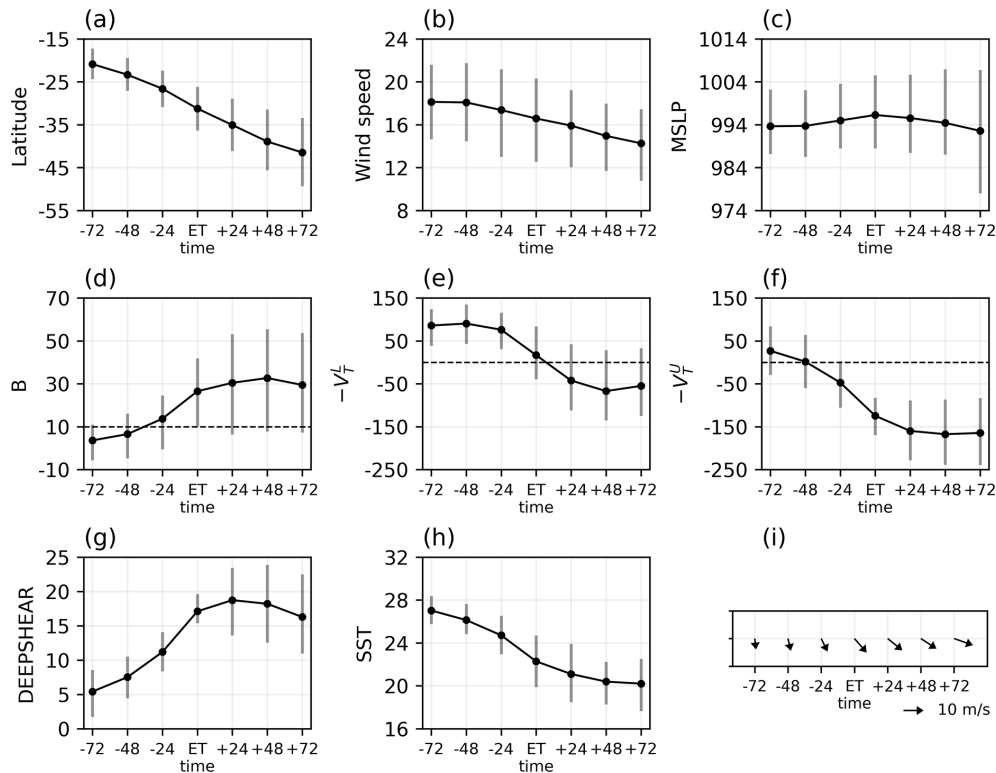
Figure 5. Evolution of (a) latitude, (b) wind speed (in \text{m s}^{-1} ), (c) central pressure (MSLP, in hPa), (d) B , (e) -V_T^L , (f) -V_T^U , (g) vertical wind shear (DEEPSHEAR, in \text{m s}^{-1} ), (h) SST (in ^{\circ}\text{C} ), and (i) cyclone speed (in \text{m s}^{-1} ) and direction from 72 h before to 72 h after ET. Dots denote the mean, and whiskers mark the 25th and 75th percentiles. Dashed horizontal lines in (d–f) mark the thresholds for ET definition in the CPS framework. The bottom (right) aligns with south (east) in (i).
