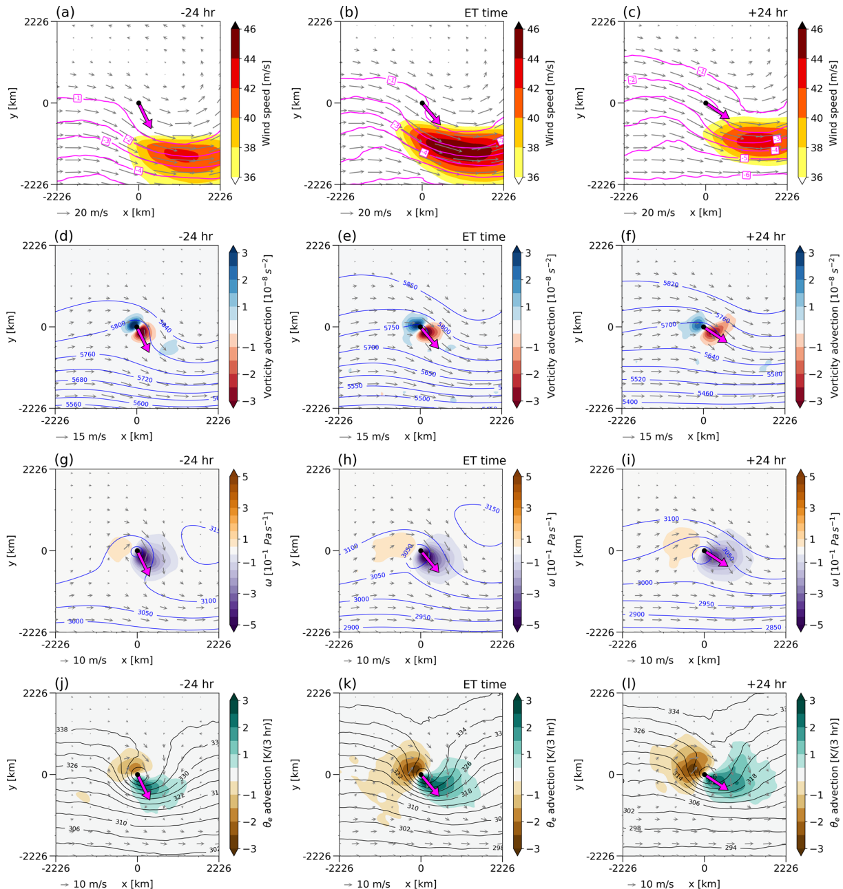
Figure 6. Lead-lag composites of (a–c) wind speed (shaded as per the colourbar), wind (arrows), and PV (magenta contours every 1 PVU; 1 \text{ PVU} = 10^{-6} \text{ K m}^2 \text{ kg}^{-1} \text{ s}^{-1} ) at 200 hPa; (d–f) vorticity advection (shaded as per the colourbar), wind (arrows), and geopotential height (blue contours every 50 m) at 500 hPa; (g–i) vertical velocity (shaded as per the colourbar), wind (arrows), and geopotential height (blue contours every 50 m) at 700 hPa; and (j–l) advection of equivalent potential temperature (shaded as per the colourbar), wind (arrows), and equivalent potential temperature (black contours every 4 K) at 850 hPa. Magenta arrows indicate the direction of the cyclone. Coordinates are in km relative to the cyclone centre. The bottom (right) of the composites aligns with south (east).
