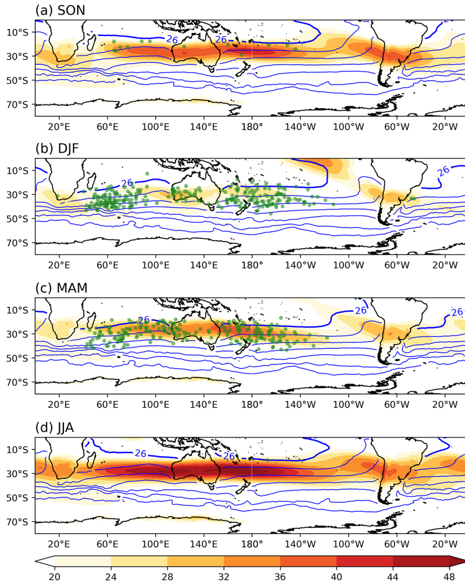
Figure 4. Seasonal climatologies of vertical wind shear (in \text{m s}^{-1} ; shaded as per the colourbar) and SST (in ^{\circ}\text{C} ; blue contours every 4^{\circ}\text{C} starting from 2^{\circ}\text{C} ) for (a) September–October–November (SON), (b) December–January–February (DJF), (c) March–April–May (MAM), and (d) June–July–August (JJA) over the Southern Hemisphere. Green dots mark the positions of ET. A thick blue line highlights the 26^{\circ}\text{C} contour. The seasonal climatologies are based on the period 1979–2021.
