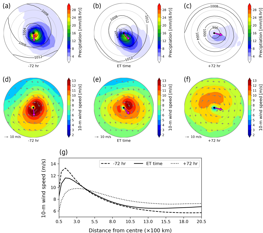
Figure 8. Composites of (a–c) 6 hourly accumulated precipitation (shaded as per the colourbar) and MSLP (black contours every 4 hPa), (d–f) 10 m wind (grey arrows) and wind speed (shaded as per the colourbar), and (g) azimuthally-averaged 10 m wind speed from 72 h before to 72 h after ET. Each panel has a radius of 1000 km, with grey dashed rings plotted every 250 km from the centre. The magenta arrow indicates the direction of the cyclone. The composites are not rotated, and the bottom (right) of the composites aligns with south (east).
