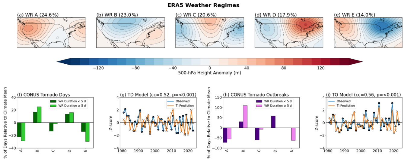
Figure 1. 500hPa anomaly patterns of WRs A–E with long-term frequency indicated in panel title (a–e). ERA5 tornado day (f) and tornado outbreak (h) CONUS probability anomalies for persistent ( \geq 5 d; light green, pink) and nonpersistent ( < 5 d; dark green, indigo) WRs. Time series of standardized tornado days (g) and tornado outbreak days (i) from the observation (blue) and estimation of the empirical modeling (red). Spearman rank correlation and p value are indicated in panels (g) and (i).
