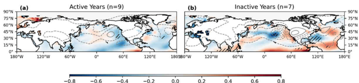
Figure 7. April composite SST anomalies for active and inactive tornado outbreak years. Hatching indicates significant SST anomalies ( p \leq 0.05 ) using a one-sample, two-sided t -test. 500hPa anomalies are shown in gray contours. Sample sizes are included in each panel title.
