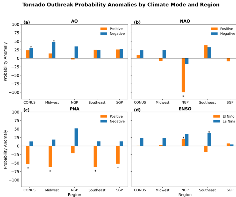
Figure 5. TO probability anomalies by region and climate mode: AO (a), NAO (b), PNA (c), and ENSO (d). Asterisks represent significant anomalies ( p \leq 0.05 ) based on a Monte Carlo test with 10 000 resamples of each regions' data.
