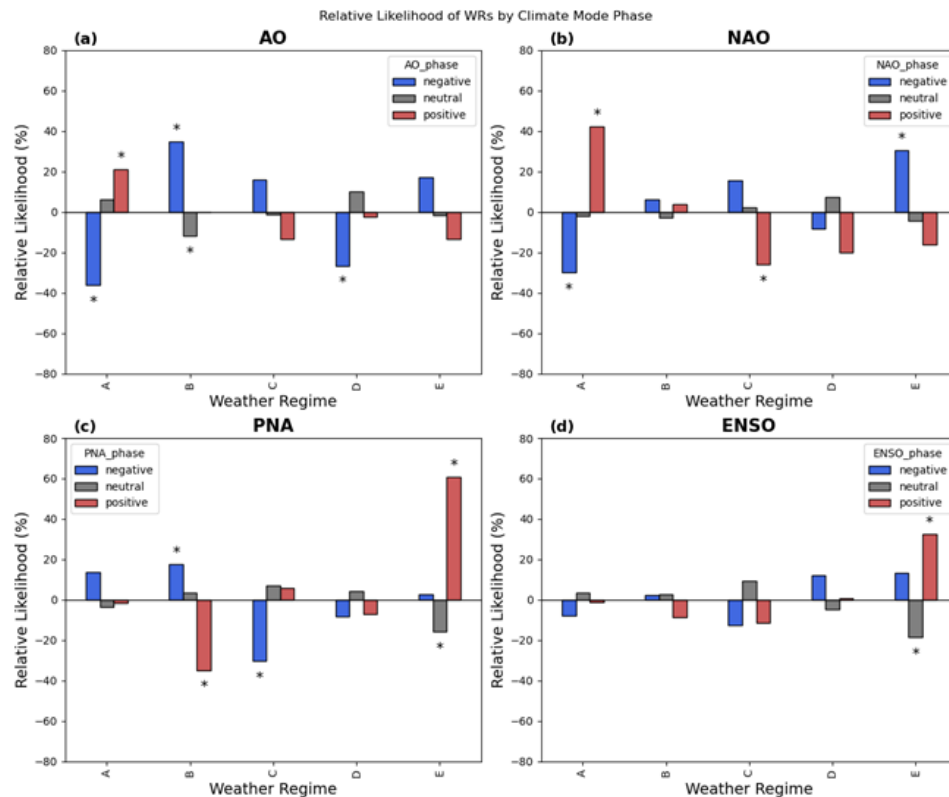
Figure 6. Relative likelihood (RL: %) of each WR in different phases of AO (a), NAO (b), PNA (c), and ENSO (d). An asterisk indicates that the frequency is significantly different ( p \leq 0.05 ) from climatology using a scipy binomial test. Black horizontal line representing the climatological frequency is at RL = 0.0.
