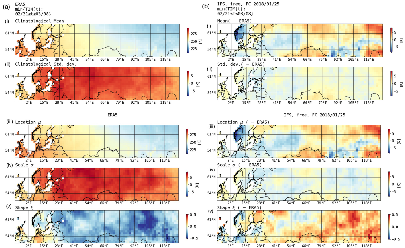
Figure 3. Statistical summary maps of surface temperature minima in the 16 d interval from 21 February. (a) Shows values over the “ensemble” of years from 1980–2020 in ERA5, (b) shows values from the IFS free ensemble for SSWFeb18 initialized on 25 January 2018 (early), as a difference relative to ERA5. Panels (i) show mean minima, (ii) standard deviation of minima, and (iii), (iv), and (v) show GEV parameters of location, scale, and shape, respectively. The similarity in spatial patterns between “normal” summary statistics (mean, standard deviation) with analogous GEV summary statistics (location, scale) affirms qualitatively that the GEV distribution is an appropriate parametric choice. The small differences in shown in panels (b) (i)–(iv), relative to corresponding panels (a) (i)–(iv), affirm qualitatively that the early forecast is not highly skillful, but statistically accurate with respect to climatology. Only the shape parameter \xi differs between ERA5 and IFS on the same order as its ERA5 value, which reflects its high sensitivity to the far tail.
