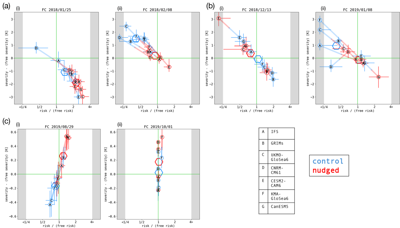
Figure 6. Relative risks (RRs) and quantile shifts (QSs). For each case study of extreme temperatures ( a : SSWFeb18, b : SSWJan19, and c : SSWSep19), for each initialization date (i: early and ii: late), for both forcing experiments (blue: control and red: nudged ), and for each model (represented by circled letters, as per the key), the response to forcing is plotted in a two-dimensional space (RR, QS), both defined with respect to the free experiment as a baseline (Fig. 5a and b(iv) are the IFS-only versions for SSWFeb18). Thick shaded lines connect each model’s free and control responses, to help see patterns in the direction of influence. Multi-model means are represented by the large hexagons, with the relative-risk component being a geometric mean (taken in log space).
