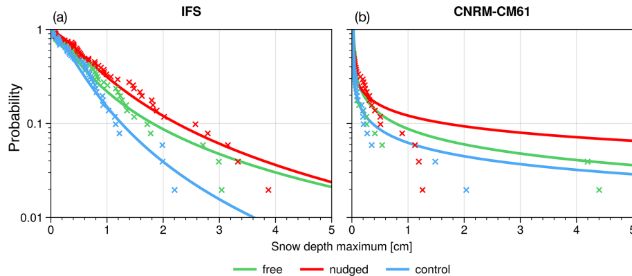
Figure 8. Empirical risk functions, calculated as in Fig. 4a(i), but for maximum snow depth over the southern UK and Ireland, for IFS (a) and CNRM-CM6-1 (b). Values are shown for the 25 January 2018 initialization, with the same time window as in Table 1. Crosses indicate risk calculated from individual ensemble members, solid lines show GEV fits.
