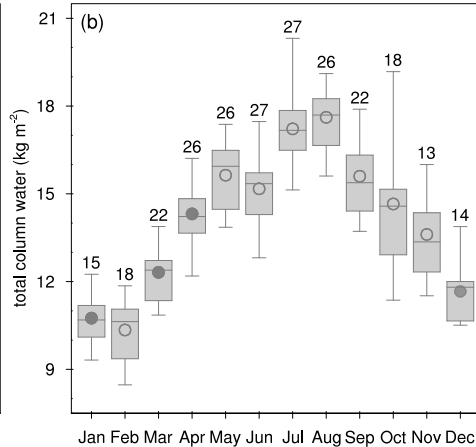
neutral ENSO
