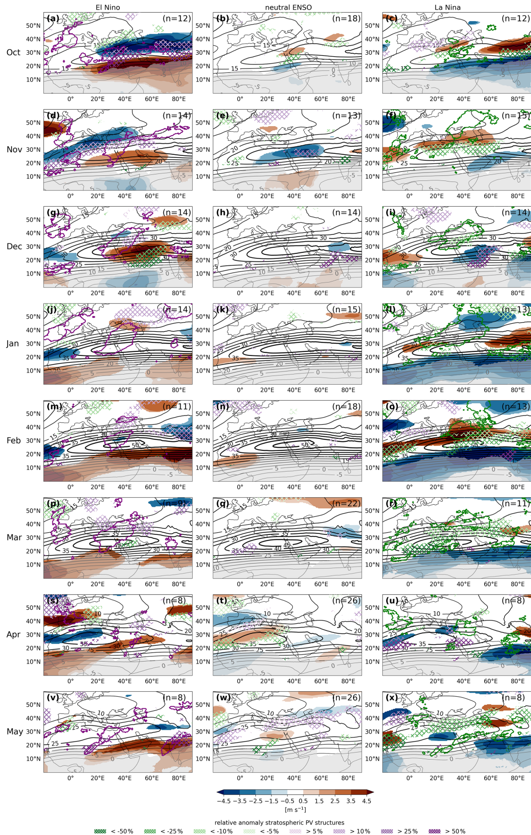
Figure A2. As Fig. 5a, c but for individual months from October to May in rows and the ENSO phases – warm, neutral, and cold – in columns. The ENSO phases are defined based on 3-monthly running mean SST anomalies in the Niño3.4 region. Sample sizes are indicated in text in the top right corner of each panel.
