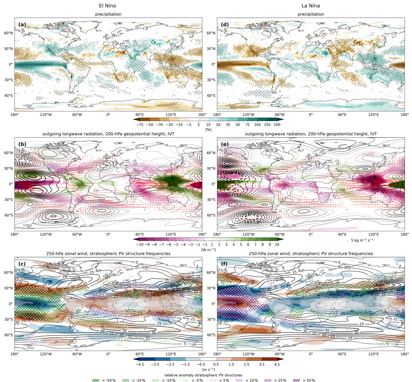
Figure 11. Composites of cool-season anomalies for (a–c) El-Niño and (d–f) La Niña. (a, d) Relative precipitation anomalies (%) from MSWEP, (b, e) top thermal radiation ( \text{W m}^{-2} ) in colors with negative anomalies corresponding to enhanced tropical convection and positive anomalies to reduced convection, 200 hPa geopotential height meter contours at 4 gpm intervals with positive and negative values in solid and dashed lines, respectively, and vertically integrated horizontal water vapor transport ( \text{kg m}^{-1} \text{s}^{-1} ) in red vectors, and (c, f) 250 hPa zonal wind anomalies ( \text{m s}^{-1} ) in colors, the climatological mean of 250 hPa zonal wind in contours at 5 \text{ m s}^{-1} intervals, and relative anomalies in stratospheric PV structure occurrences, aggregated over 300–350 K, in hatching, as indicated by the legend. Anomalies in top thermal radiation are only shown where considered significant at p < 0.05 and in zonal wind and Rossby wave breaking frequencies where considered significant at p < 0.1 .
