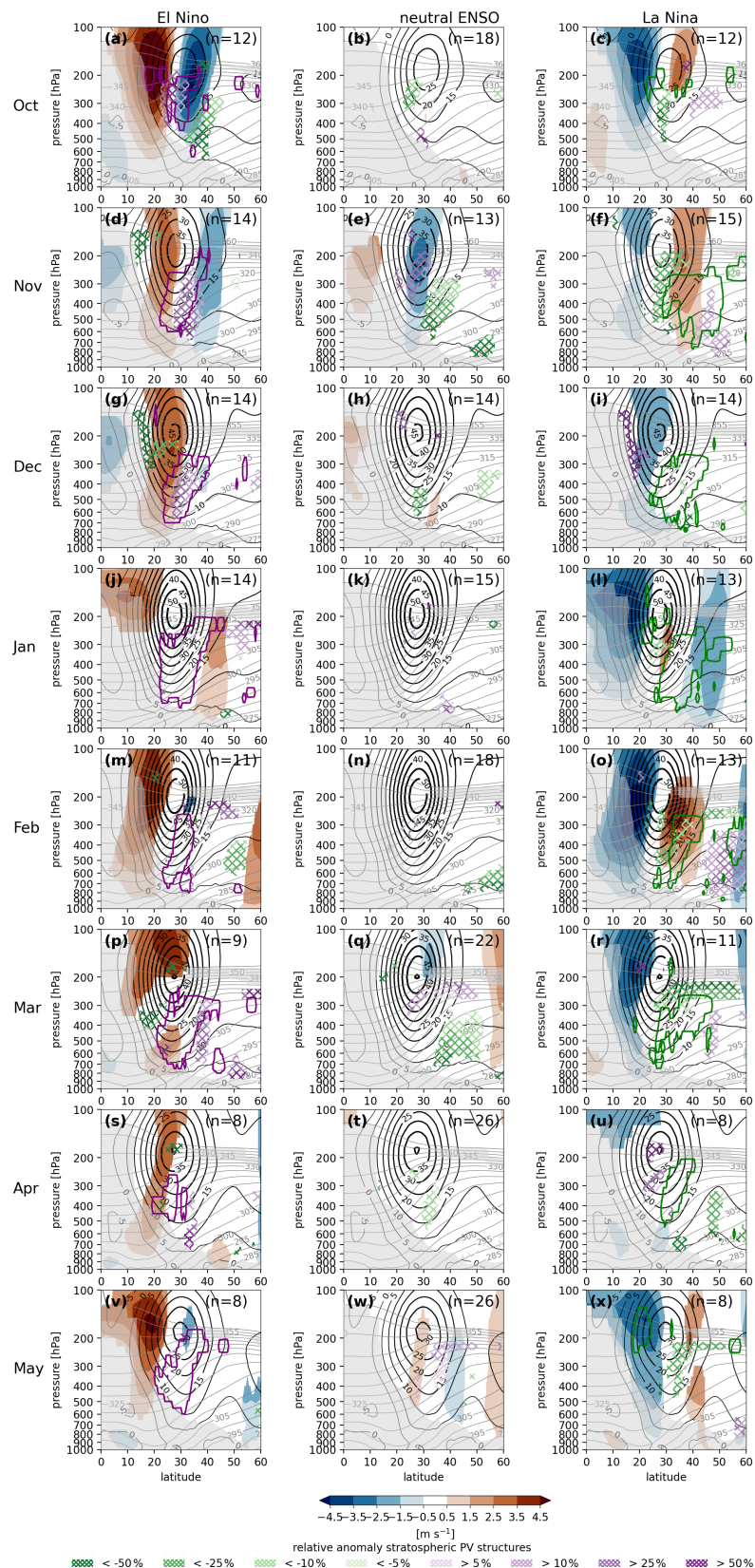
Figure A3. As Fig. 5b, d but for individual months from October to May in rows and the ENSO phases – warm, neutral, and cold – in columns. The ENSO phases are defined based on 3-monthly running mean SST anomalies in the Niño3.4 region. Sample sizes are indicated in text in the top right corner of each panel.
