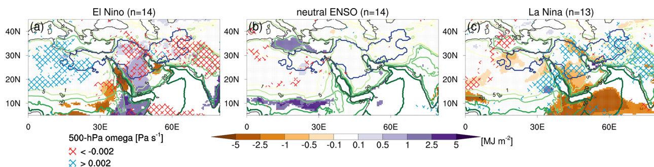
Figure 9. Composites of cool-season anomalies in I_{\max} [ \text{MJ m}^{-2} ] in colors for (a) El-Niño, (b) neutral ENSO, and (c) La Niña events. Yellow-green contours show the climatological distribution of I_{\max} at intervals of 1, 5, 20, 50, and 100 \text{MJ m}^{-2} . Red and blue hatching mark regions with anomalous 500 hPa omega falling below -0.002 \text{ Pa s}^{-1} (ascent) and exceeding 0.002 \text{ Pa s}^{-1} (descent). Anomalies in I_{\max} and 500 hPa omega are only plotted where significant at the p < 0.05 level. The numbers in the figure title indicate the number of samples for each ENSO phase, and the blue contour highlights the region of interest.
