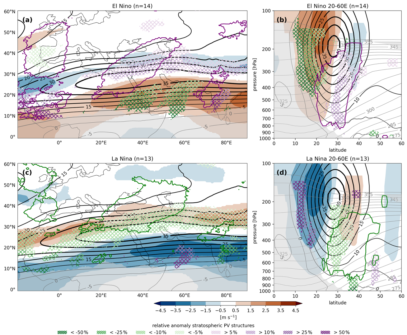
Figure 5. Composites of anomalies in cool-season zonal wind and Rossby wave breaking frequencies for (a, b) El Niño and (c, d) La Niña events. (a, c) 250 hPa zonal wind anomalies in colors and relative anomalies of stratospheric PV structure frequencies – aggregated over 300–350 K – in hatching, as indicated by the legend. (b, d) The zonal mean (20–60°E) zonal wind anomalies in colors and relative anomalies of stratospheric PV structure frequencies in hatching at pressure levels interpolated from data on isentropic surfaces between 275 and 360 K with 5 K intervals. These isentropic surfaces are plotted in grey contours. Zonal wind and Rossby wave breaking anomalies are only shown where considered significant at p < 0.1 . Gray shading denotes regions where climatological frequencies of vertically aggregated PV structure occurrences over 300–350 K (a, c) are below 25 counts and of PV structure occurrences (b, d) fall below 5 counts. For reference, regions where relative anomalies in stratospheric PV structure frequencies exceed 10 % for precipitation events are outlined in green contours (a, b), while those falling below –10 % for dry-day events are outlined in purple contours (c, d).
