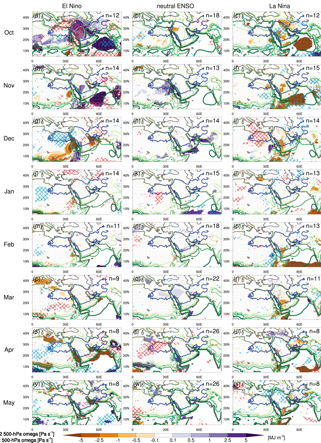
Figure A5. As Fig. 9 but for individual months from October to May in rows and the ENSO phases – warm, neutral, and cold – in columns. The ENSO phases are defined based on 3-monthly running mean SST anomalies in the Niño3.4 region. Sample sizes are indicated in text in the top right corner of each panel.
