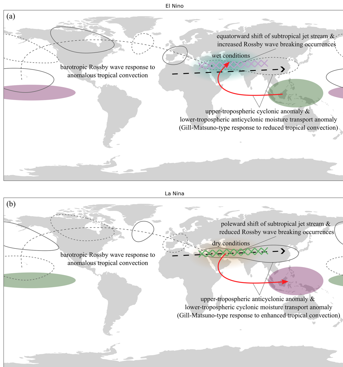
Figure 13. A schematic representation of three different mechanisms through which ENSO modulates Middle Eastern precipitation variability during the cool season under (a) El Niño and (b) La Niña conditions: (1) a zonally symmetric displacement of the subtropical jet (cf. Kumar et al., 2016; Alizadeh-Choobari et al., 2018; Sandeep and Ajayamohan, 2018; Hoell et al., 2024) alongside modifications in Rossby wave breaking occurrences on the poleward flank and beneath the jet core, (2) a barotropic Rossby wave response arching from the tropical Pacific via the extratropics toward the Middle East (cf. Kumar et al., 2016; Hoell et al., 2013, 2015a; Abid et al., 2020), and (3) a regional baroclinic response in the tropical circulation extending westwards from the tropical Warm Pool, consistent with a Gill-Matsuno-type response (cf. Barlow et al., 2002; Hoell et al., 2012, 2015a). This schematic is inspired by Fig. 9 from Barlow et al. (2016), showing mechanism (2) and (3) for La Niña conditions.
