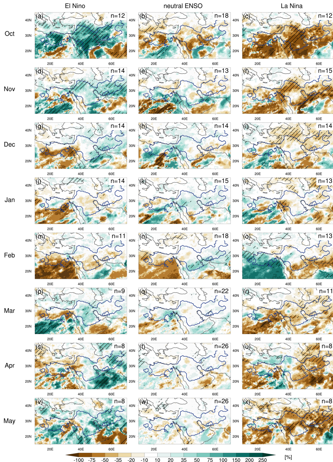
Figure A1. As Fig. 2a, b, c but for individual months from October to May. The ENSO phases are defined based on 3-monthly running mean SST anomalies in the Nino3.4 region. Sample sizes are indicated in text in the top right corner of each panel.
