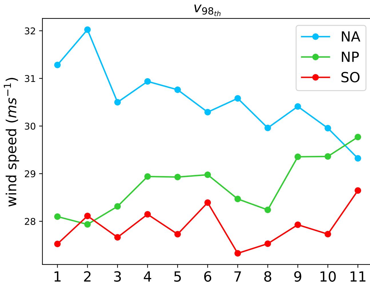
Figure S4. Winter basin-wide 98th percentiles of near-surface wind speed (y-axis) across 11 different ISCA experiment runs used to produce scatterplot in Fig. 7. Numbers on x-axis correspond to the experiments named in Table S1. Among other things, a consideration of the experiments that are not further analyzed in Fig. 8 shows strong nonlinear response to the flattening of orography. For example, flattening orography while SSTs keep the climatological distribution (experiment 2) does not reduce the asymmetry between the North Atlantic and the Southern Ocean. Moreover, the winter basin-wide 98th percentiles in the North Atlantic and North Pacific have the opposite response to flat orography when SSTs have climatological distribution (experiment 2) compared to the case when SSTs are zonalized (experiment 11 - HemSymFlat). It could also be interesting to point out that, once the SSTs are zonalized across midlatitudes (experiment 3), the 98th percentile in the North Atlantic is not heavily influenced by the presence of orography on Greenland (experiment 7) or the existence of Greenland (experiment 8) in ISCA model.
