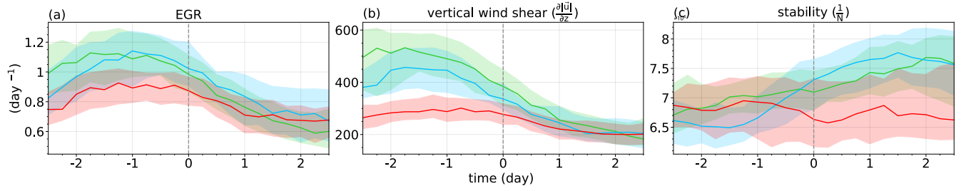
Figure S1. Time-evolution of median values in the 1000-km footprint around top 100 extremes of mid-tropospheric Eady growth rate (a), and contributions to it from the vertical wind shear (b) and stability terms (c). Shading in (a-c) shows the area between 25th and 75th percentiles.
