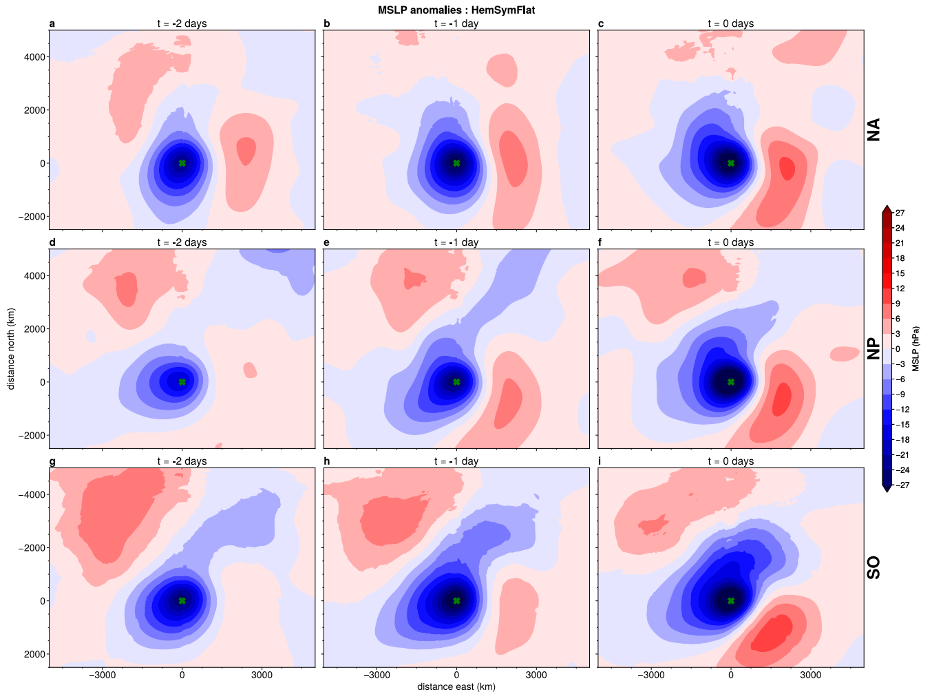
Figure S7. Composite MSLP anomalies in ISCA's HemSymFlat experiment relative to the winter climatology for top 100 extremes in the NA (a-c), NP (d-f) and SO (g-i) centered on the cyclone locations from t = -2 days to t = 0 days. Lags are relative to the time of maximum 10-m wind speeds on the day with maximum severity. Green crosses denote locations of cyclone centers of top 100 extremes.
