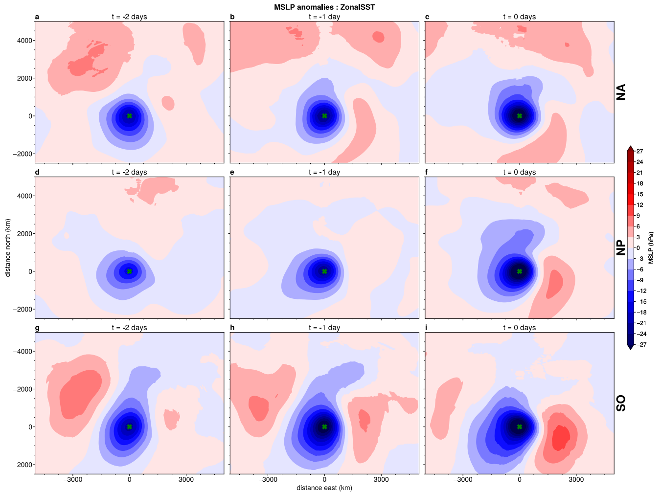
Figure S6. Composite MSLP anomalies in ISCA's ZonalSST experiment relative to the winter climatology for top 100 extremes in the NA (a-c), NP (d-f) and SO (g-i) centered on the cyclone locations from t = -2 days to t = 0 days. Lags are relative to the time of maximum 10-m wind speeds on the day with maximum severity. Green crosses denote locations of cyclone centers of top 100 extremes.
