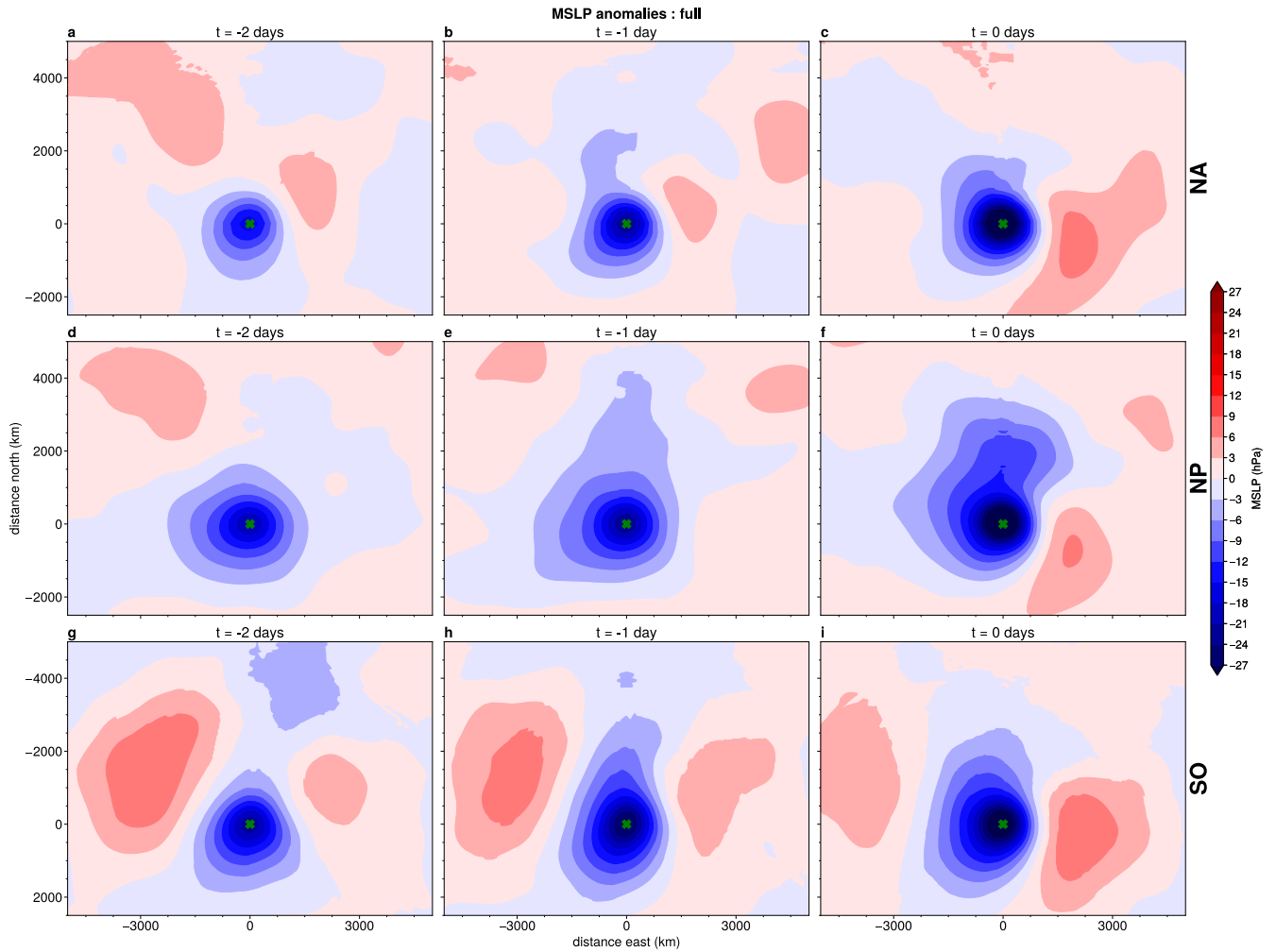
Figure S5. Composite MSLP anomalies in ISCA's Full experiment relative to the winter climatology for top 100 extremes in the NA (a-c), NP (d-f) and SO (g-i) centered on the cyclone locations from t = -2 days to t = 0 days. Lags are relative to the time of maximum 10-m wind speeds on the day with maximum severity. Green crosses denote locations of cyclone centers of top 100 extremes.
