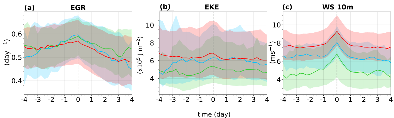
Figure S2. Time-evolution of median values of mid-tropospheric Eady growth rate (a), vertically integrated eddy kinetic energy (b) and 10-w wind speed (c) in the 1000-km footprint around winter cyclones where the maximum EGR during their life-cycle is restricted to be 30 % lower than that of top 100 extremes. Shading in (a-c) shows the area between 25th and 75th percentiles.
