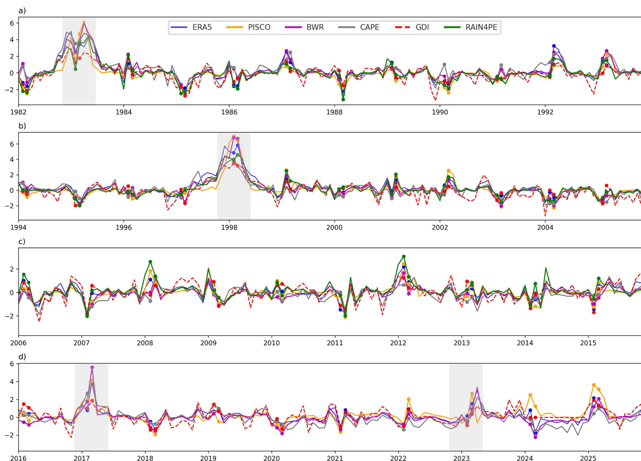
Figure 6. Time series of monthly standardized anomalies of convective indices, such as CAPE (gray), BWR (magenta), and GDI (dashed red), and standardized precipitation from ERA5 (blue), PISCO (orange), and RAIN4PE (green). All data are spatially averaged over the coastal subdomain (Fig. 2b) for the period 1981–2025. The RAIN4PE dataset is only available for 1981–2015. Anomalies were calculated taking the 1981–2015 median as climatology. Circle markers indicate February and March of every year. The vertical gray shadings show the four most extreme events: 1983, 1998, 2017 and 2023.
