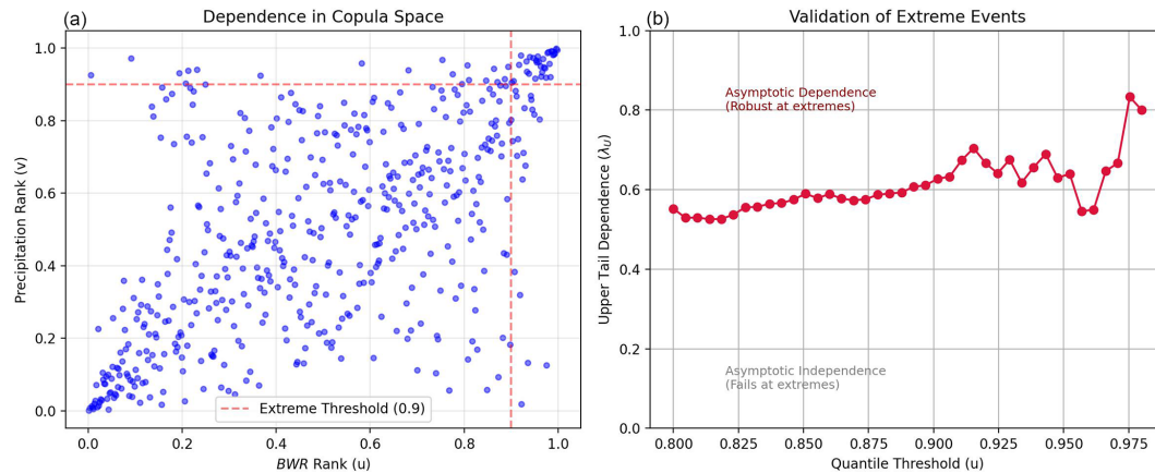
Figure 13. Analysis of the extreme dependence structure between BWR index and precipitation anomalies in the NWSA adjacent to Niño 1 + 2. (a) Scatterplot of pseudo-observations (uniform ranks) in the empirical copula space. The dashed red lines indicate the 0.90 quantile threshold; points in the upper-right quadrant represent concurrent extreme events. (b) The empirical Upper Tail Dependence Coefficient ( \lambda_U ) as a function of the quantile threshold ( u ).
