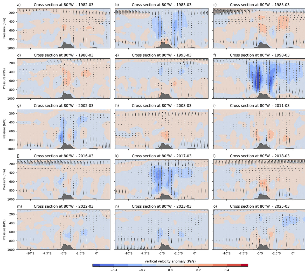
Figure 9. Latitudinal cross-section of the resultant vector between the anomalies of \omega and meridional wind at 80^\circ\text{W} , spanning from 12^\circ\text{S} to 2^\circ\text{N} , for the extreme hydroclimatic anomalies identified in Sect. 4. The blue (red) shaded colors indicate negative (positive) values of \omega . The \omega vector was multiplied by -20 to increase its scale and to get upward (downward) arrows with the air ascent (descent). Anomalies were calculated taking the 1981–2025 median as climatology.
