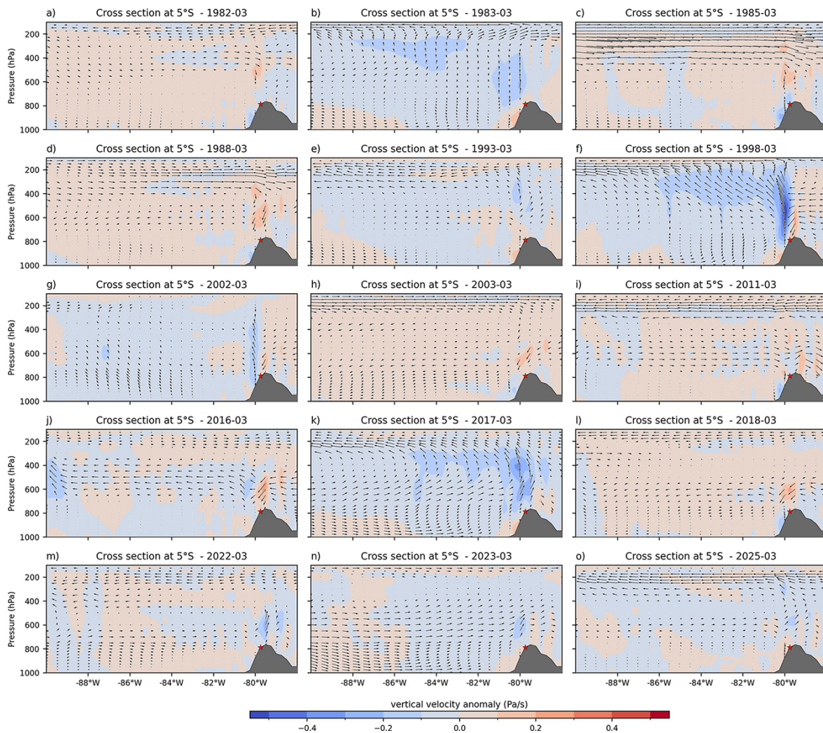
Figure 10. Longitudinal cross-section of the resultant vector between the anomalies of \omega and zonal wind at 5^{\circ}\text{S} , spanning from 90 to 78^{\circ}\text{W} , for the extreme hydroclimatic anomalies identified in Sect. 4. The blue (red) shaded colors indicate negative (positive) values of \omega . The \omega vector was multiplied by -20 to increase its scale and to get upward (downward) arrows with the air ascent (descent). Anomalies were calculated taking the 1981–2025 median as climatology. Red star represents the longitude of the boundary between the ascent core and the descent core of the 1998 event.
