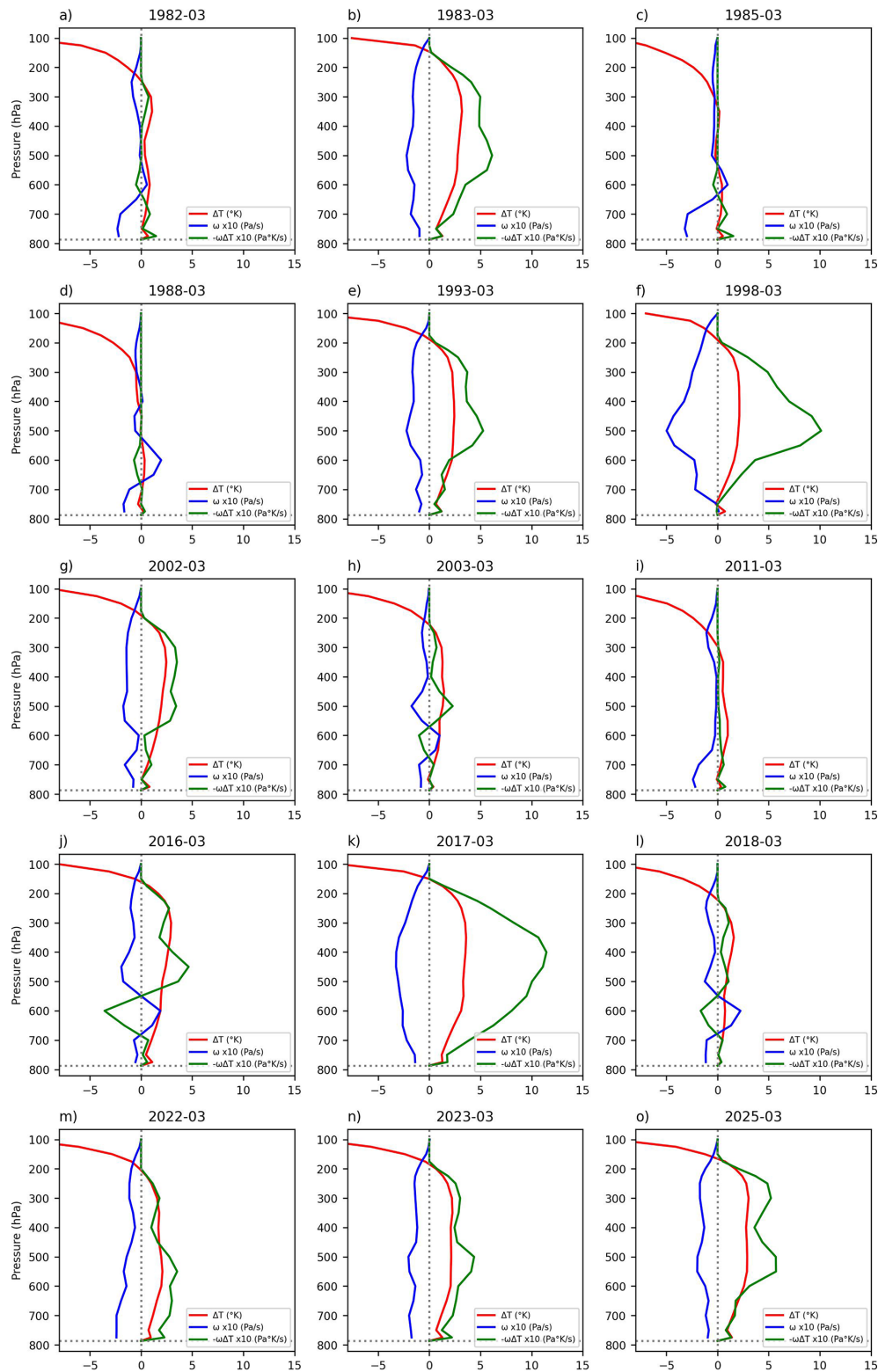
Figure 11. Profiles of \Delta T (red), \omega (blue) and -\omega\Delta T (green) at (79.75°W, 5°S) for the extreme hydroclimatic anomalies identified in Sect. 4. The \omega was multiplied by 10 to increase its scale. The horizontal dotted line shows the equivalent altitude of that point in pressure units. All variables share the same horizontal numerical axis.
