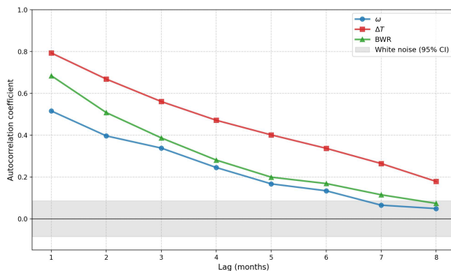
Figure 14. Analysis of signal persistence for the physical components of the BWR index. The plot displays the autocorrelation function (ACF) for vertical velocity ( \omega , blue), parcel buoyancy 400–700 hPa average ( \Delta T , red), and the BWR index (green) up to a lag of 8 months. The gray shaded area indicates the 95% confidence interval for a white noise process ( \pm 1.96/\sqrt{N} ).
