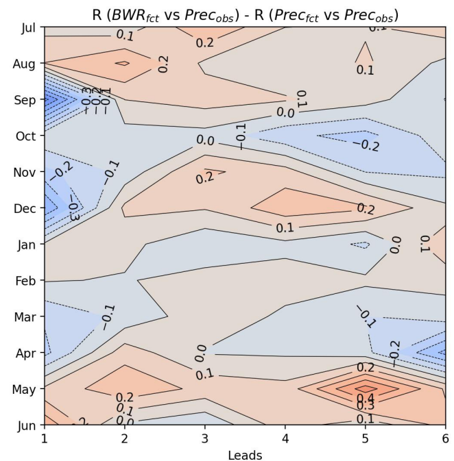
Figure 15. Predictive skill of BWR anomalies predicted up to a lead of 6 months. Shaded colors in red (blue) and contours with \Delta R > 0 ( \Delta R < 0 ) represent better (worse) BWR predictive skill compared to the precipitation anomalies predicted by the SEAS5 model for the 2017–2025 operational period, using the PISCO dataset as the observational reference. The Y-axis represents the initial condition of the prediction.
