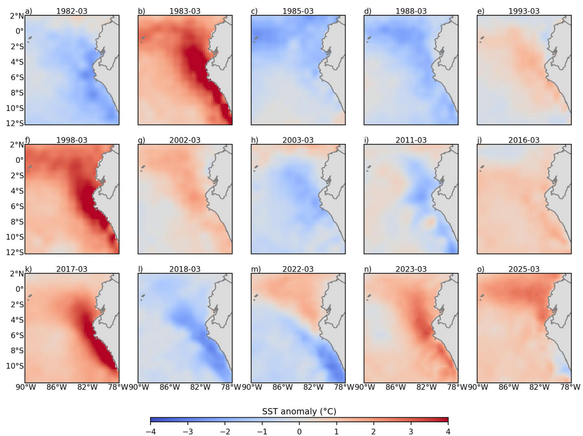
Figure A2. SST anomaly over the Niño 1 + 2 region from ERA5 for the extreme hydroclimatic events identified in Sect. 4. The blue (red) shaded colors indicate negative (positive) anomalies of SST. Taking the 1981–2025 median as climatology.
