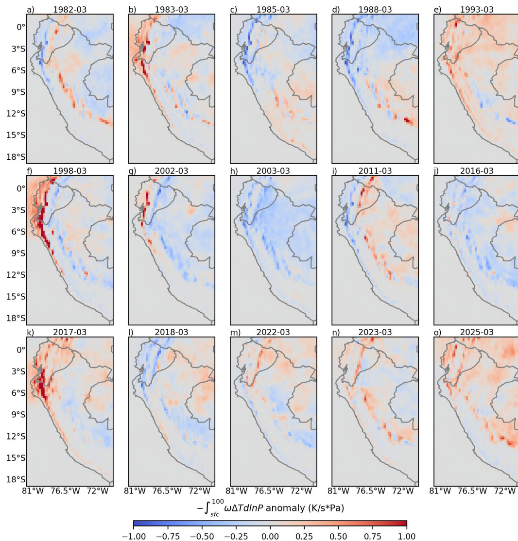
Figure 12. BWR anomaly, taking the 1981–2025 median as climatology, for the extreme hydroclimatic events identified in Sect. 4. The blue (red) shaded colors indicate negative (positive) anomalies of BWR.
