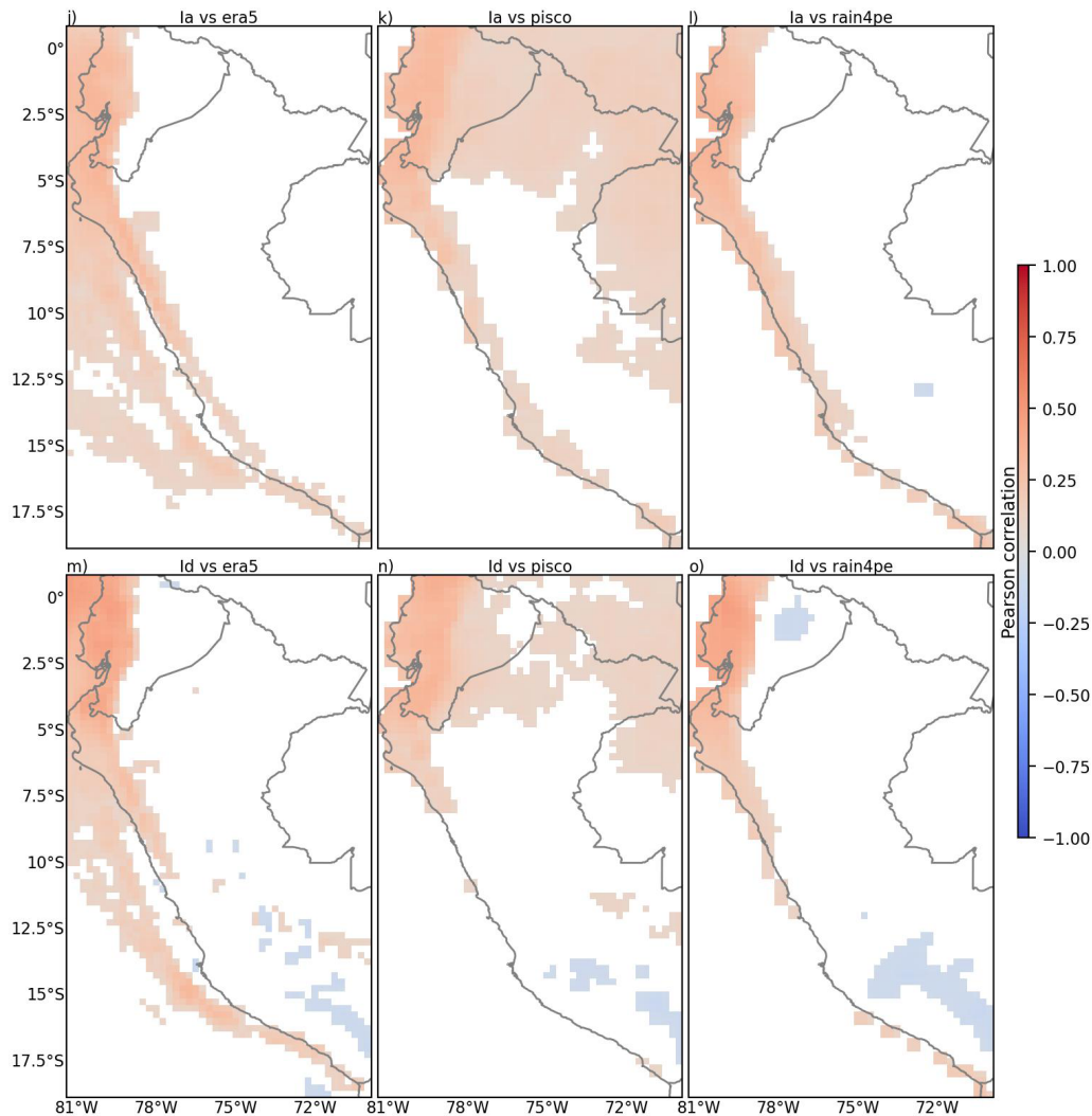
Figure 4. Pearson correlation ( R ) maps at the 95 % confidence level between monthly anomalies of convective indices (rows) and precipitation datasets (columns) for the 1981–2015 common period. The indices (rows) are (a–c) CAPE, (d–f) BWR, (g–i) GDI, (h–l) Ia, and (m–o) Id. The precipitation datasets (columns) are (a, d, g) ERA5, (b, e, h) PISCO, and (c, f, i) RAIN4PE. Shading is shown only for significant correlations ( p -value < 0.05). Red (blue) indicates positive (negative) R values. Gray points highlight strong correlations ( R > 0.7 ). Anomalies were calculated taking the 1981–2015 median as climatology.
