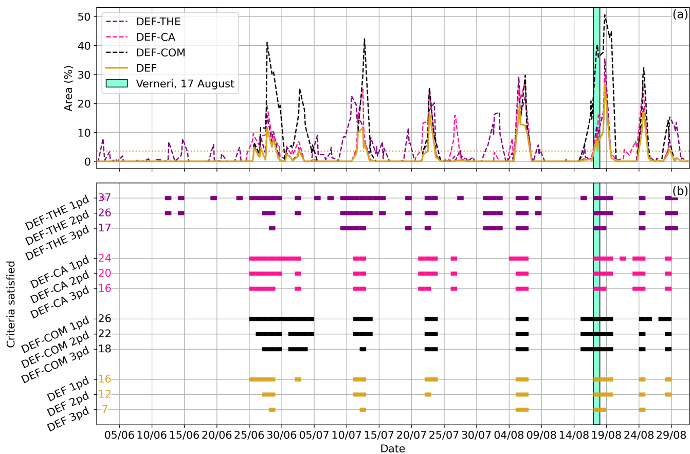
Figure S17. Same as Fig. S14 but for summer 2022.
