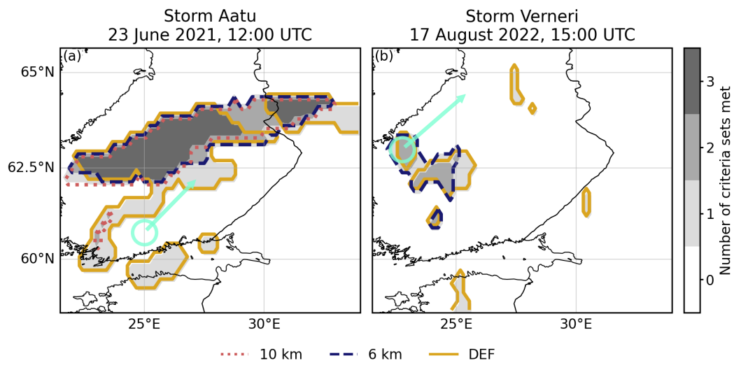
Figure S9. Same as Fig. S8 but for storms Aatu (a) and Verner (b).
