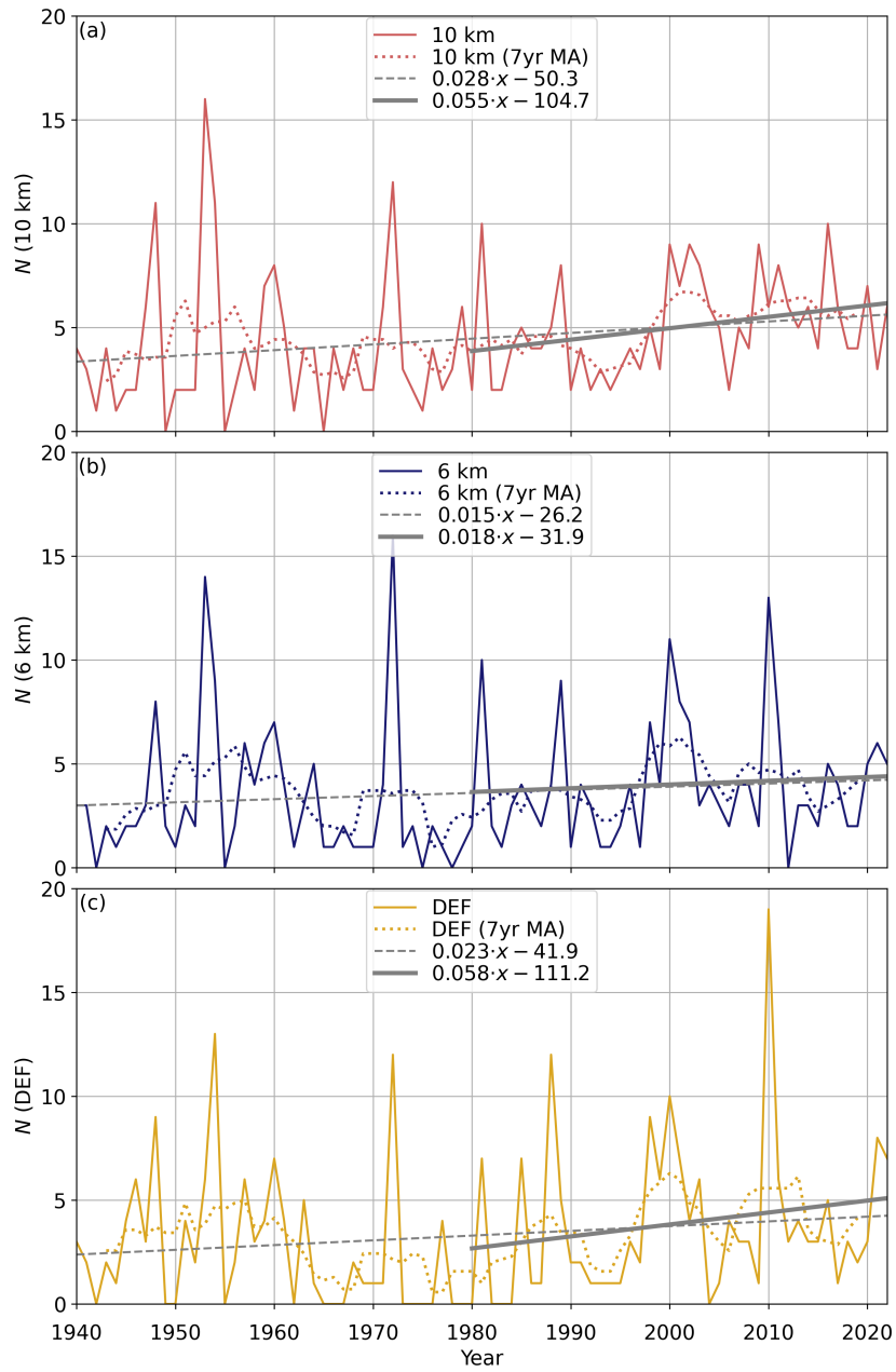
Figure S19. Same as Fig. S18 but with conditions satisfied at all three analyzed times (3pd).
