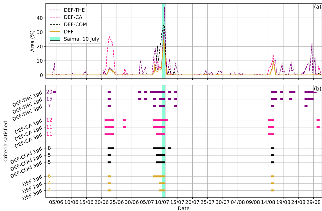
Figure S15. Same as Fig. S14 but for summer 2006.
