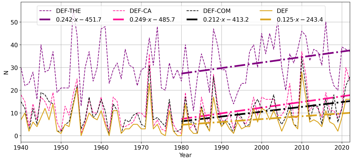
Figure S20. Same as Fig. 8 in the main article but with conditions satisfied at least once per day (1pd): the figure is similar to Fig. S21, but for the same criteria combinations within the DEF criteria as in Fig. S17. The corresponding linear regression lines for the 1980–2022 period are drawn with dash-dotted lines.
