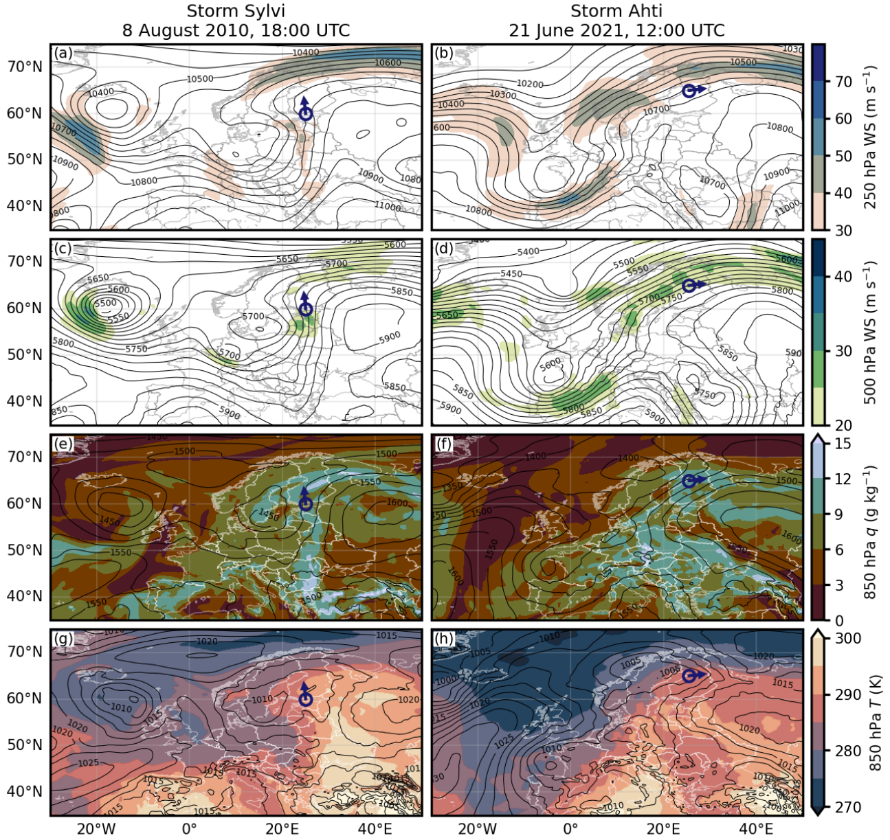
Figure S2. Same as Fig. S1 but only for two storms: Sylvi (panels a, c, e and g) and Ahti (panels b, d, f and h). Panels (a-b) show 250 hPa jet stream (shade) and geopotential (contours), (c-d) 500 hPa jet stream (shade) and geopotential (contours), (e-f) 850 hPa specific humidity (shade) and geopotential (contours), and (g-h) 850 hPa temperature (shade) and MSLP (contours)
