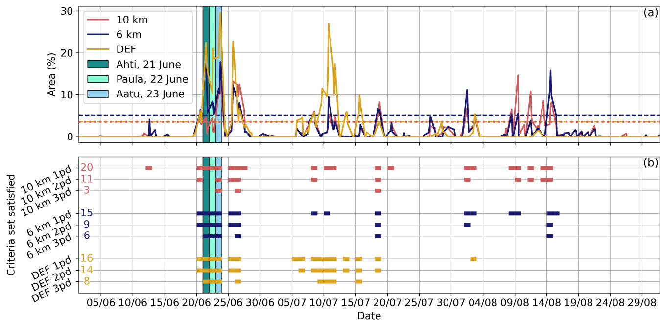
Figure S12. Same as Fig. S10 but for summer 2021.
