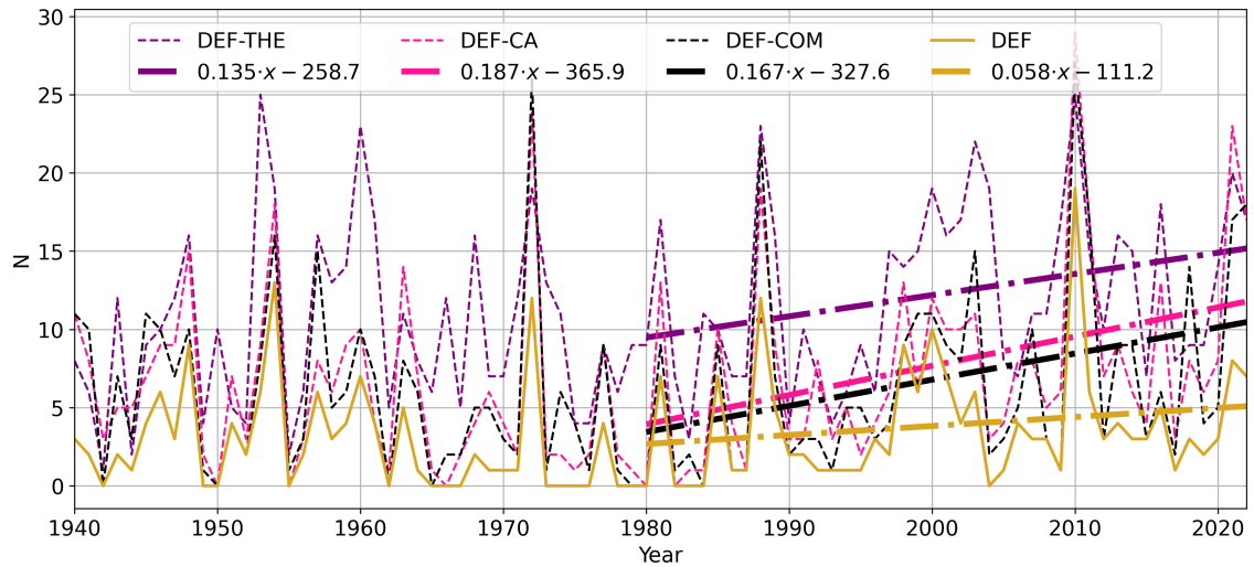
Figure S21. Same as Fig. S20 but with conditions satisfied at all three analyzed times (3pd).
