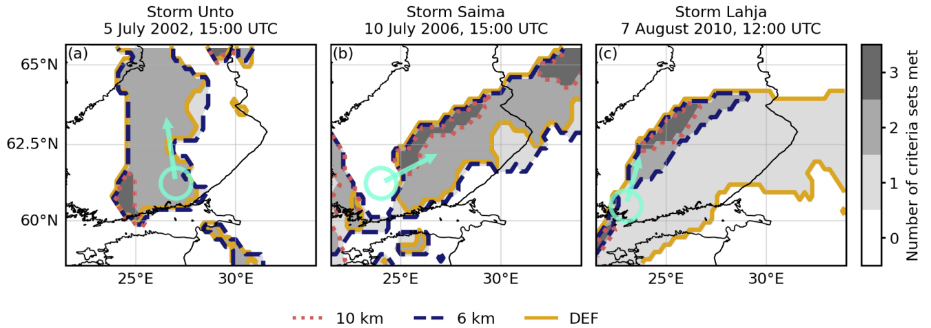
Figure S7. Same as Fig. 4 in the main article but for storms Unto (a), Saima (b) and Lahja (c): shades of gray indicate how many of the three criteria sets are met in each grid cell. The areas satisfying the 10 km criteria set are outlined with red dotted lines, the 6 km criteria set with blue dashed lines and the DEF criteria set with gold solid lines. Aquamarine circles indicate the approximate location of the systems at the times of the analyses and arrows point to the approximate movement of the system during the following three hours.
