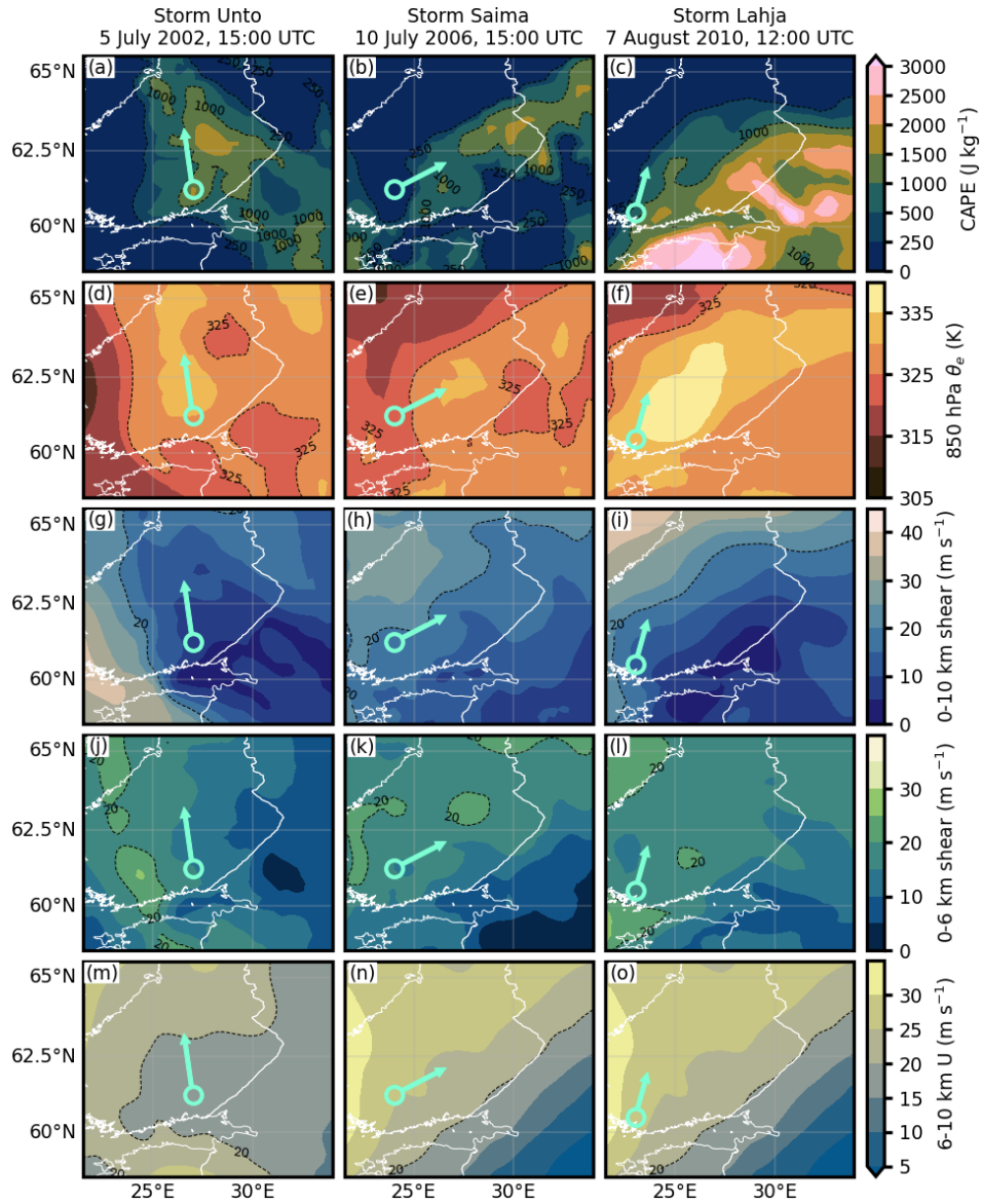
Figure S4. Same as Fig. 3 in the main article but for storms Unto (panels a, d, g, j and m), Saima (panels b, e, h, k and n) and Lahja (panels c, f, i, l and o): panels (a-c) show CAPE (shading, isolines of 250 \text{ J kg}^{-1} and 1000 \text{ J kg}^{-1} are also drawn with black dashed contours to help readability), (d-f) equivalent potential temperature ( \theta_E ) at 850 hPa (shading, 325 \text{ K} isolines drawn with dashed black contours), (g-i) 0–10 km vertical wind shear (shading, 20 \text{ m s}^{-1} isolines drawn with dashed black contours), (j-l) 0–6 km vertical wind shear (shading, 20 \text{ m s}^{-1} isolines drawn with dashed black contours) and (m-o) 6–10 km layer mean wind speed (shading, 20 \text{ m s}^{-1} isotachs drawn with dashed black contours). In all panels, aquamarine circles indicate the approximate location of the systems at the times of the analyses and arrows point to the approximate movement of the system during the following three hours.
