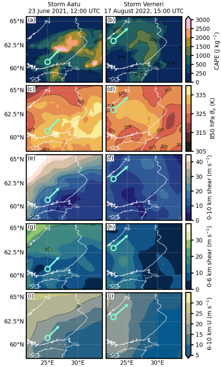
Figure S6. Same as Fig. S5 but for storms Aatu (panels a, c, e, g and i) and Verner (panels b, d, f, h and j).
