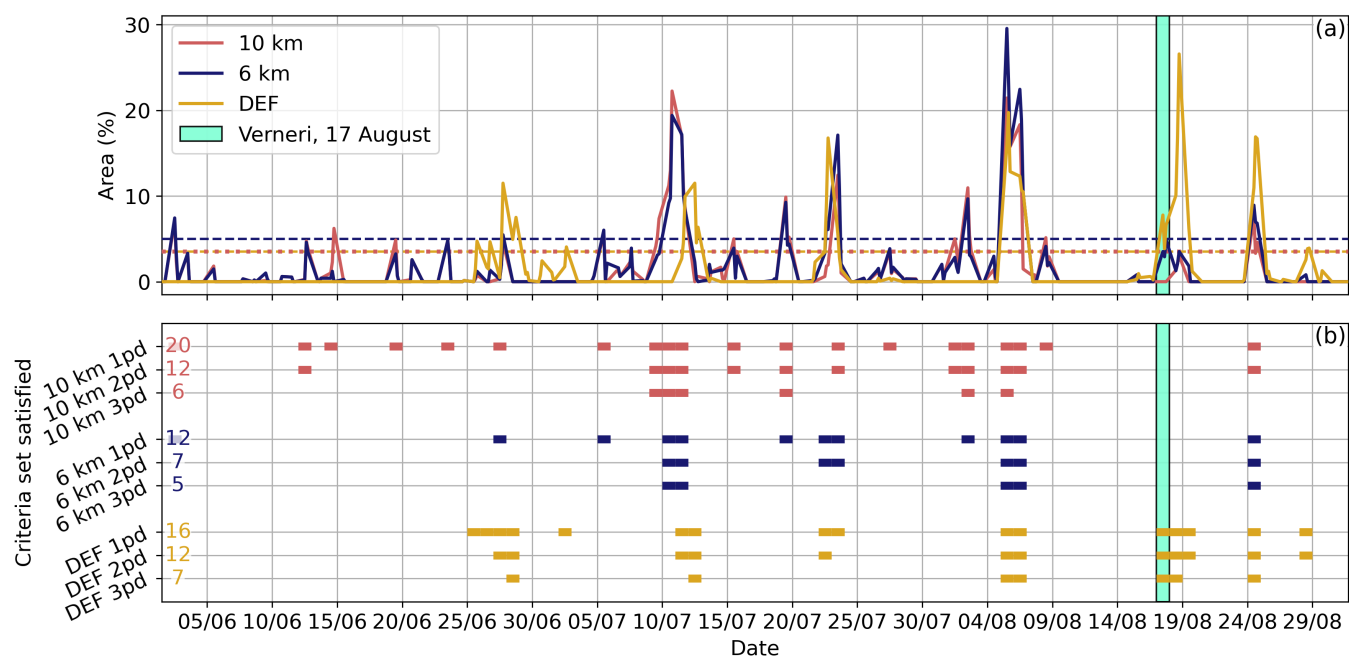
Figure S13. Same as Fig. S10 but for summer 2022.
