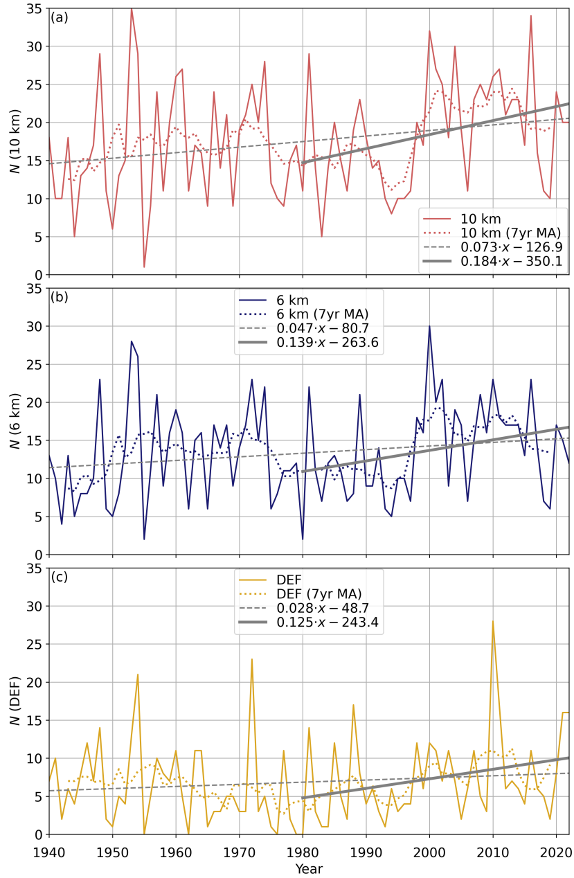
Figure S18. Same as Fig. 7 in the main article for the number of favorable days ( N ) per year but with conditions satisfied at least once per day (1pd), obtained with the 10 km criteria set (a, solid red line), 6 km criteria set (b, solid blue line) and DEF criteria set (c, solid gold line). Linear regressions are fitted to each panel for both the 1940–2022 time range (gray dashed lines) and 1980–2022 time range (solid gray lines). The dotted lines represent 7-year moving averages (7yr MA).
