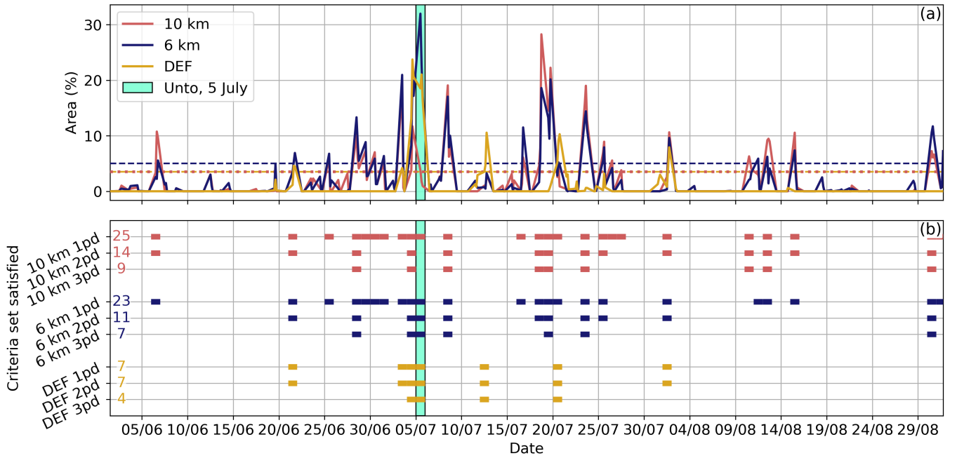
Figure S10. Same as Fig. 5 in the main article but for summer 2002: vertical bar(s) in both panels indicate day(s) when derechos occurred. Panel (a) shows the fraction (%) of the grid area where each criteria set is satisfied. The red line represents the 10 km criteria set, the blue line the 6 km criteria set and the gold line the DEF criteria set. Data includes three time steps per day (12, 15, and 18 UTC), as described in the main article in Sect. 2.4. Horizontal lines illustrate the area demands for each criteria set: 5 % for the 6 km criteria set (blue, dashed) and 3.5% for both the 10 km (red, dashed) and DEF criteria sets (gold, dotted). Panel (b) presents the favorable days throughout the summer for each criteria set, with conditions satisfied once per day (1pd), twice per day (2pd) and at all three times per day (3pd), illustrated with bold lines. Total number of favorable days for each category is indicated on the left side of the panel.
