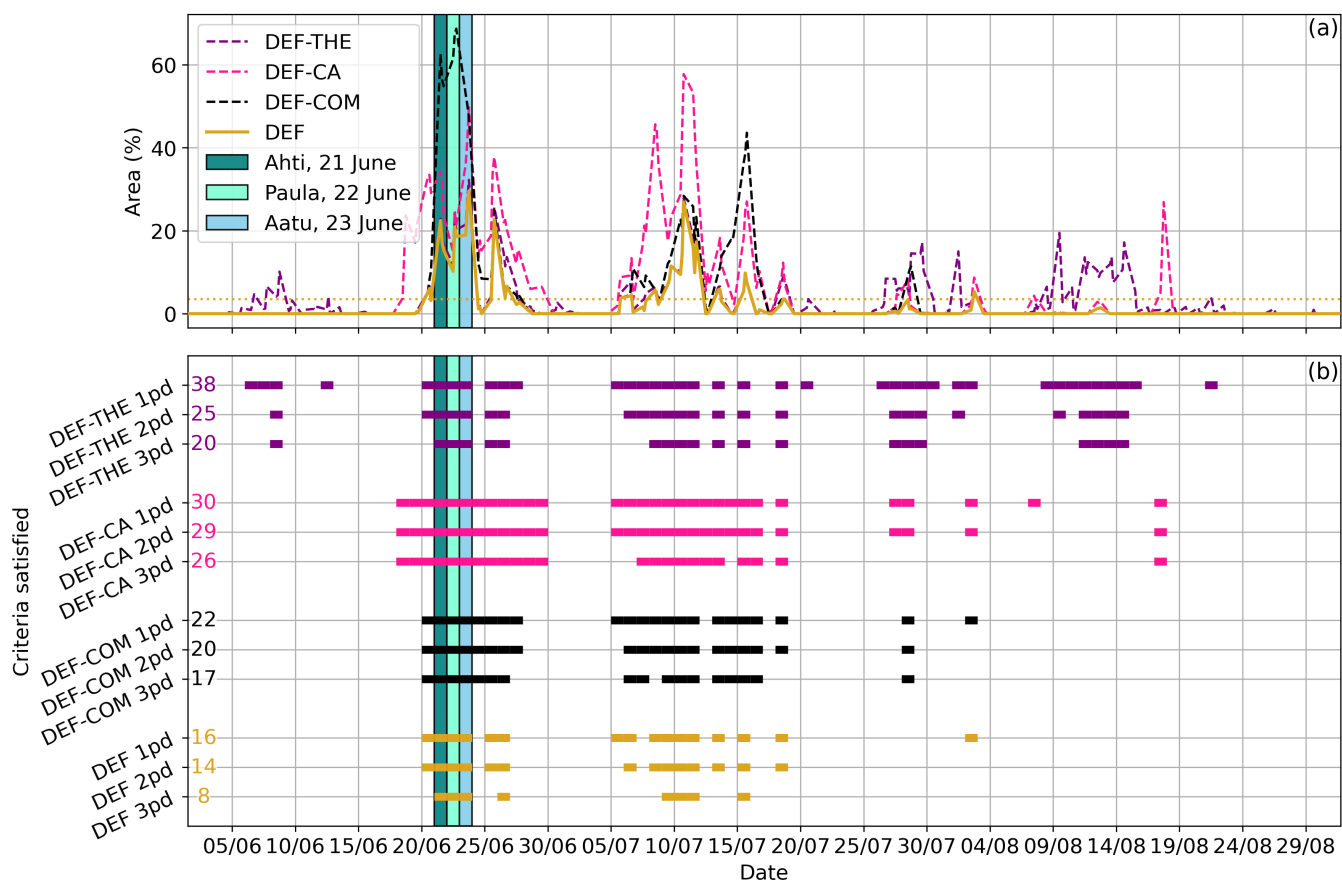
Figure S16. Same as Fig. S14 but for summer 2021.
