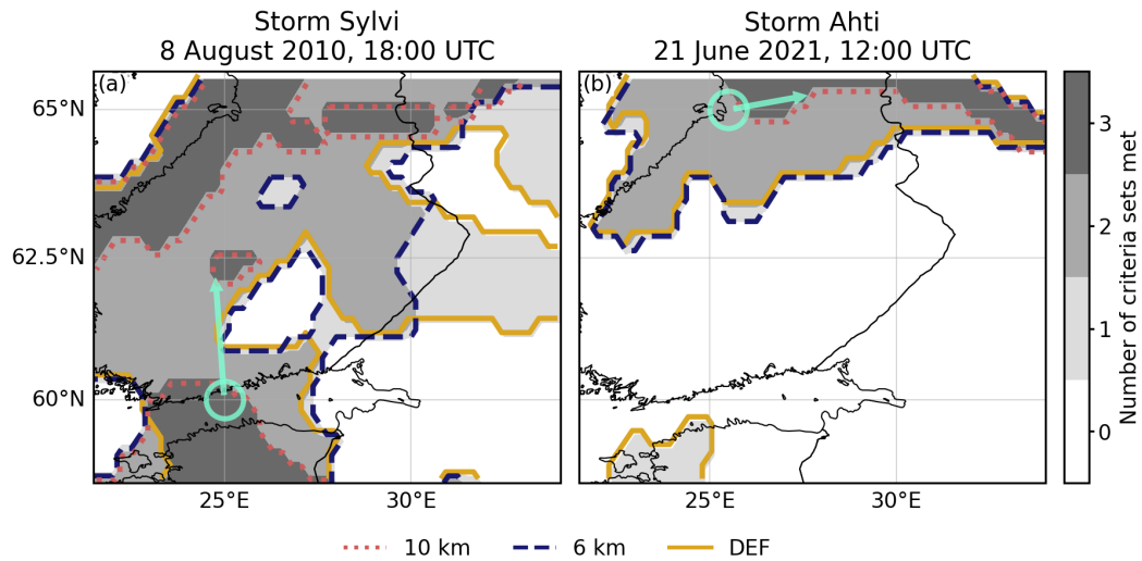
Figure S8. Same as Fig. S7 but only for two storms: Sylvi (a) and Ahti (b).
