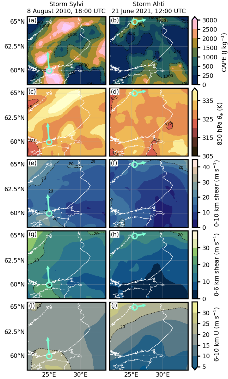
Figure S5. Same as Fig. S4 but only for two storms: Sylvi (panels a, c, e, g and i) and Ahti (panels b, d, f, h and j). Panels (a–b) show CAPE, (c–d) 850 hPa \theta_e , (e–f) 0–10 km shear, (g–h) 0–6 km shear, and (i–j) 6–10 km mean wind speed.
