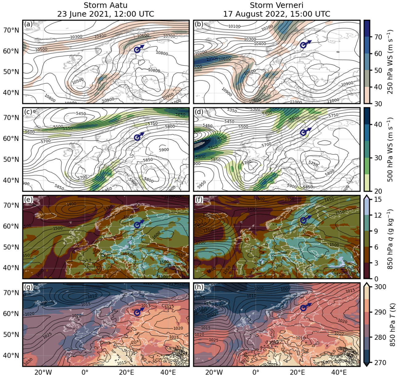
Figure S3. Same as Fig. S2 but for storms Aatu (panels a, c, e and g) and Verner (panels b, d, f and h).
