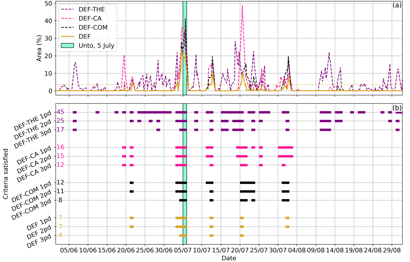
Figure S14. Same as Fig. 6 in the main article but for summer 2002: As in Fig. S13 but for combinations of criteria within the DEF criteria set, with the dashed lines representing the DEF criteria set excluding the 850 hPa \theta_E \geq 325 K condition (DEF-THE, purple), CAPE \geq 250 J \text{kg}^{-1} condition (DEF-CA, pink) and combined shear condition (DEF-COM, black). The gold solid line shows the full DEF criteria set (DEF) as a reference.
