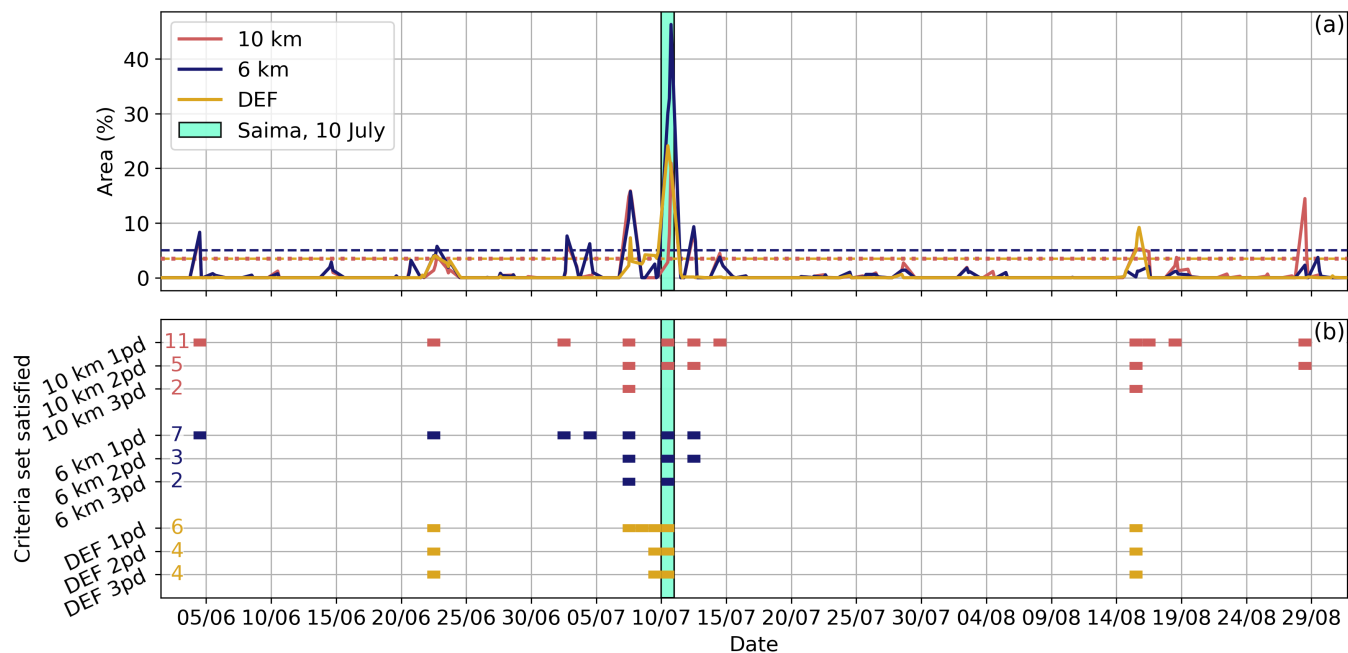
Figure S11. Same as Fig. S10 but for summer 2006.
