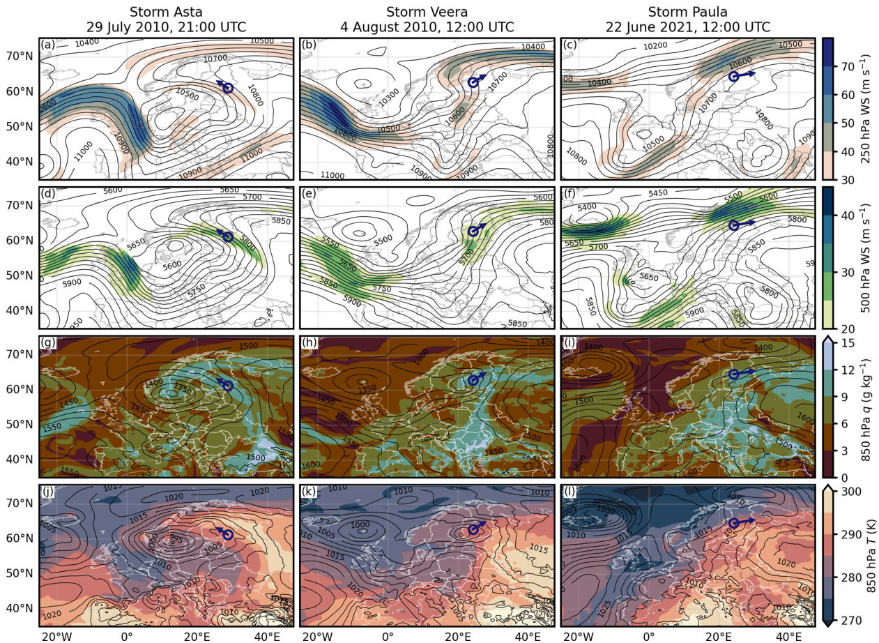
Figure 2. Synoptic-scale pattern during the storms Asta (29 July 2010 at 21:00 UTC) in the left column (a, d, g, j), Veera (4 August 2010 at 12:00 UTC) in the center column (b, e, h, k) and Paula (22 June 2021 at 12:00 UTC) in the right column (c, f, i, l). Panels (a)–(c) show wind speed (WS, shading starting from 30 \text{ m s}^{-1} ) and geopotential height at 250 hPa, (d–f) wind speed (WS, shading starting from 20 \text{ m s}^{-1} ) and geopotential height at 500 hPa, (g–i) specific humidity ( q , shading) and geopotential height (black contours) at 850 hPa, and (j–l) temperature ( T ) at 850 hPa (shading) and mean sea level pressure (MSLP, black contours). In all panels, blue circles indicate the approximate location of the systems at the times of the analyses and arrows point to the approximate movement of the system during the following 3 h.
