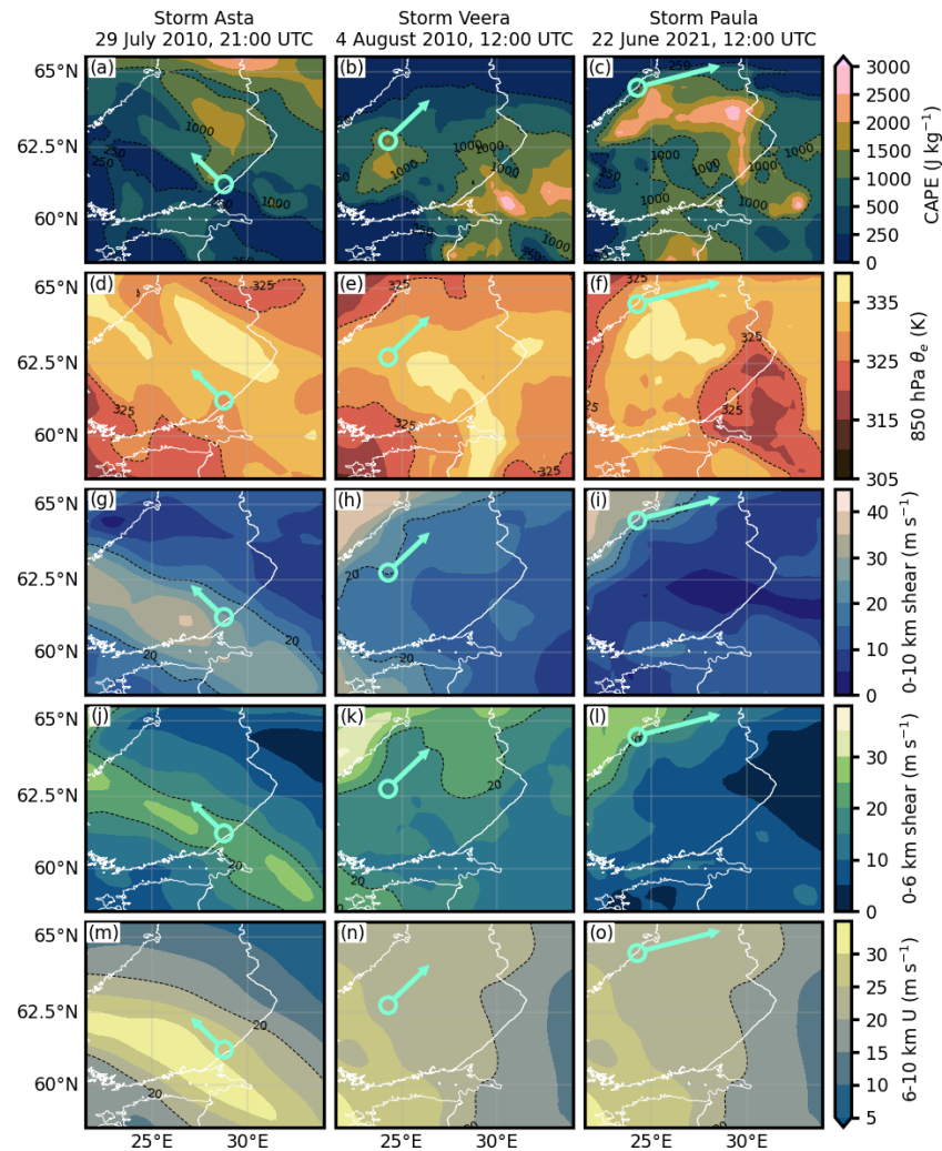
Figure 3. Atmospheric conditions in southern and central Finland during the storms Asta (29 July 2010 at 21:00 UTC) in the left column (a, d, g, j, m), Veera (4 August 2010 at 12:00 UTC) in the center column (b, e, h, k, n) and Paula (22 June 2021 at 12:00 UTC) in the right column (c, f, i, l, o). Panels (a)–(c) show CAPE (shading, isolines of 250 and 1000 J kg −1 are also drawn with black dashed contours to help readability), (d)–(f) equivalent potential temperature ( \theta_E ) at 850 hPa (shading, 325 K isolines drawn with dashed black contours), (g)–(i) 0–10 km vertical wind shear (shading, 20 m s −1 isolines drawn with dashed black contours), (j)–(l) 0–6 km vertical wind shear (shading, 20 m s −1 isolines drawn with dashed black contours) and (m)–(o) 6–10 km layer mean wind speed (shading, 20 m s −1 isotachs drawn with dashed black contours). In all panels, aquamarine circles indicate the approximate location of the systems at the times of the analyses and arrows point to the approximate movement of the system during the following 3 h.
