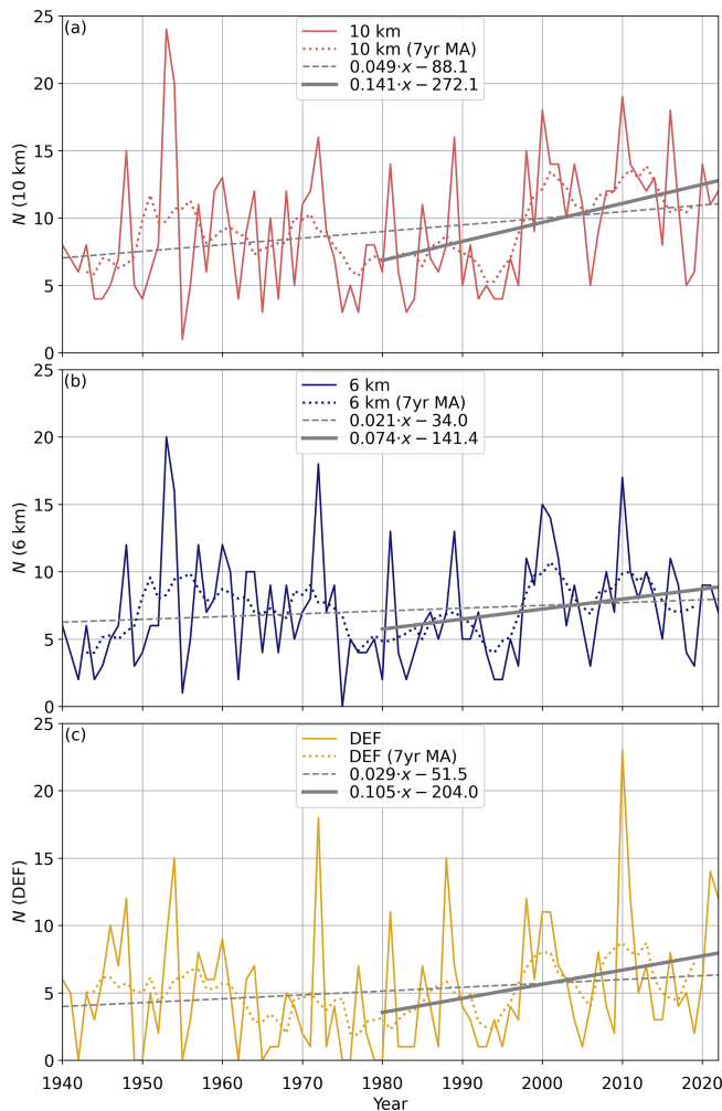
Figure 7. Number of favorable days ( N ) per year, with conditions satisfied at least twice per day (2pd), obtained with the 10 km criteria set (a, solid red line), 6 km criteria set (b, solid blue line) and DEF criteria set (c, solid gold line). Linear regressions are fitted to each panel for both the 1940–2022 time range (dashed gray lines) and 1980–2022 time range (solid gray lines). The dotted lines represent 7-year moving averages (7yr MA).
