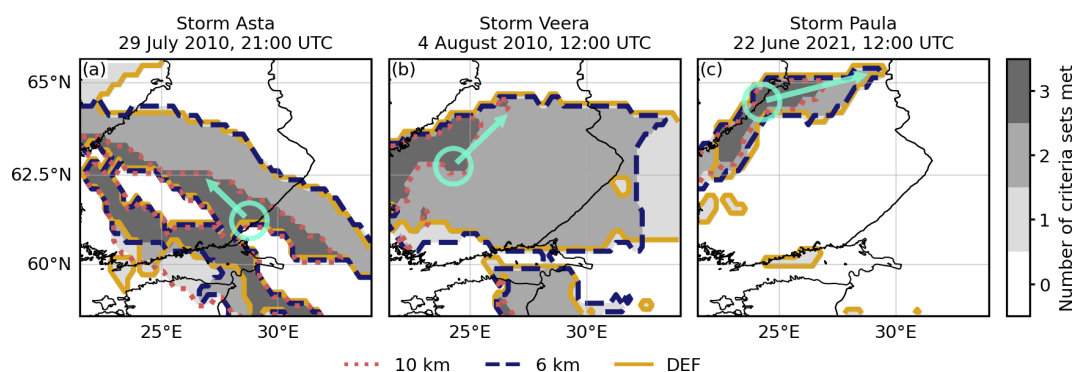
Figure 4. Areas satisfying each criteria set during the storms Asta (29 July 2010 at 21:00 UTC) in panel (a), Veera (4 August 2010 at 12:00 UTC) in panel (b) and Paula (22 June 2021 at 12:00 UTC) in panel (c). Shades of gray indicate how many of the three criteria sets are met in each grid cell. The areas satisfying the 10 km criteria set are outlined with red dotted lines, the 6 km criteria set with blue dashed lines and the DEF criteria set with gold solid lines. Aquamarine circles indicate the approximate location of the systems at the times of the analyses and arrows point to the approximate movement of the system during the following 3 h.
