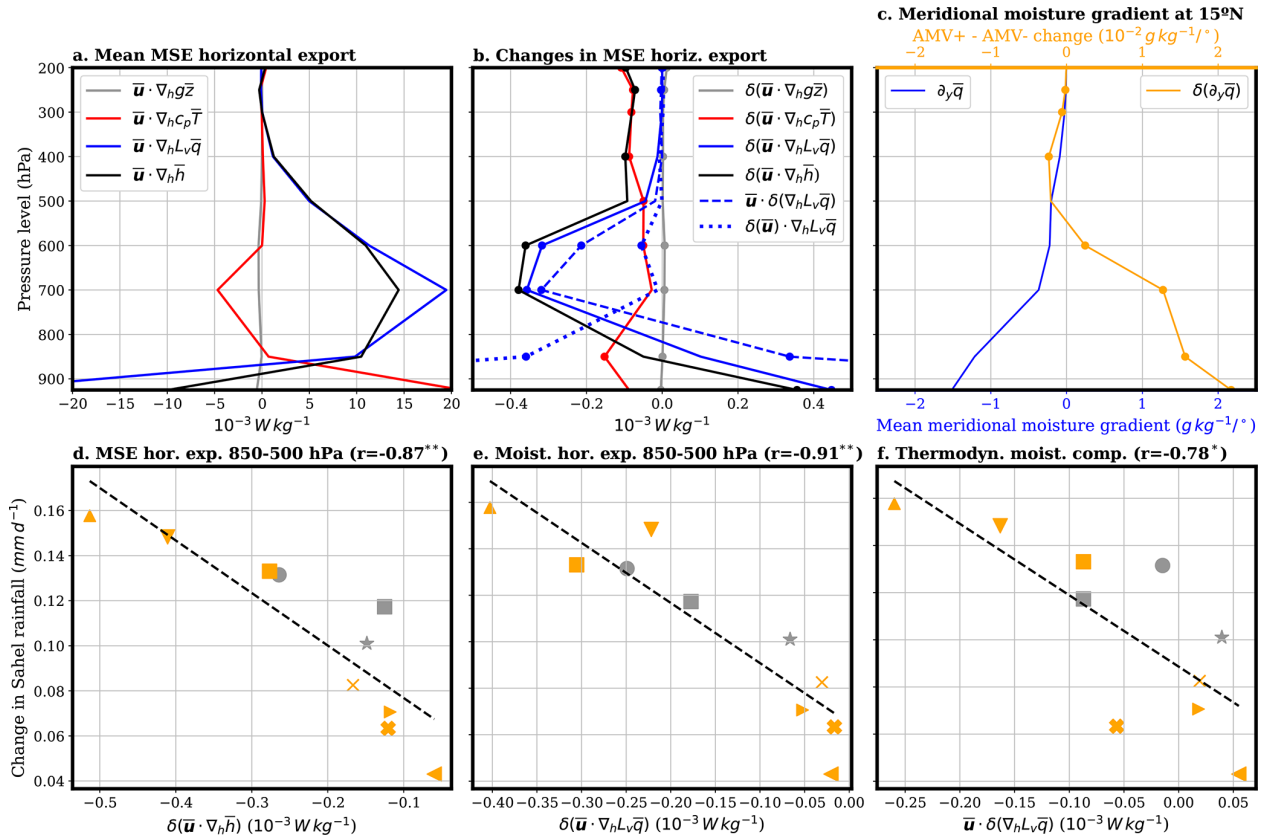
Figure 7. (a) Climatological export of MSE by the time-mean horizontal flow ( \bar{\mathbf{u}} \cdot \nabla_h \bar{h} , black line) partitioned into the potential energy ( \bar{\mathbf{u}} \cdot \nabla_h g \bar{z} , grey line), sensible ( \bar{\mathbf{u}} \cdot \nabla_h c_p \bar{T} , red line), and latent enthalpy ( \bar{\mathbf{u}} \cdot \nabla_h L_v \bar{q} , blue line) components averaged over the Sahel box ( 10^\circ \text{W} – 10^\circ \text{E} , 10^\circ – 20^\circ \text{N} ) for the multimodel mean. (b) \text{AMV}^+ minus \text{AMV}^- multimodel change in the export of MSE by the time-mean horizontal flow ( \delta(\bar{\mathbf{u}} \cdot \nabla_h \bar{h}) , black) partitioned into the potential energy ( \delta(\bar{\mathbf{u}} \cdot \nabla_h g \bar{z}) , grey), sensible ( \delta(\bar{\mathbf{u}} \cdot \nabla_h c_p \bar{T}) , red), and latent enthalpy ( \delta(\bar{\mathbf{u}} \cdot \nabla_h L_v \bar{q}) , blue) averaged over the Sahel box. The change in latent enthalpy has been further decomposed into its thermodynamic ( \bar{\mathbf{u}} \cdot \delta(\nabla_h L_v \bar{q}) , blue dashed) and dynamic ( \delta(\bar{\mathbf{u}}) \cdot \nabla_h L_v \bar{q} , blue dotted) components. (c) Multimodel mean meridional gradient of the 10^\circ \text{W} – 10^\circ \text{E} zonally averaged specific humidity ( \text{g kg}^{-1} per degree) at 15^\circ \text{N} ( \partial_y \bar{q} , blue) and \text{AMV}^+ minus \text{AMV}^- changes ( \delta(\partial_y \bar{q}) , orange). Scatter plots of averaged Sahel rainfall change ( \text{mm d}^{-1} ) and averages of changes over the Sahel box between 850 hPa and the 500 hPa levels of: (d) total export of MSE due to time-mean horizontal flow ( \delta(\bar{\mathbf{u}} \cdot \nabla_h \bar{h}) ); (e) MSE export due to horizontal moisture advection in MSE units ( \delta(\bar{\mathbf{u}} \cdot \nabla_h L_v \bar{q}) ); and (f) its thermodynamic component also in MSE units ( \bar{\mathbf{u}} \cdot \delta(\nabla_h L_v \bar{q}) ). Units for the energetic terms are 10^{-3} \text{ W kg}^{-1} . For the models following the PRIMAVERA protocol (marked with orange symbols), only half of the anomalies are shown. The legend for the symbols in the scatter plots is the same as in Fig. 2c. Dots in panels (b) and (c) mark changes for which at least 80 % of the models agree on the sign. In the scatter plots, the dashed line shows the linear regression fit, and the correlation coefficient is shown in the title. Correlations are marked with one asterisk if they are statistically significant at the level of \alpha = 0.05 when taking all the models as independent samples. Two asterisks are used if correlations are statistically significant when lowering the number of independent samples to 6.
