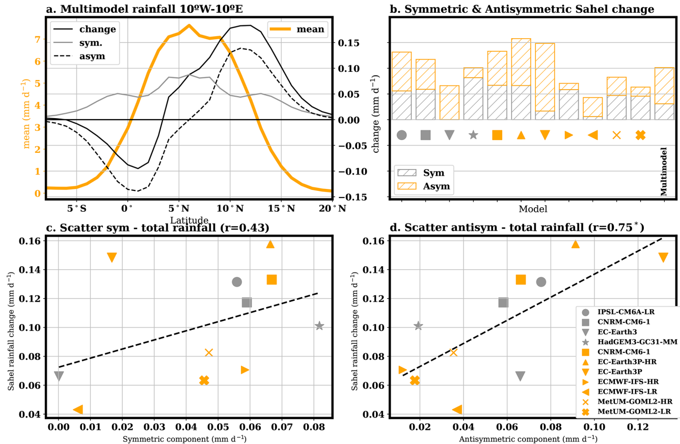
Figure 3. Decomposition of rainfall changes into symmetric and antisymmetric components. (a) Multimodel mean climatology of rainfall in JAS averaged between 10° W and 10° E (orange, left axis, \text{mm d}^{-1} ) and \text{AMV}^+ minus \text{AMV}^- change (black continuous line, right axis, \text{mm d}^{-1} ). The change has been decomposed into symmetric (grey line, right axis) and antisymmetric (dashed line, right axis), relative to the maximum climatological value. (b) Symmetric and antisymmetric components of \text{AMV}^+ minus \text{AMV}^- average rainfall change in the Sahel box (see purple box in Fig. 2b) in JAS for all models and the multimodel mean ( \text{mm d}^{-1} ). (c, d) show scatter plots of rainfall change in the Sahel box as a function of its symmetric and antisymmetric components, respectively ( \text{mm d}^{-1} ). For the models following the PRIMAVERA protocol (marked as orange symbols), only half the anomalies are shown. In the scatter plots, the dashed line shows the linear regression fit, and the correlation coefficient is shown in the title. Correlations are marked with one asterisk if they are statistically significant at the level of \alpha = 0.05 when taking all the models as independent samples. Two asterisks are used if correlations are statistically significant when lowering the number of independent samples to 6.
