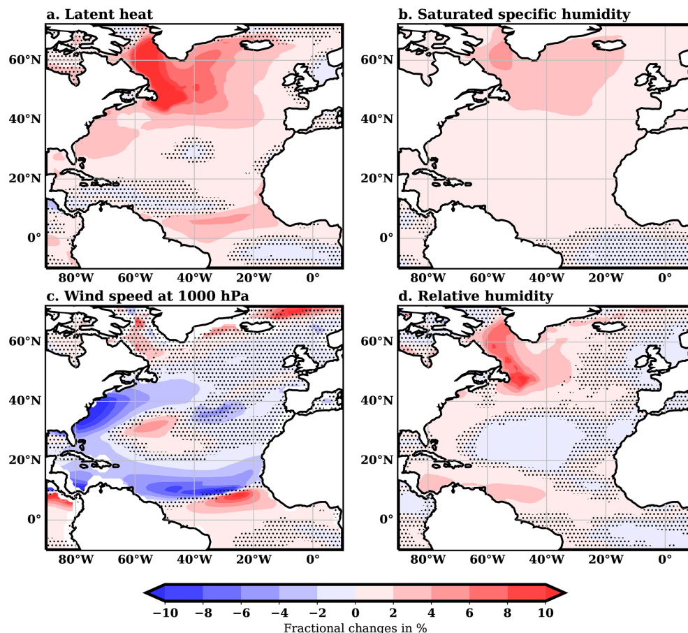
Figure 5. Multimodel mean of fractional changes in AMV^+ minus AMV^- in JAS for: (a) latent heat; (b) saturation specific humidity at surface; (c) wind speed at 1000 hPa; and (d) near-surface relative humidity (plotted as -\delta RH/(1 - \bar{RH}) ). Relative humidity is calculated using near-surface specific humidity and the saturated specific humidity at the surface. The latter is estimated over the ocean by first calculating the saturation vapour pressure based on surface temperature (WMO, 2024) and then transforming it into saturation specific humidity, taking into account sea level pressure. Note that ECMWF-IFS-HR and ECMWF-IFS-LR models were not used for surface calculations since they did not provide near-surface specific humidity. Likewise, EC-Earth3 was not used for wind speed at 1000 hPa. Fractional changes are expressed relative to the climatological values at each grid point, which are calculated as half the sum of AMV^+ and AMV^- simulations. Dots mark regions where fewer than 80 % of the models agree on the sign of changes, and values over land are masked out.
