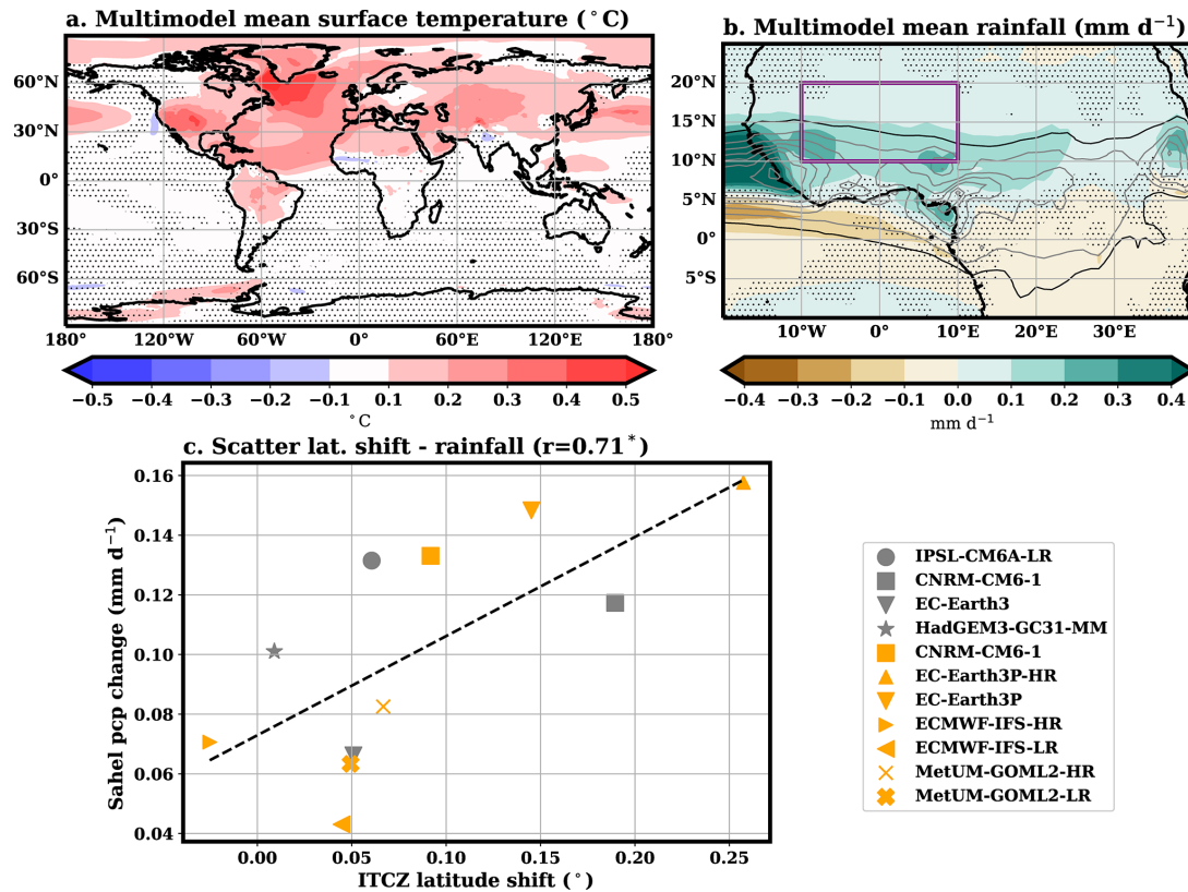
Figure 2. Multimodel mean AMV + minus AMV − change in JAS for: (a) surface temperature (°C) and (b) rainfall over West Africa (mm d −1 ). Dots mark regions where less than 80 % of the models (less than 9 out of 11) agree on the sign of changes. Contours in panel (b) show multimodel mean JAS rainfall (grey contours are drawn every 2 mm d −1 with the starting black contour at 2 mm d −1 ). (c) Scatter plot of Sahel (10° W–10° E, 10–20° N, see purple box in panel b) rainfall change as a function of the ITCZ latitude shift (°) averaged over the 10° W–10° E longitude range. The dashed line shows the linear regression fit, and the correlation coefficient is shown in the title. Correlations are marked with one asterisk if they are statistically significant at the level of \alpha = 0.05 when taking all the models as independent samples. Two asterisks are used if correlations are statistically significant when lowering the number of independent samples to 6. For the models following the PRIMAVERA protocol (marked with orange symbols in the scatter plot), only half the anomalies are shown.
