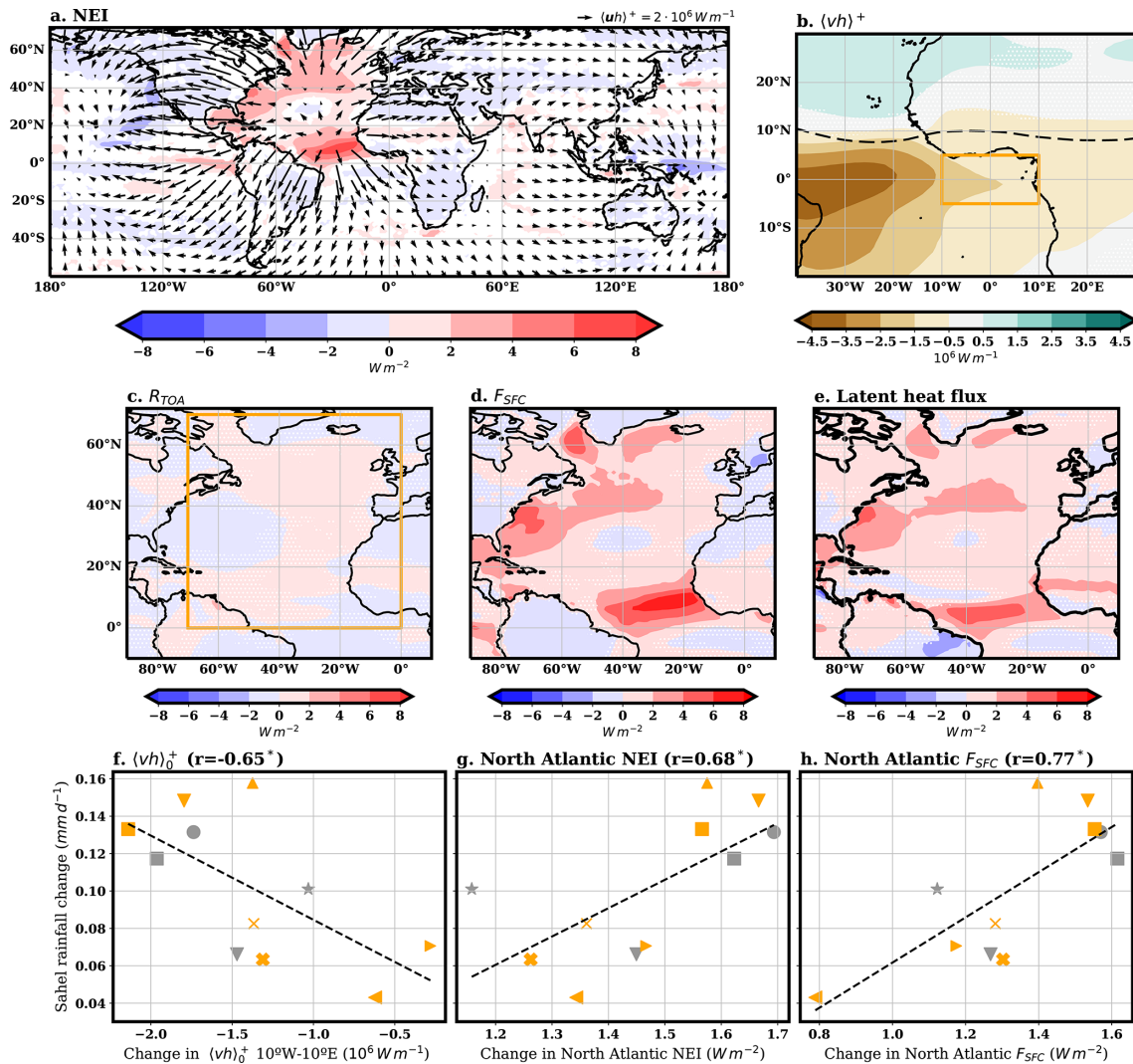
Figure 4. Multimodel average changes in AMV + minus AMV - in JAS for: (a) net energy input (NEI) into the atmospheric column ( \text{W m}^{-2} , shaded) and associated divergent component of the column integrated MSE flux ( \langle uh \rangle^+ , 10^6 \text{ W m}^{-1} , arrows); (b) meridional component of the divergent column integrated MSE flux ( \langle vh \rangle^+ , with meridional wind v , 10^6 \text{ W m}^{-1} ); (c) energy imbalance at TOA ( R_{\text{TOA}} , \text{W m}^{-2} ); (d) energy imbalance at the surface ( F_{\text{SFC}} , \text{W m}^{-2} ); (e) latent heat flux at surface ( \text{W m}^{-2} ). For NEI and the energy imbalances, positive values indicate energy gain for the atmosphere. Scatter plots of averaged Sahel rainfall change ( \text{mm d}^{-1} ) and: (f) strength of the divergent component of the column integrated meridional MSE flux at equatorial latitudes averaged over the Sahel longitudes ( \langle vh \rangle_0^+ , 10^6 \text{ W m}^{-1} , see orange box in panel b); (g) NEI averaged over the North Atlantic ( \text{W m}^{-2} , see orange box in panel c); (h) surface energy imbalance averaged over the North Atlantic ( F_{\text{SFC}} , \text{W m}^{-2} ). For panel (a), anomalies are only shown in regions where at least 80 % (9 out of 11) of simulations agree on their sign. Dots in panels (b)–(e) mark regions where fewer than 80 % of the models agree on the sign of changes. For the models following the PRIMAVERA protocol (marked with orange symbols in the scatter plot), only half the anomalies are shown. The legend for the symbols in the scatter plots is the same as in Fig. 2c. In the scatter panels, the dashed line shows the linear regression fit, and the correlation coefficient is shown in the title. Correlations are marked with one asterisk if they are statistically significant at the \alpha = 0.05 level when considering all models as independent samples. Two asterisks are used if correlations are statistically significant when lowering the number of independent samples to 6.
