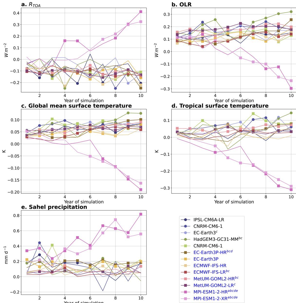
Figure 1. Simulation drifts. Differences between AMV^+ and AMV^- yearly means averaged across all ensemble members for each model vs. simulated year for: (a) global mean net TOA energy imbalance R_{TOA} ( W m^{-2} ); (b) global mean OLR ( W m^{-2} , positive anomalies meaning the Earth is losing more longwave radiation at TOA in AMV^+ than in AMV^- ); (c) global mean surface temperature (K); (d) tropical ( 20^\circ S – 20^\circ N ) mean surface temperature (K); (e) Sahel rainfall (averaged over the 10^\circ W – 10^\circ E , 10 – 20^\circ N box, mm d^{-1} ). For the models following the PRIMAVERA protocol (marked as blue in the model names), only half the anomalies are shown. Solid symbols mark statistically significant differences (two-tailed t -test) in the AMV^+ and AMV^- experiments evaluated separately for each year. Letters a to e next to the model name indicate trends in the variables shown in the corresponding plot that are statistically different from 0 (at the level of \alpha = 0.05 ).
