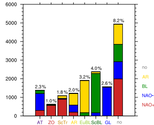
(c) 7+no LC \rightarrow 4 EOF, JJA
