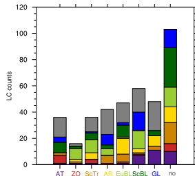
(g) x decay to ... (JJA)
