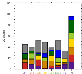
(h) x decay to ... (SON)
