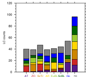
(f) x decay to ... (MAM)
