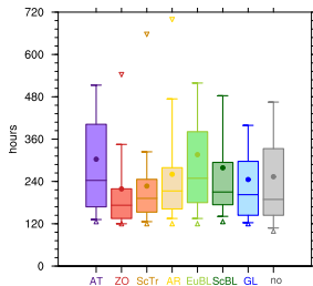
(c) duration (JJA)
