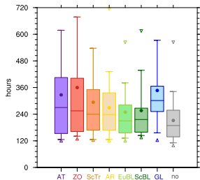
(a) duration (DJF)
