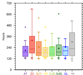
(b) duration (MAM)
