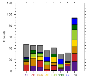
(e) x decay to ... (DJF)
