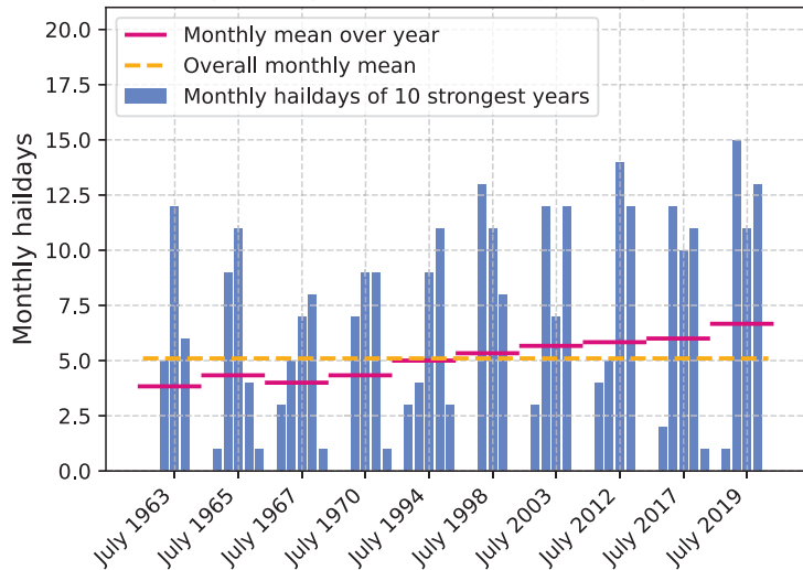
Monthly haildays of the 10 strongest hailyears south
