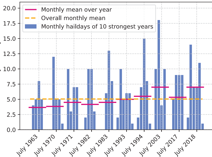
Monthly haildays of the 10 strongest hailyears north
