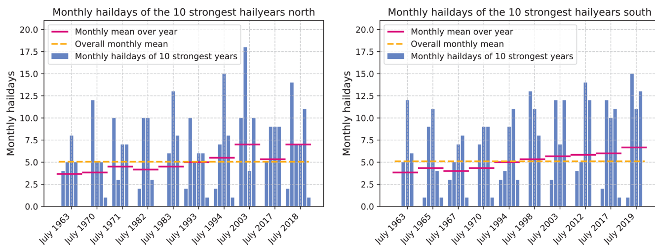
Figure A6. Monthly hail days for the 10 most active hail seasons in (a) northern and (b) southern Switzerland. Blue bars show the number of hail days per month for each of these years. The magenta line indicates the mean monthly hail days within each year, while the yellow dashed line represents the long-term monthly mean across all years. This comparison highlights how the most active hail seasons exceed the climatological average and illustrates the variability of monthly hail activity among these peak seasons in both regions.
