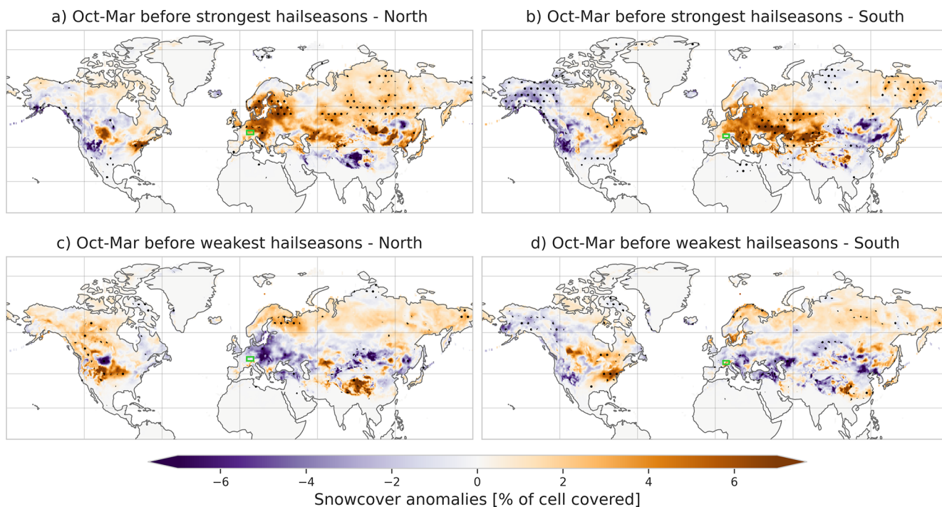
Figure A3. Mean snow cover anomalies over October to March preceding the ten most active and least active hail seasons in northern and southern Switzerland. Panels (a) and (b) show anomalies prior to the most active hail seasons for the northern and southern regions, and panels (c) and (d) show anomalies prior to the weakest hail seasons for the northern and southern regions respectively. Stippling indicates statistical significance at the 95 % confidence level.
