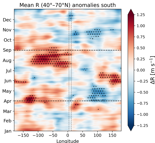
Figure 6. Mean anomalies of the R-metric of 500 hPa meridional wind (averaged between 40 and 70° N) for the ten most active hail seasons in southern Switzerland. The R-metric represents the spatial recurrence of similar large-scale flow patterns. Red colors denote enhanced recurrence, and blue colors indicate reduced recurrence relative to climatology. Stippling marks areas statistically significant at the 95 % confidence level. The grey vertical dashed lines highlight the longitudinal sector of the study region, and the black horizontal dashed lines indicate the beginning and end of the Swiss hail season.
