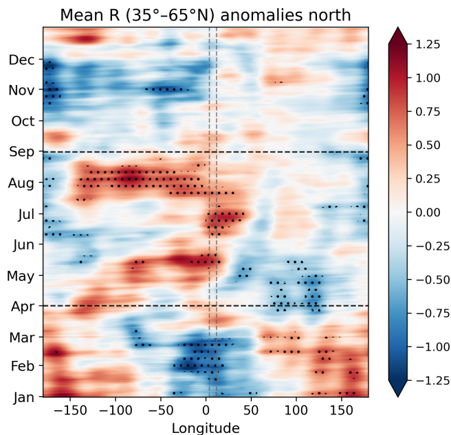
Figure 3. Mean anomalies of the R-metric of 500 hPa meridional wind (averaged between 35 and 65° N) for the ten most active hail seasons in northern Switzerland. Red colors denote enhanced recurrence, and blue colors indicate reduced recurrence relative to climatology. Stippling marks areas statistically significant at the 95 % confidence level. The grey vertical dashed lines highlight the longitudinal sector of the study region, and the black horizontal dashed lines indicate the beginning and end of the Swiss hail season.
