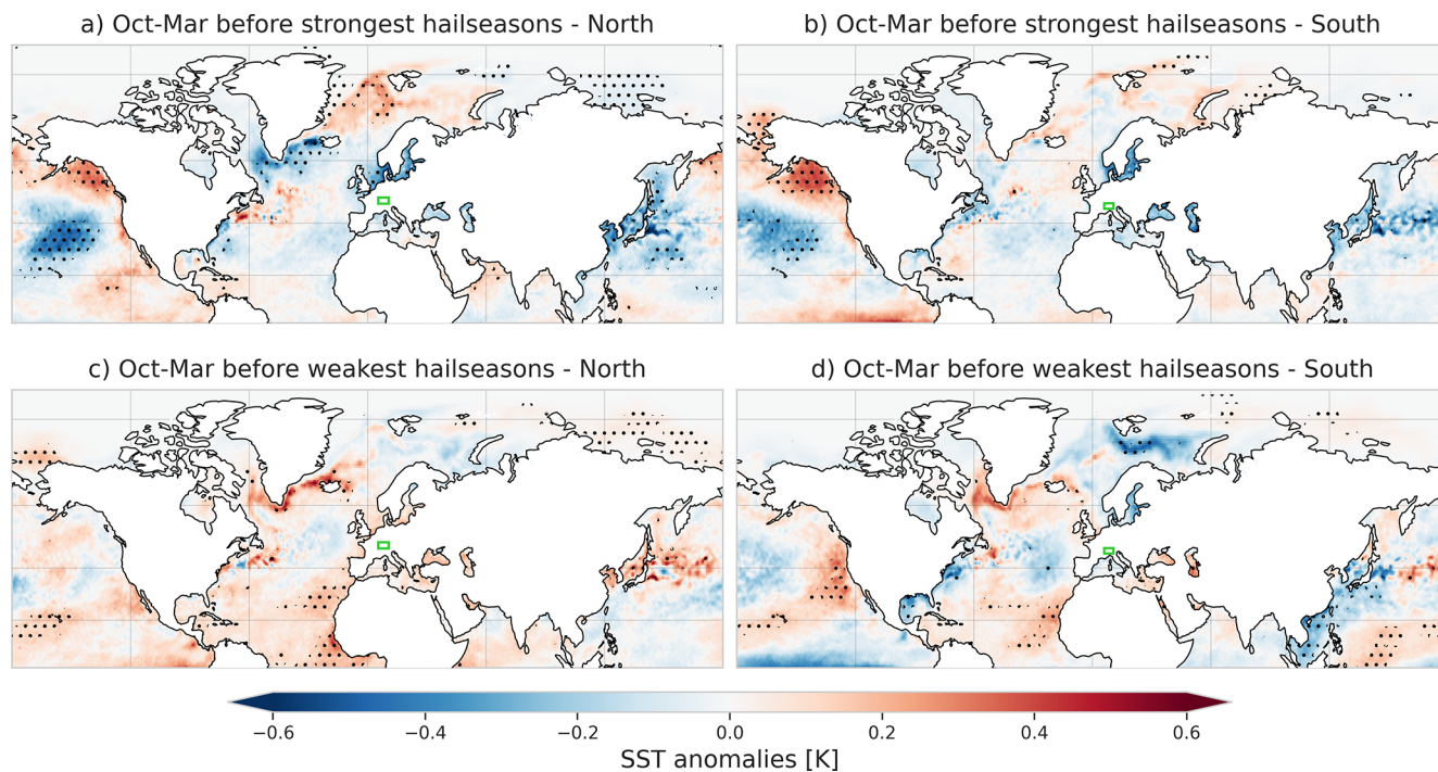
Figure A5. Same as Fig. A3, but for sea surface temperature.
