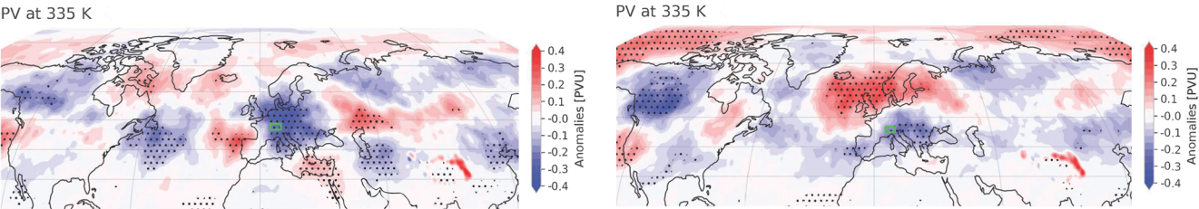
Figure A1. Mean anomalies of PV during the ten most active hail seasons in northern (left) and southern (right) Switzerland. Stippling indicates areas statistically significant at the 95 % confidence level. The green box marks the respective study region.
