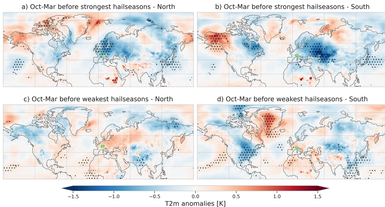
Figure A4. Same as Fig. A3, but for 2 m temperature.
