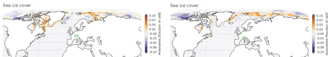
Figure A2. Mean anomalies of sea ice cover during the ten most active hail seasons in northern (left) and southern (right) Switzerland. Stippling indicates areas statistically significant at the 95 % confidence level. The green box marks the respective study region.
