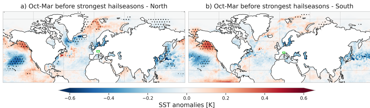
Figure 12. As Fig. 11, but for sea surface temperature.
