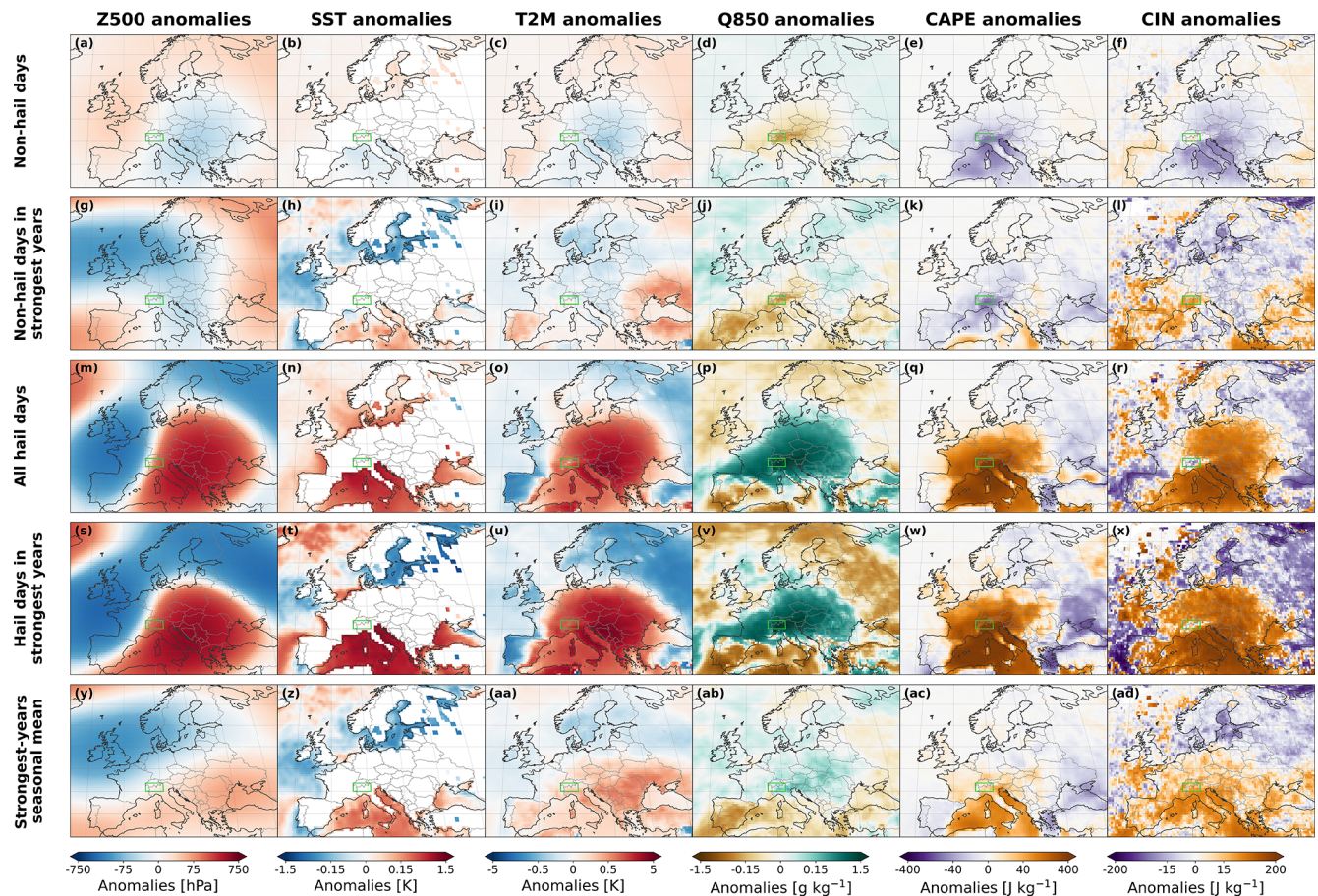
Figure 9. Same as Fig. 8, but for southern Switzerland.
