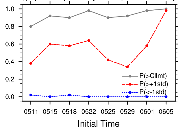
(f) Episode3: probability of Europe Z500 anomaly
