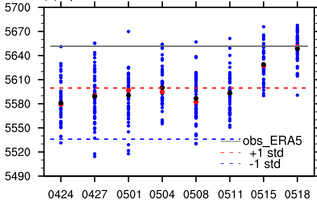
(b) Episode2: S2S ensemble Ural Z500
