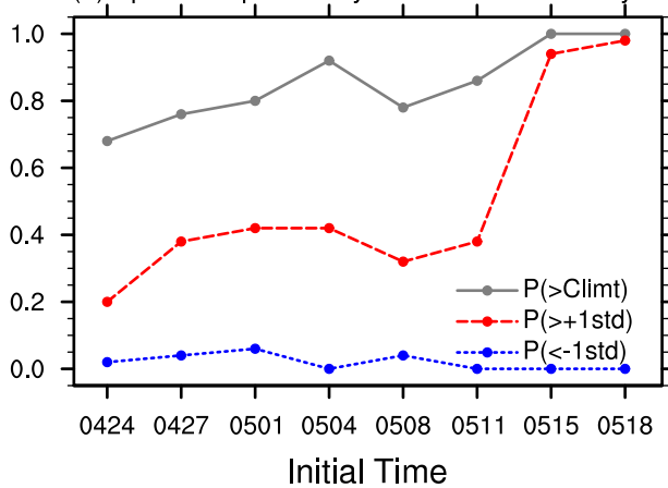
(e) Episode2: probability of Ural Z500 anomaly
