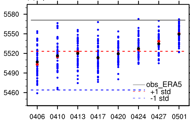
(a) Episode1: S2S ensemble Canada Z500
