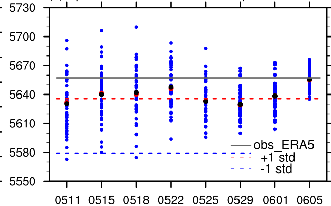
(c) Episode3: S2S ensemble Europe Z500
