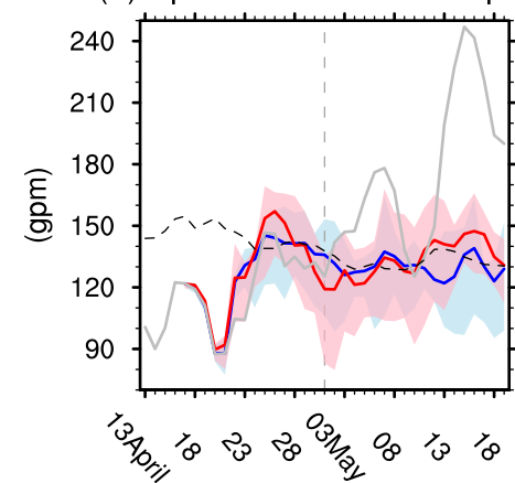
(g) Episode1: Canada Wavenum
