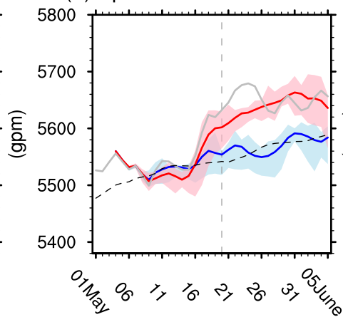
(e) Episode2: Ural Amplit
