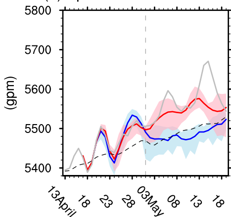
(a) Episode1: Canada Z500
