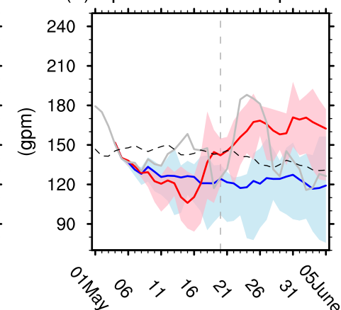
(h) Episode2: Ural Wavenum
