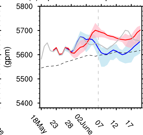
(f) Episode3: Europe Amplit
