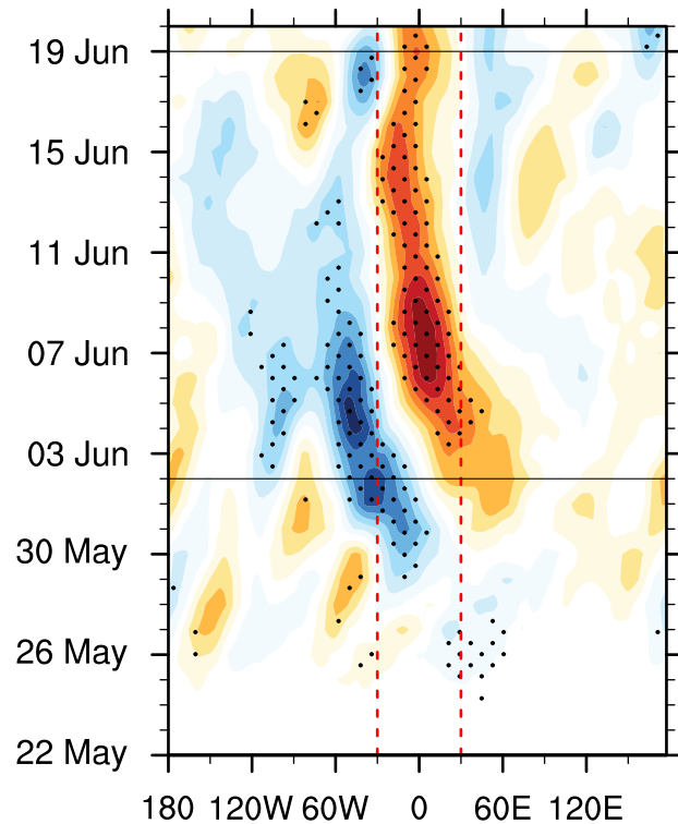
(c) S2S Episode3: Initial@22May
