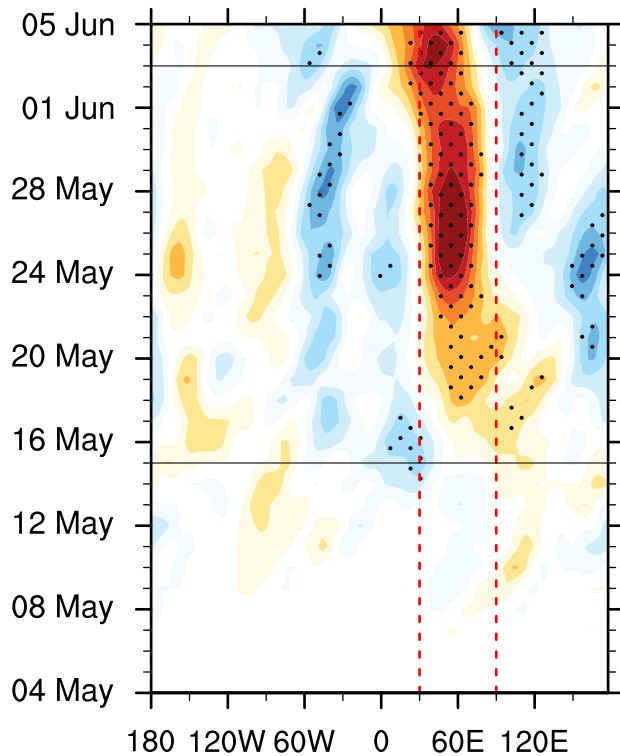
(b) S2S Episode2: Initial@04May
