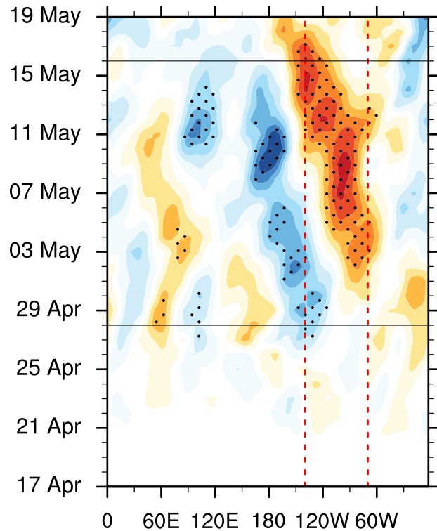
(a) S2S Episode1: Initial@17Apr
