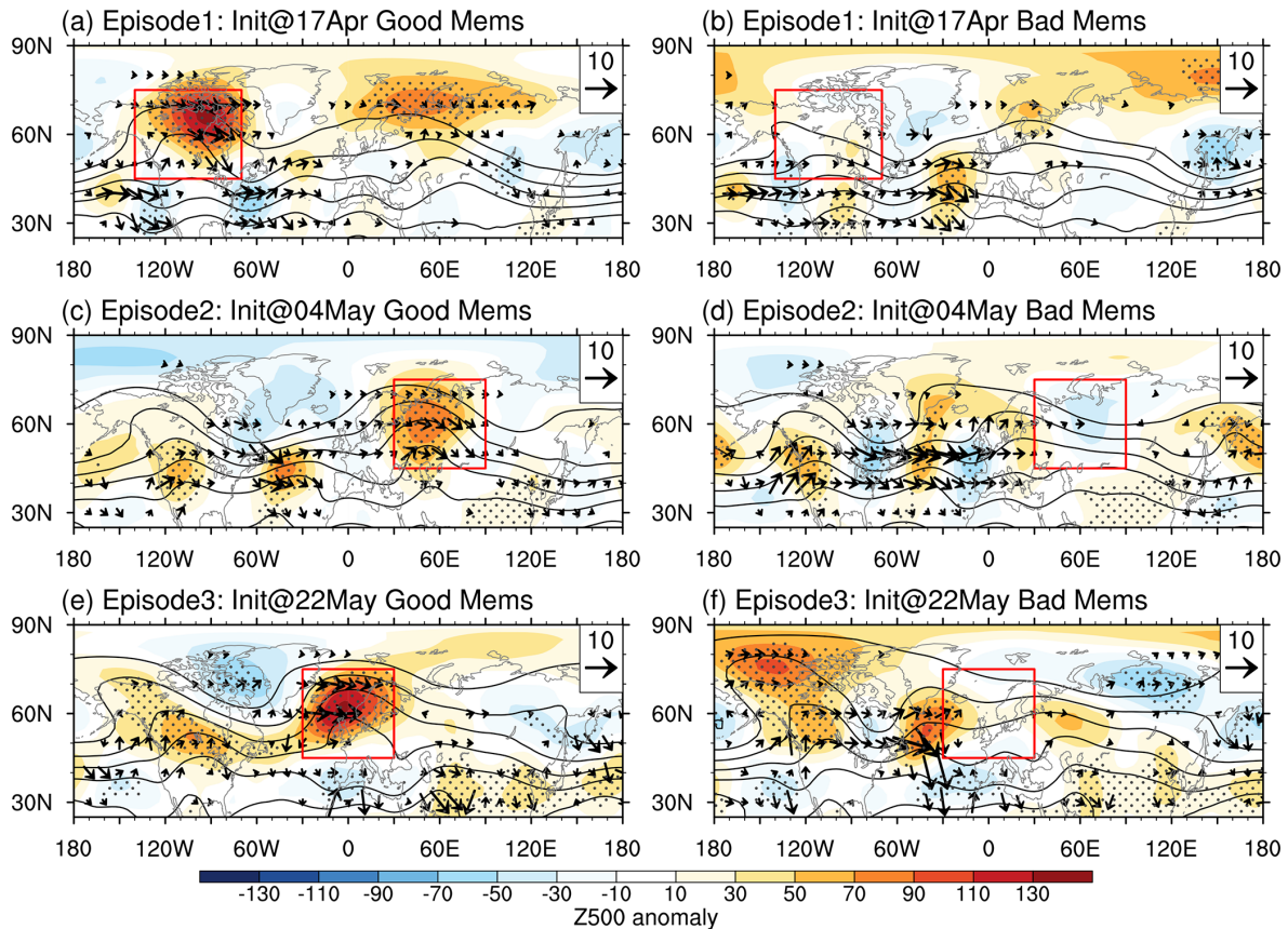
Figure 9. Ensemble-mean Z500 anomalies (shading; units: gpm), associated WAF (vectors; units: \text{m}^2 \text{s}^{-2} ), and Z500 (contours; units: gpm) for good ensemble members (a, c, and e) and bad ensemble members (b, d, and f). Three panels from top to bottom correspond to the Canadian blocking (initialized at 17 April; a and b), Ural blocking (initialized 4 May; c and d), and European blocking (initialized 22 May; e and f). Red boxes mark the blocking regions. Stippling denotes ensemble-mean Z500 anomalies exceeds 0.8\sigma based on ERA5.
