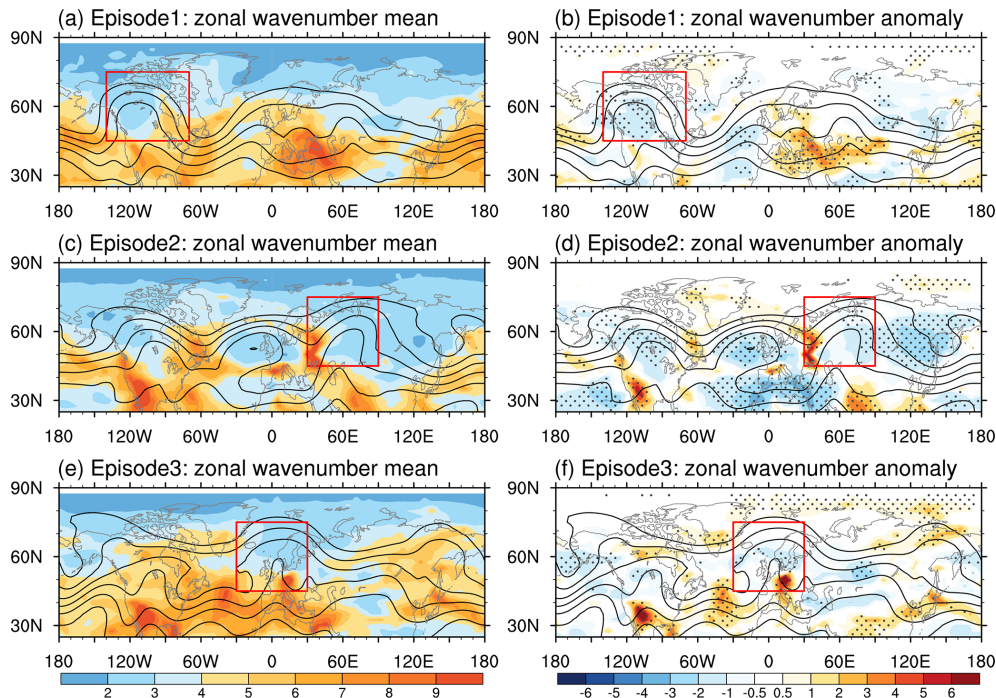
Figure 4. Time-mean zonal wavenumber (shading; left panels: a , c , and e ) and its anomalies (shading; right panels: b , d , and f ) at 500 hPa averaged during ( a , b ) episode 1, ( c , d ) episode 2, and ( e , f ) episode 3. Stippling in the right panels indicates anomalies exceeding 1\sigma . Black solid contours show the corresponding time-mean Z500.
