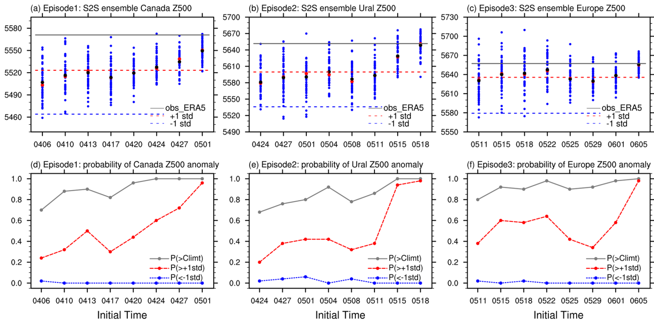
Figure 6. (a–c) ECMWF S2S forecasted time- and spatially averaged Z500 for episode 1 (a), episode 2 (b), and episode 3 (c). The three panels (from left to right) correspond to averages over the Canada (a), the Ural Mountains (b), and Europe (c), respectively. Each blue dot represents one of the 50 ensemble members. Black (red) dots denote the ensemble mean (median). In each episode, the solid gray line shows the observed time- and spatially averaged Z500 in 2023 from ERA5, while the red and blue dashed lines indicate the observed +1\sigma and -1\sigma bounds based on ERA5 from 1979–2023, respectively. (d–f) Probabilities of forecasted time-mean Z500 exceeding the climatological mean (gray line), exceeding +1\sigma (red line), and falling below -1\sigma (blue line) as a function of initialization date for episode 1 (d), episode 2 (e), and episode 3 (f). The abscissa represents forecast initialized dates with twice weekly.
