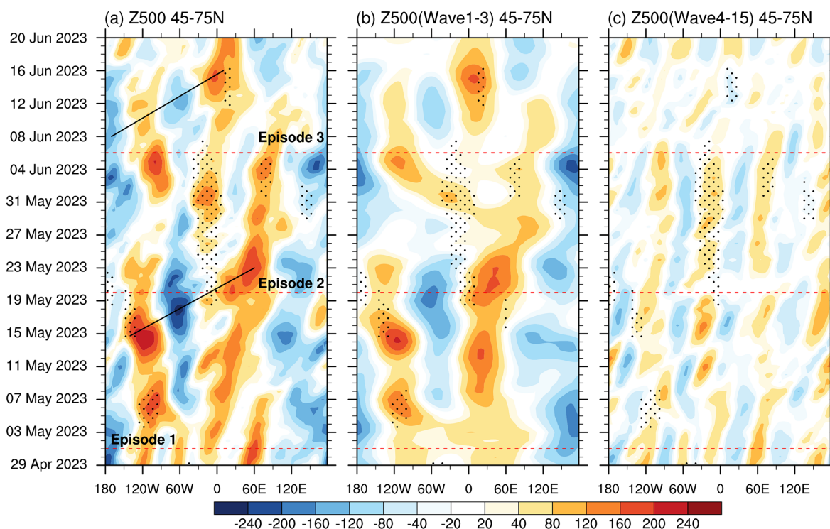
Figure 2. Hovmöller diagrams of zonal-mean-removed (a), 1–3-wave (b) and 4–15-wave (c) Z500 (units: gpm) averaged over 45–75°N during three successive episodes in May–June 2023. Black lines in (a) show the downstream development of Rossby waves. Black dots mark the locations of identified large-scale blocking events.
