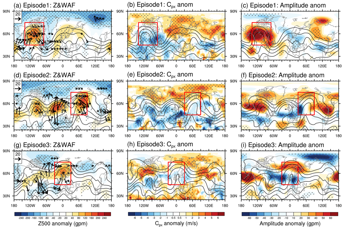
Figure 3. Anomalies of Z500 (shading; left panels, a , d , and g ; units: gpm), zonal phase speed (shading; middle panels, b , e , and h ; units: \text{m s}^{-1} ), and wave amplitude (shading; right panels, c , f , and i ; units: gpm) at 500 hPa during ( a–c ) episode 1, ( d–f ) episode 2, and ( g–i ) episode 3. Stippling indicates anomalies exceeding 1\sigma . Solid black contours show the corresponding time-mean Z500. Vectors in the left panels represent the wave activity flux at 500 hPa (units: \text{m}^2 \text{s}^{-2} ).
