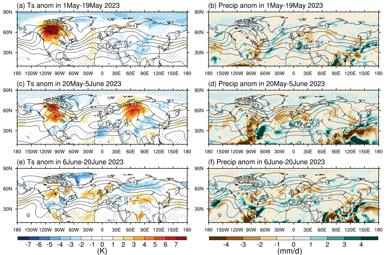
Figure 1. Anomalies of surface temperature (shading; left panels, a , c , and e ; units: K) and precipitation (shading; right panels, b , d , and f ; units: \text{mm d}^{-1} ) during three successive episodes in 2023: 1–19 May ( a , b ), 20 May–5 June ( c , d ), and 6–20 June ( e , f ). Stippling indicates regions where the anomalies of surface temperature or precipitation exceed 1 standard deviation ( 1\sigma ). Solid black contours show the corresponding time-mean 500 hPa geopotential height ( Z_{500} ).
