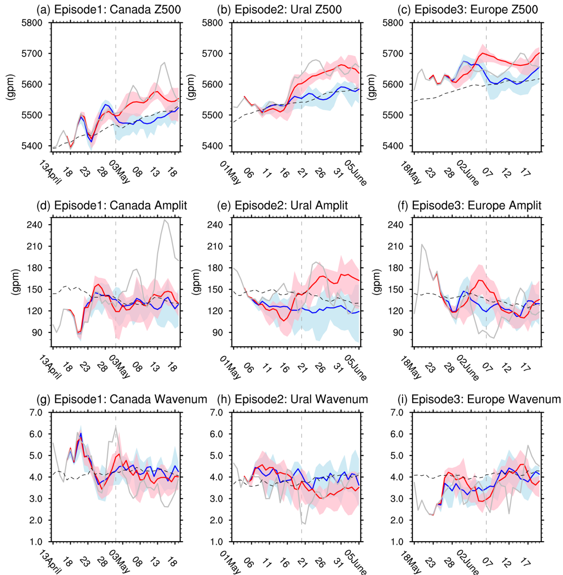
Figure 7. Daily evolution of ECMWF S2S forecasted spatially averaged Z500 ( a–c ; units: gpm), wave amplitude ( d–f ; units: gpm), and zonal wavenumber ( g–i ) at 500 hPa during different episodes. The three panels (from left to right) correspond to averages over the Canada (initialized at 17 April; a , d , and g ), the Ural Mountains (initialized at 4 May; b , e , and h ), and Europe (initialized at 22 May; c , f , and i ), respectively. In each panel, red and blue solid lines represent the ensemble means of the good-forecast ensemble members and bad-forecast ensemble members, respectively, while the pink and light blue shading indicate the 20%–80% spread of the good and bad members, respectively. The gray solid line and the black dashed line denote the observed daily evolution in 2023 and observed daily climatology based on ERA5, respectively. Vertical gray dashed lines mark the onset day of each episode.
