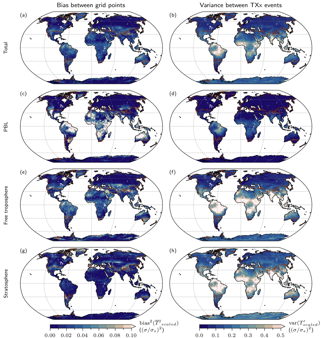
Figure 5. Distribution of (left) \text{bias}^2(\overline{T'}_{\text{scaled}}) and (right) \text{var}(T'_{\text{scaled}}) , vertically averaged over (a, b) all hybrid sigma–pressure levels, (c, d) only the PBL, (e, f) only the free troposphere, and (g, h) only the stratosphere. The brown lines denote the boundaries between the three clusters. The coldest 10 TXx events are excluded at each grid point. Note the different scales used for \text{bias}^2(\overline{T'}_{\text{scaled}}) and \text{var}(T'_{\text{scaled}}) .
