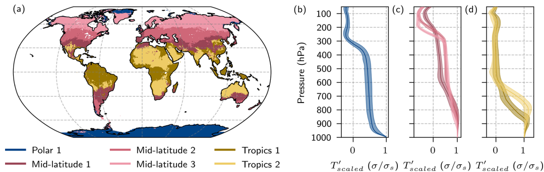
Figure 4. Refinement of the global area-weighted clustering with now six clusters over land: (a) map of clusters polar 1 (dark blue, N = 30\,127 grid points), mid-latitude 1 (red, N = 9124 ), mid-latitude 2 (dark pink, N = 10\,312 ), mid-latitude 3 (light pink, N = 17\,422 ), tropics 1 (brown, N = 11\,299 ), and tropics 2 (yellow, N = 9865 ). (b–d) Median and interquartile range of the vertical median scaled T' profile of all the grid points within each cluster for the (b) polar, (c) mid-latitude, and (d) tropical clusters on pressure levels (surface pressure set again to the reference pressure 1000 hPa).
