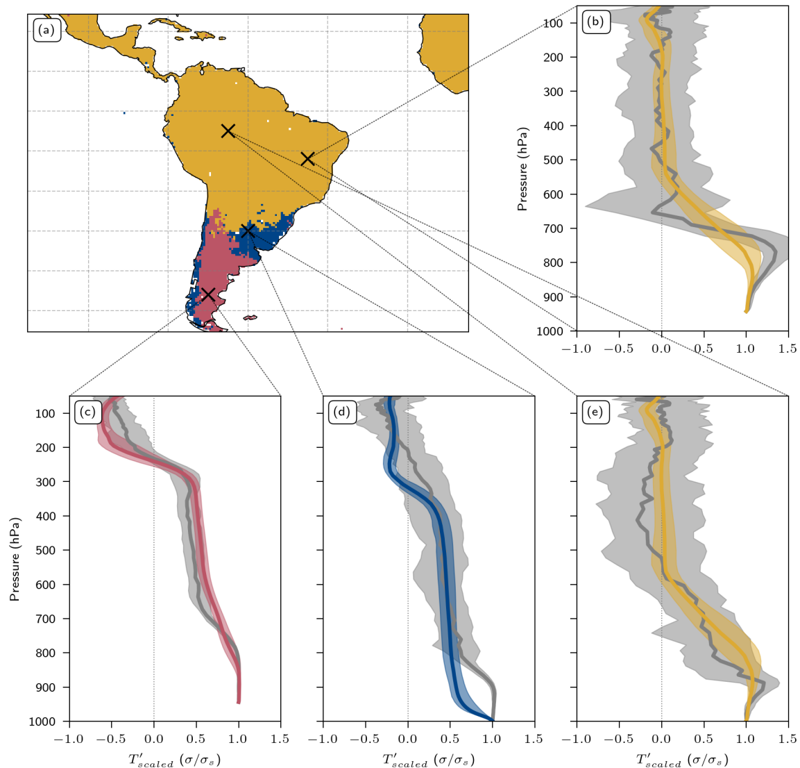
Figure D3. Area-weighted k -means clustering with three clusters from Fig. 2a shown as (a) a zoomed in map of South America and (b–e) vertical T'_{\text{scaled}} profiles for individual grid points, (b) 12^{\circ}\text{S} , 45^{\circ}\text{W} , (c) 46^{\circ}\text{S} , 70^{\circ}\text{W} , (d) 30^{\circ}\text{S} , 60^{\circ}\text{W} , and (e) 5^{\circ}\text{S} , 65^{\circ}\text{W} . The grey line and its shading denote the median and interquartile range of all TXx events at that grid point, the yellow, red, and blue lines and shading the clusters' median and interquartile range of all T'_{\text{scaled}} within the tropical, mid-latitude, and polar clusters, respectively. For the cluster T'_{\text{scaled}} profiles, we use the median surface pressure of the TXx events as a reference pressure to interpolate on pressure levels.
