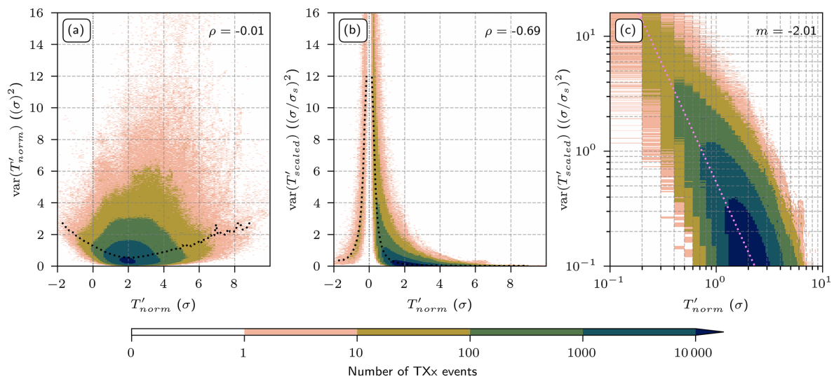
Figure 7. Joint distributions of the mean vertical variance of individual TXx event profiles relative to their median profile and near-surface T'_{\text{scaled}}(k=0) (lowest model level), (a) for T'_{\text{norm}} , (b) T'_{\text{scaled}} , and (c) T'_{\text{scaled}} in log-log-scale. The values of \rho in the upper right corner in panels (a) and (b) denote the Spearman correlation (both p -values < 10^{-3} ). Bin widths are 0.1\sigma ( x -axis) and 0.02\sigma or 0.02\sigma/\sigma_s ( y -axis). The black dotted line marks the weighted median. The violet dotted line and the m value in the upper right corner in panel (c) indicate the regression line and slope, respectively. Note that the negative T'_{\text{scaled}}(k=0) values on the x -axes arise from our event definition and make up 0.03 % of the TXx events.
