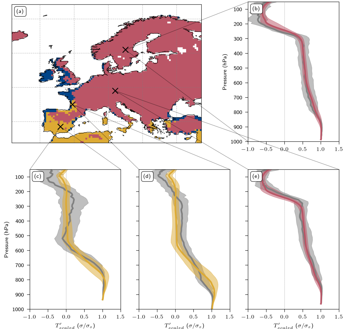
Figure D1. Area-weighted k -means clustering with three clusters from Fig. 2a shown as (a) a zoomed in map of Europe and (b–e) vertical T'_{\text{scaled}} profiles for individual grid points at (b) 61° N, 15° E, (c) 38.5° N, 4° W, (d) 45° N, 0.5° W, and (e) 49° N, 12° E. The grey line and its shading denote the median and interquartile range of all TXx events at that grid point, the yellow, red, and blue lines and shading the clusters' median and interquartile range of all T'_{\text{scaled}} within the tropical, mid-latitude, and polar clusters, respectively. For the cluster T'_{\text{scaled}} profiles, we use the median surface pressure of the TXx events as a reference pressure to interpolate on pressure levels.
