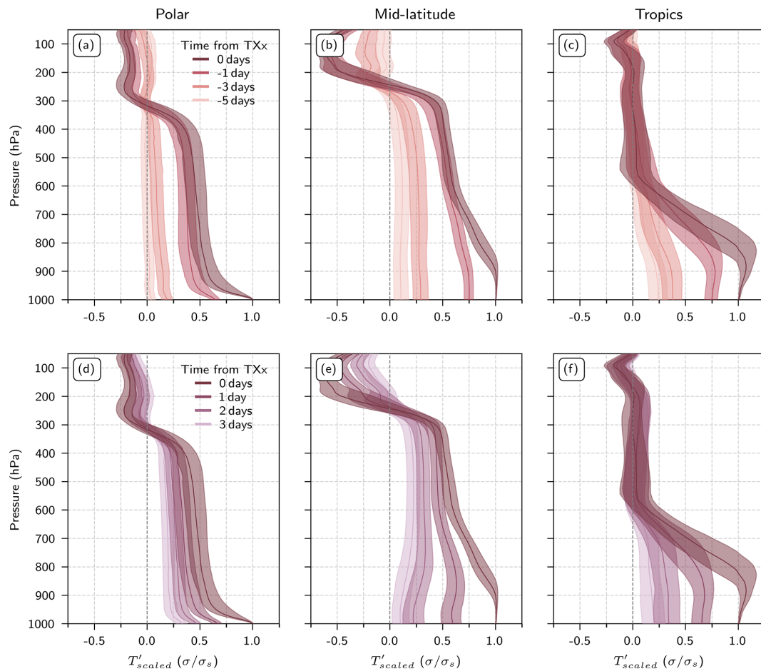
Figure 3. Temporal evolution of the median and interquartile range of the median scaled temperature anomalies ( T'_{\text{scaled},C} ) of all the grid points (a–c) during the 5 d genesis and (d–f) 3 d decay of TXx events for (a, d) the polar, (b, e) mid-latitude, and (c, f) tropical clusters. The surface pressure is set again to a reference pressure of 1000 hPa.
