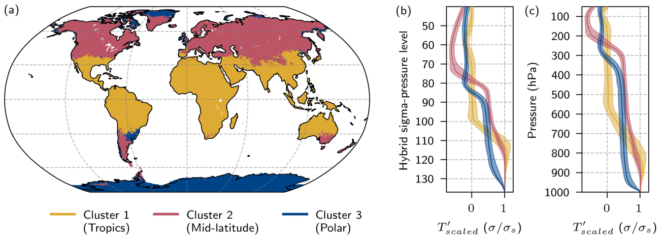
Figure 2. (a) Global distribution of the three area-weighted clusters over land: cluster 1 (yellow, N = 26\,325 grid points), cluster 2 (red, N = 30\,138 ), and cluster 3 (blue, N = 31\,626 ). (b, c) median and interquartile range of the median vertical T'_{\text{scaled}} profiles of all grid points in each cluster, (b) on sigma-hybrid model levels and (c) on pressure levels (surface pressure set to the reference pressure 1000 hPa).
