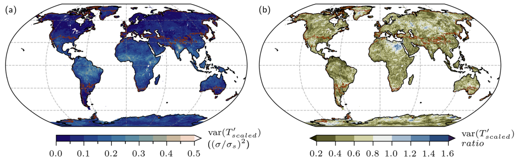
Figure 6. (a) Variance of T'_{\text{scaled}} profiles for the 10 hottest TXx events relative to the median profile of all TXx events ( \text{var}(T'_{\text{scaled}}) ), and (b) the ratio of \text{var}(T'_{\text{scaled}}) between the hottest 10 TXx events and moderate TXx events (which exclude the hottest and coldest 10 TXx events). Fields in both panels are vertically averaged over all hybrid sigma–pressure levels. The brown lines denote the boundaries between the three clusters.
