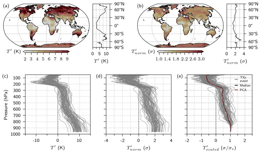
Figure 1. Global distribution of the (a) median temperature anomaly ( T' ) and (b) median normalised temperature anomaly ( T'_{\text{norm}} ) on the lowermost model level, of TXx events from 1951 to 2023. Vertical profiles (grey lines) of (c) T' , (d) T'_{\text{norm}} , and (e) scaled temperature anomaly ( T'_{\text{scaled}} ) of all TXx events at a land grid point in central Europe ( 49^\circ\text{N} , 12^\circ\text{E} ), marked in panels (a) and (b) with a red cross. The black and red lines in panel (e) show the median profile of T'_{\text{scaled}} ( \overline{T'_{\text{scaled}}} ) over all TXx events and \overline{T'_{\text{scaled}}} after the PCA, respectively (see Sect. 2.3 for details).
