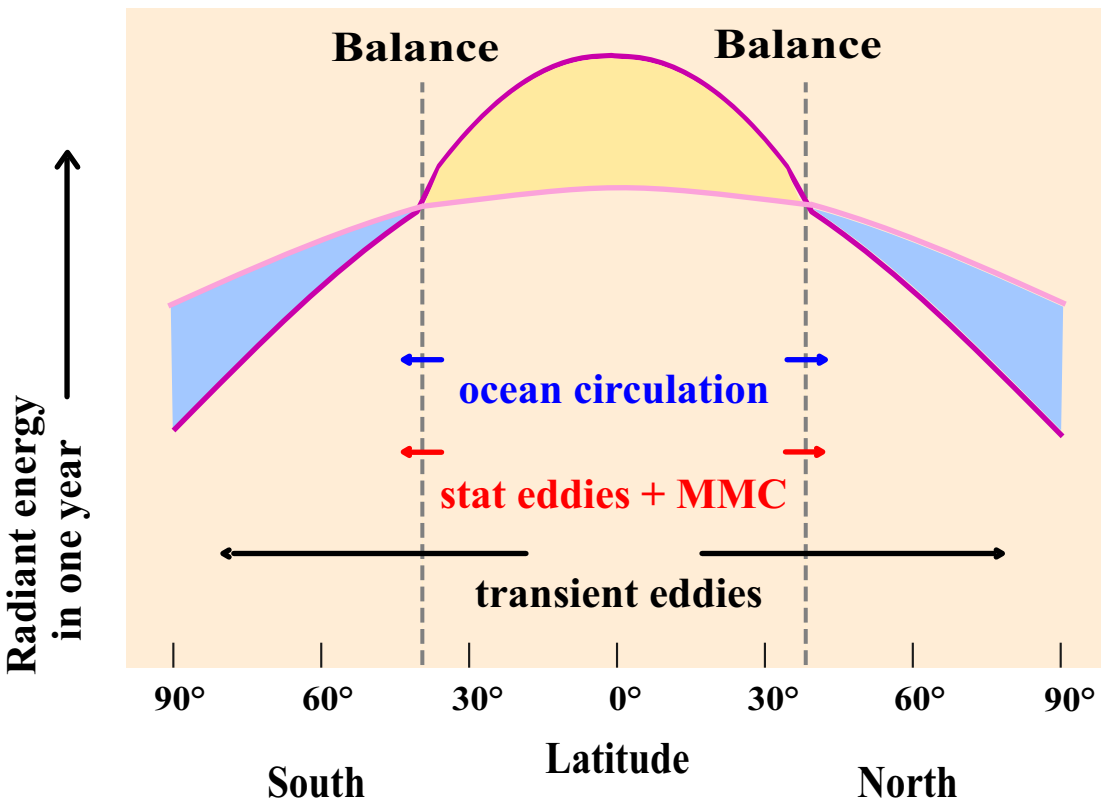
(a) aquaplanet
