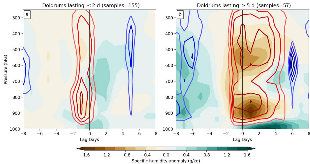
Figure 7. Hovmöller centred on the first day of doldrums formation for Davies Reef (18.75°S, 147.75°E) from 1000 to 250 hPa. Specific humidity anomalies (shading) and omega anomalies (contours, every 0.01 Pa s -1 starting from 0.02) for short and long duration doldrums are shown. Red contours denote positive (descending) anomalies while blue denotes negative (ascending) anomalies.
