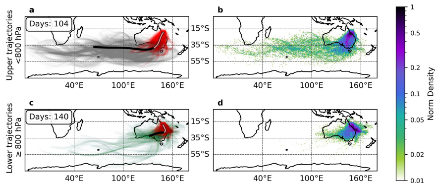
Figure 8. Density plot of the back trajectories launched from Davies Reef that descend > 250 hPa in 48 h from their launch time. Trajectories run for 5 d with 6 hourly time steps. The top row shows those that launched from < 800 hPa and the bottom row shows trajectories launched from ≥ 800 hPa. In panels (a) and (c) the red trajectories mark when the parcel is within 48 h of their launch time with the mean trajectory path marked by the solid line (black prior to 48 h, pale red after 48 h). Panels (b) and (d) show the normalised density plots of the upper and lower trajectories.
