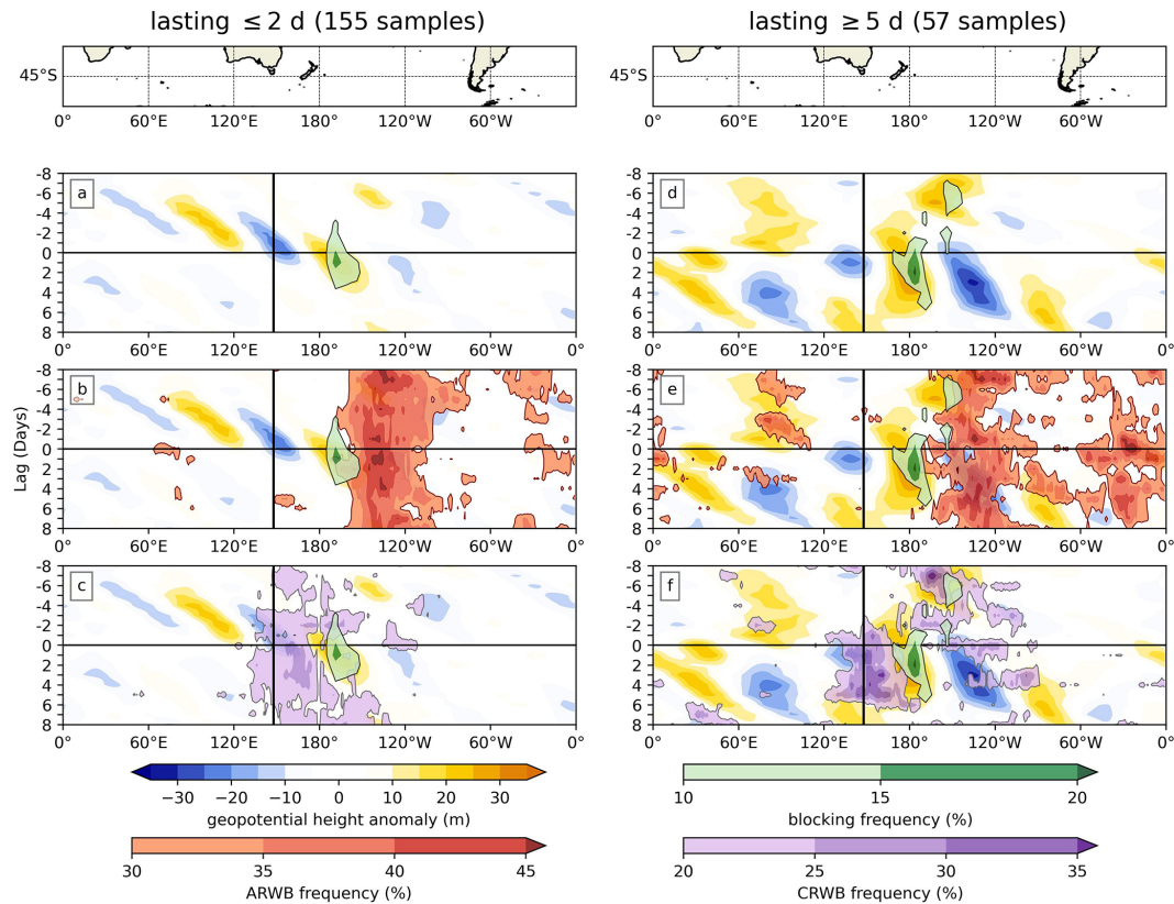
Figure 2. Hovmöller diagrams averaged over 24–66°S for lead-lag composites of 500 hPa geopotential height anomalies (blue/yellow), blocking frequency (green, a , d ), anticyclonic Rossby wave breaking (ARWB) frequency (red, b , e ) and cyclonic Rossby wave breaking (CRWB) frequency (purple, c , f ). All lead-lag composites are centred on the first day of the doldrums formation (day 0, horizontal line). The vertical line marks the longitude of Davies Reef and the GBR (148°E).
