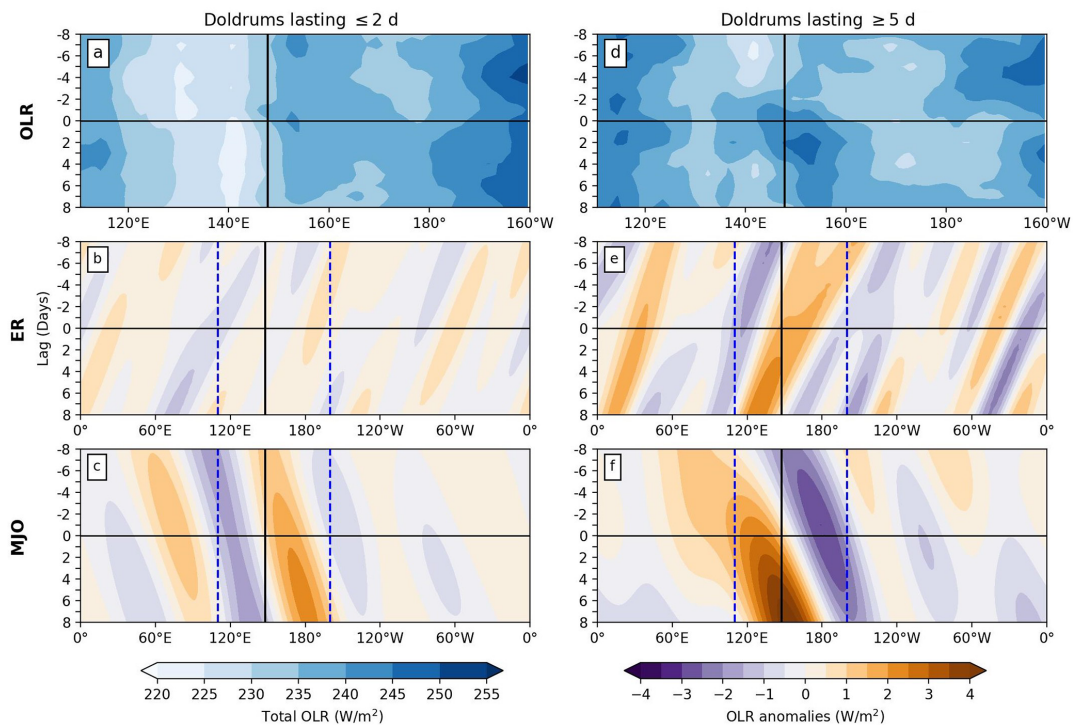
Figure 10. 0–25° S averaged Hovmöller diagrams centred on the first day of the doldrums formation. Top row shows the total OLR between 110° E and 160° W (region marked with blue lines in middle and bottom rows), middle row the ER wave filtered OLR anomalies and bottom row the MJO OLR anomalies. Here positive (negative) anomalies represent suppressed (enhanced) convection. On each panel the vertical line marks the longitude of Davies Reef within the GBR (148° E).
