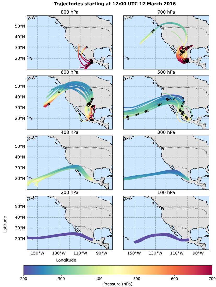
Figure S3. Lagrangian 72-hour backward trajectories over Mexico City during the STE event in March 2016, dynamically linked to Rossby wave breaking and the cut-off low (Fig. 5). Backward trajectories starting at 12:00 UTC on 12 March 2016 and 00:00 UTC on 13 March 2016. Trajectories were calculated with LAGRANTO using ERA5 reanalysis fields and initialized over the Mexico City region (Longitude: 100°W to 98°W, Latitude: 18.5°N to 20°N) at levels between 700 hPa and 100 hPa (700 hPa accounts for Mexico City's 2,300 m meters above mean sea level). At the initial time, the horizontal distance between parcels is 50 km at each level. Trajectories illustrate downward intrusion along the sloping tropopause fold into 300–700 hPa.
