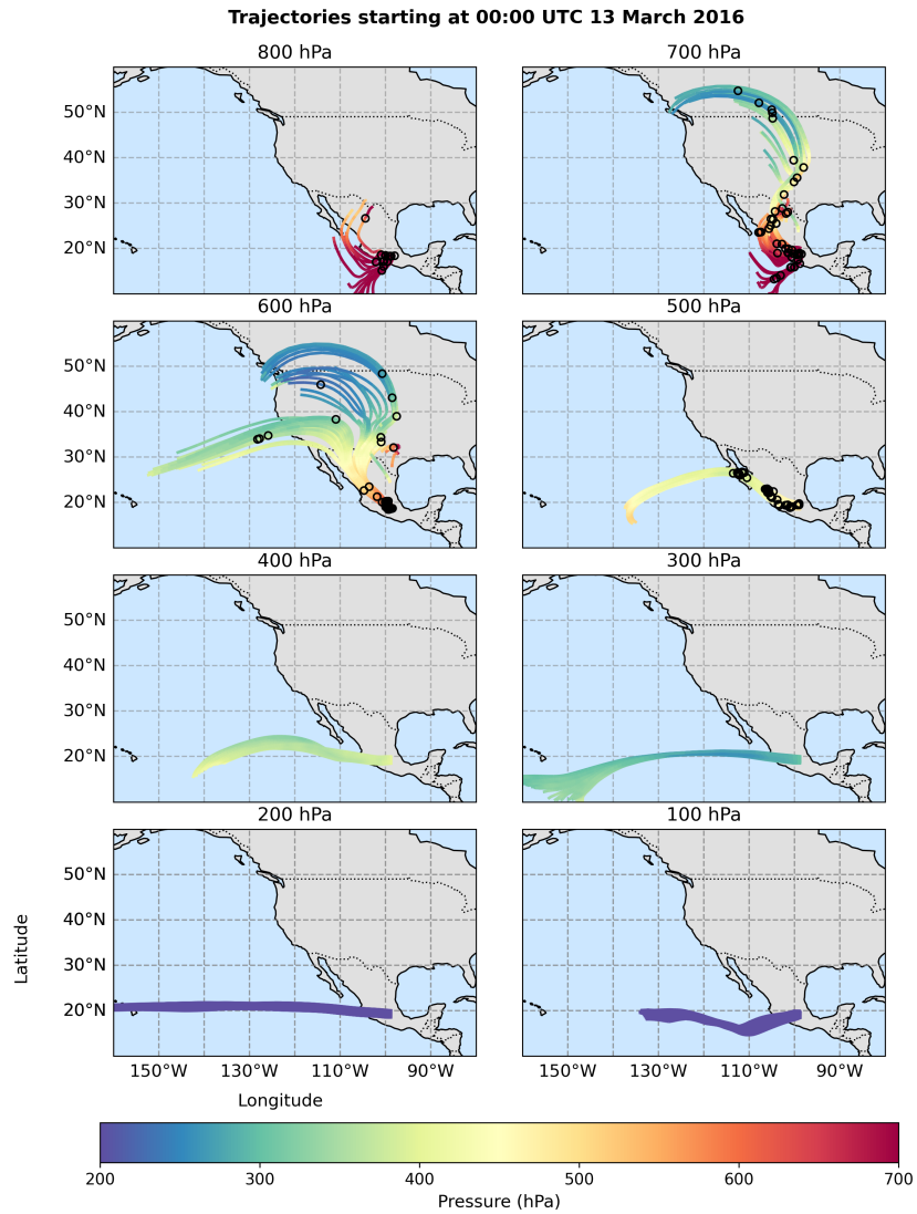
Figure S3 (continued from the previous page). Backward trajectories starting at 00:00 UTC on 13 March 2016.
