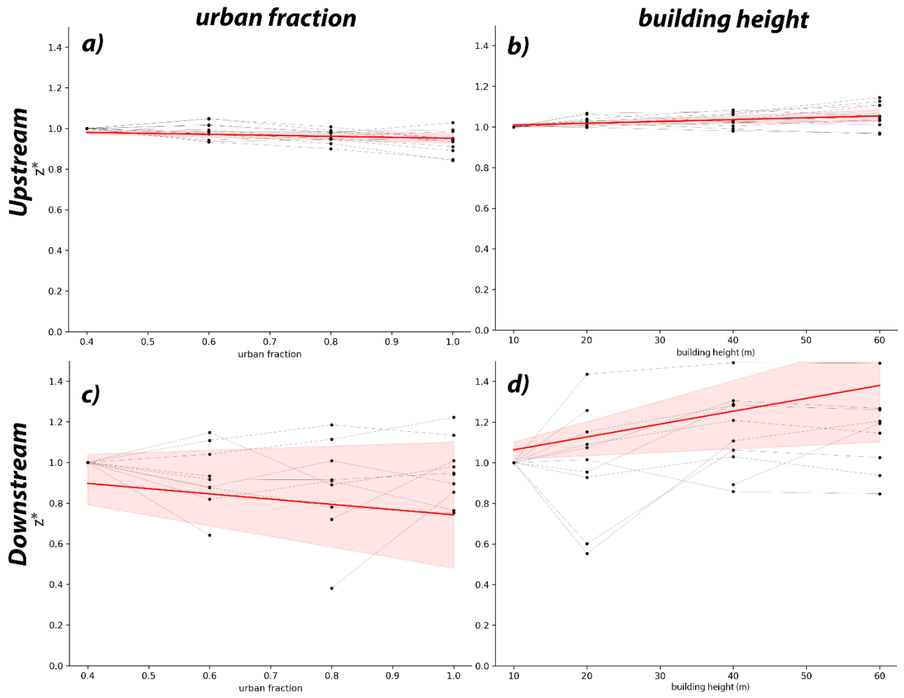
Figure S4: As in Figure S4, but for the urban fraction numerical experiment in a) and c), and for the building height experiment in b) and d).
