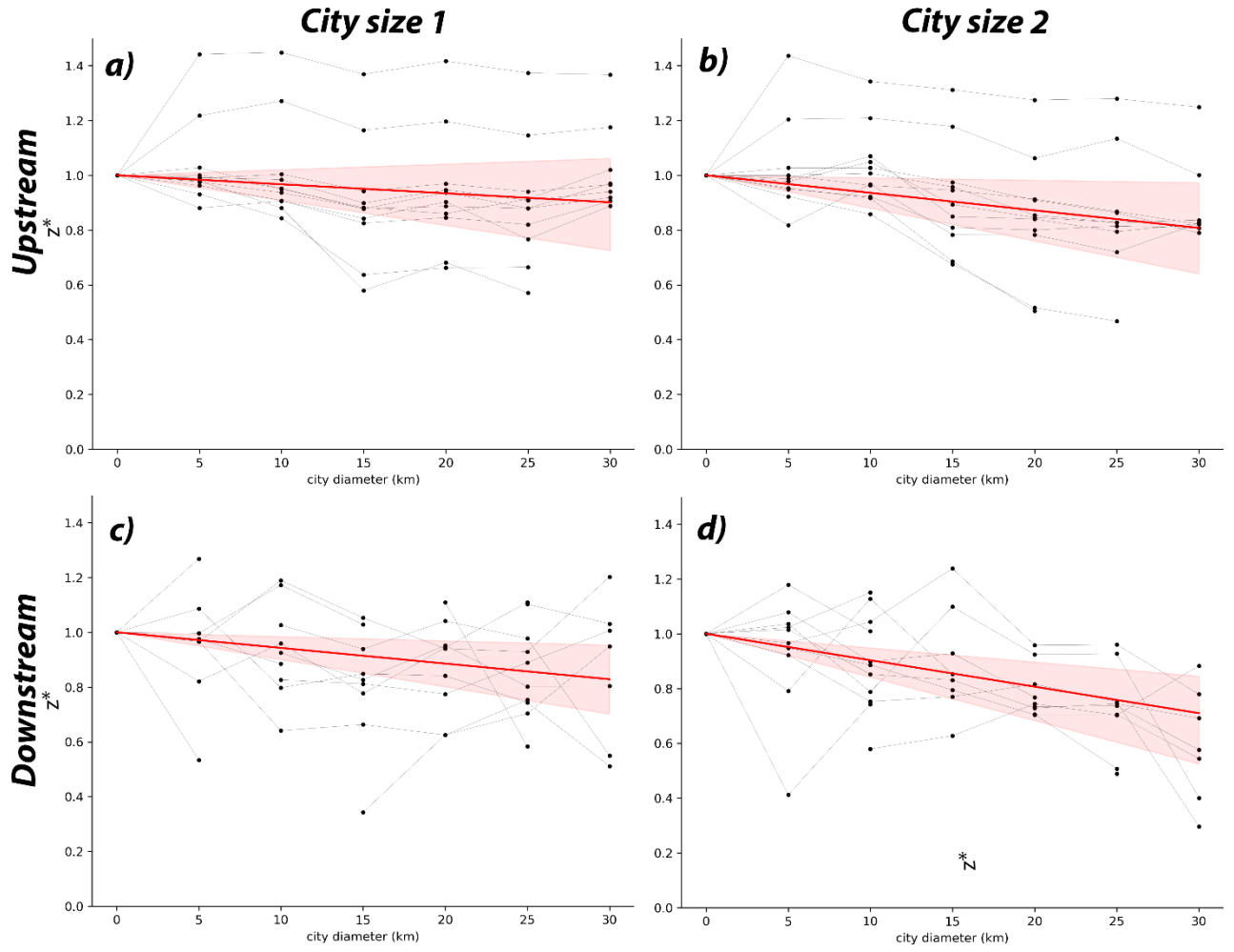
Figure S3: Normalized mean UH ( z^* ) in each ensemble member (black dots) of the city size 1 set of experiments in function of the city diameter (km) in the a) upstream region and c) downstream region. Ensemble members obtained with the same seed are connected. The mean linear fit is shown with a red line, while the 5-95% confidence interval is red shaded. b) and d) as in a) and c), respectively, but for the city size 2 numerical experiments.
