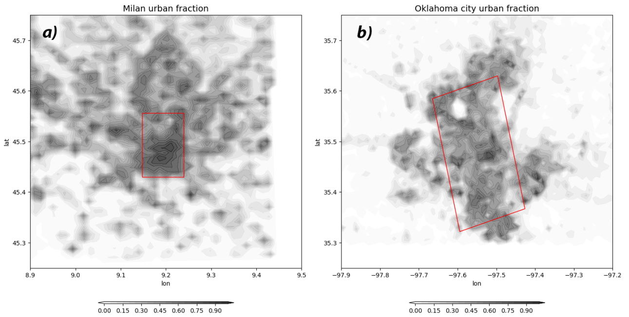
Figure S2: Urban fraction of (a) Milan and (b) Oklahoma city. The red boxes show the area within where the GLOBUS parameters are averaged.
