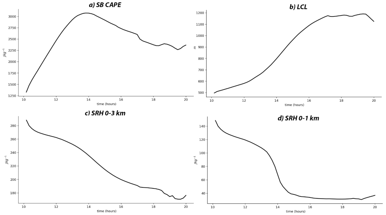
Figure S1: Time evolution of domain-averaged (a) SB CAPE, (b) LCL, (c) SRH in the 0-3 km layer, and (d) SRH in the 0-1 km layer. No convection is triggered in the simulation considered to produce these plots.
