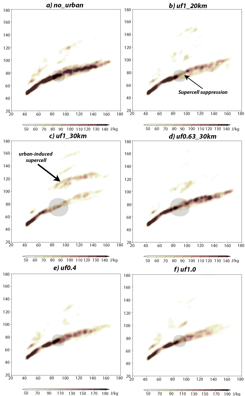
Figure 6. Cumulated UH ensemble mean in (a) the no_urban experiment (Table 5), (b) in the uf1_20km experiment, (c) in the uf1_30km experiment, (d) in the uf0.63_30km experiment (Table 4), (e) in the uf0.4 experiment (Table 6), (f) in the uf1.0 experiment. The city is highlighted in grey shading. In panel (a) the city of the 20km experiment is shown just for reference, in the experiment there are croplands everywhere.
