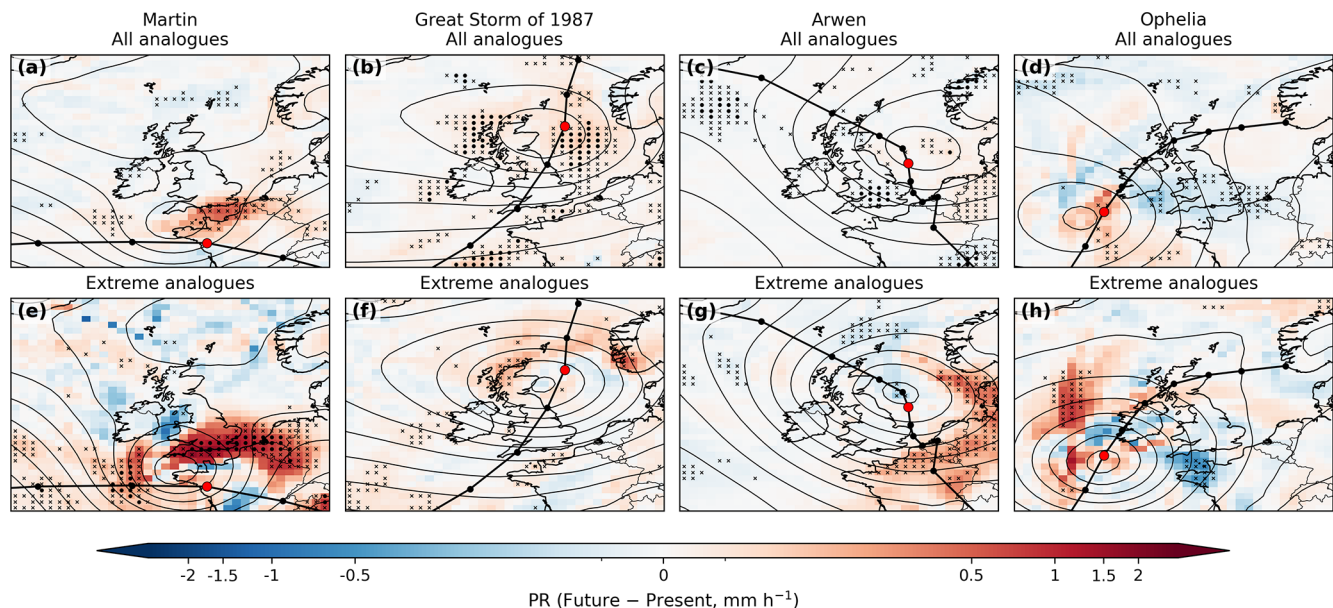
Figure 7. As Fig. 6 but for 6-h mean precipitation rate ( \text{mm h}^{-1} ) at the time of maximum intensity.
