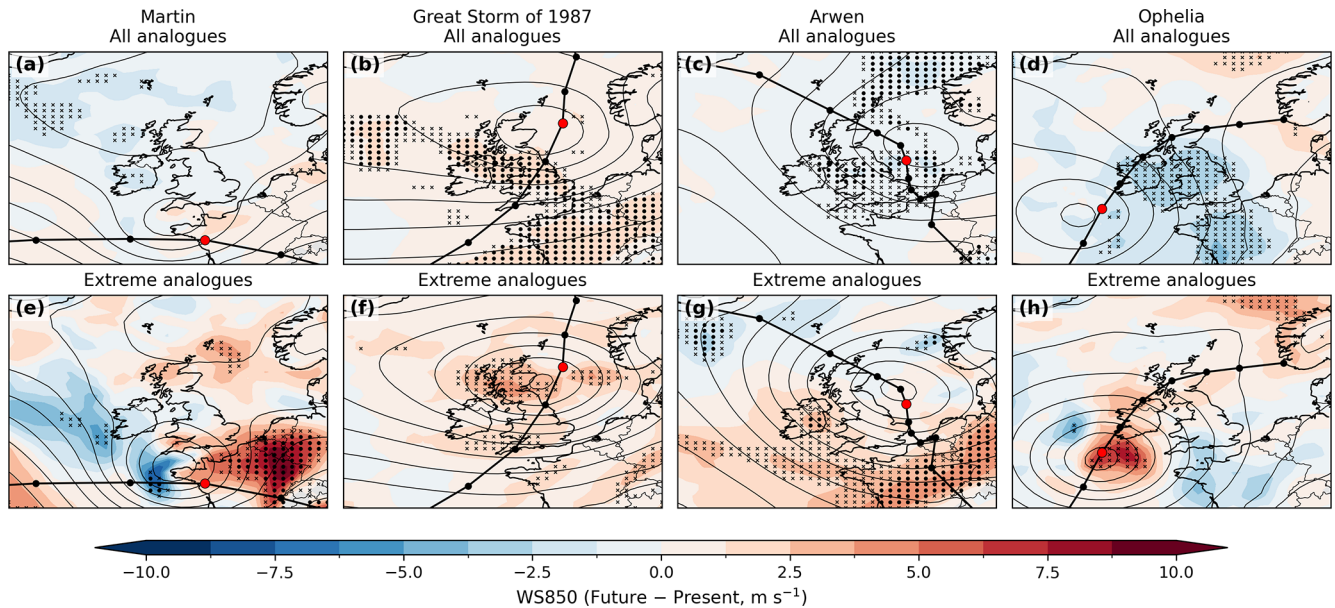
Figure 6. Composite difference plots (CANARI future–present) of wind speed at 850 hPa (shading, \text{m s}^{-1} ) for (a, e) Martin, (b, f) Great Storm of 1987, (c, g) Arwen, and (d, h) Ophelia analogues and extreme analogues at their time of maximum intensity. Black contours show the CANARI present composite SLP (intervals of 4 hPa). Stippling denotes significant regions according to the Benjamini–Hochberg false discovery rate procedure (Benjamini and Hochberg, 1995) with \alpha_{\text{FDR}} = 0.10 (Wilks, 2016) while the grid-points marked with crosses indicate local significance at the \alpha = 0.05 level, both based on a Welch’s two-sample t -test. Historical tracks are shown as black lines with the positions of maximum intensity marked by red circles.
