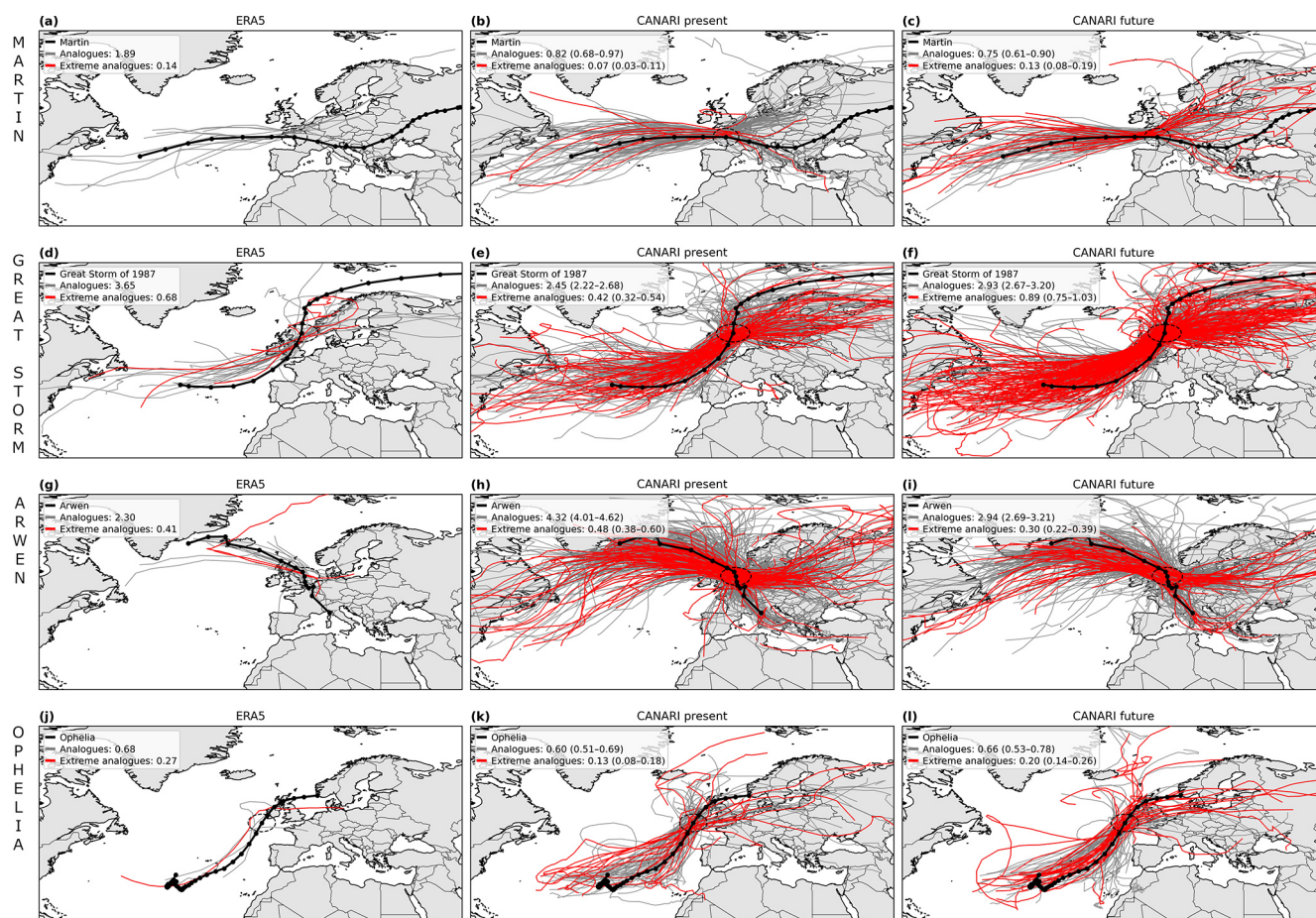
Figure 5. The full track of the case study cyclones (top to bottom) Martin, the Great Storm of 1987, Arwen and Ophelia (black lines) and their analogues (grey lines) from (a, d, g, j) ERA5, (b, e, h, k) the present-day CANARI LE, and (c, f, i, l) the future CANARI LE. Extreme analogues are marked red. The dashed circles indicate the 300 km radius used to identify the position of cyclones at peak intensity. The legends show analogue and extreme analogue rates per decade, with confidence intervals (95 %) constructed from a bootstrap resampling of the CANARI LE members.
