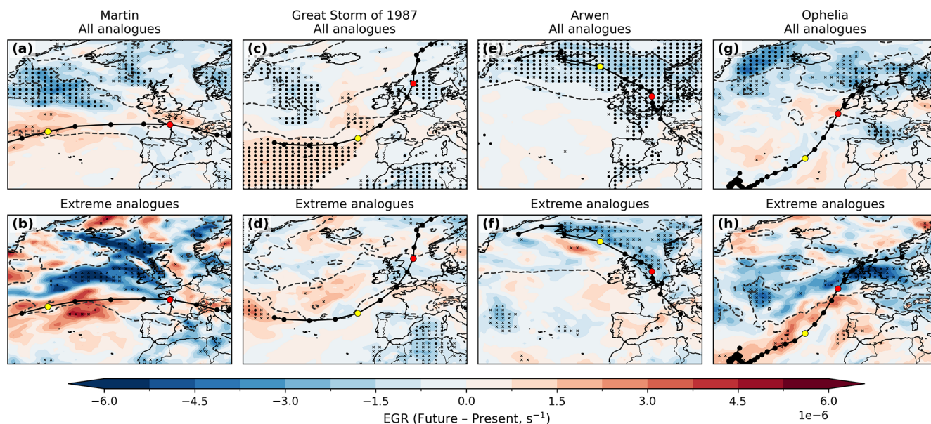
Figure 8. As Fig. 6 but for Eady growth rate (EGR, \text{s}^{-1} ) 24 h prior to the time of maximum intensity. Dashed contours show the CANARI present composite EGR and yellow circles indicate the track position 24 h prior to the time of maximum intensity.
