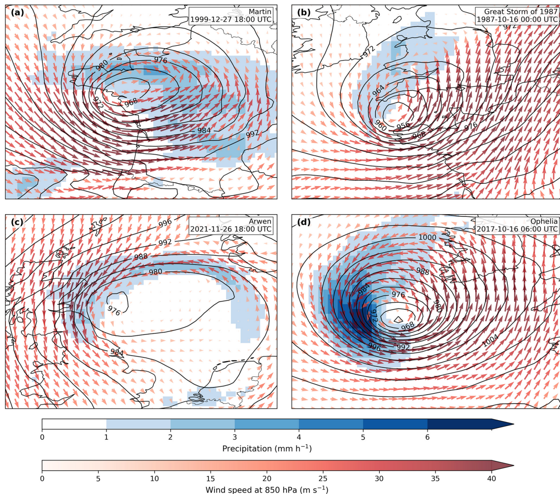
Figure 1. Sea-level pressure (hPa; black contours), 6-h mean precipitation rate ( \text{mm h}^{-1} ; shading for values \geq 1 \text{ mm h}^{-1} ), and 850-hPa wind ( \text{m s}^{-1} ); coloured wind vectors for (a) Storm Martin, (b) the Great Storm of 1987, (c) Storm Arwen, and (d) cyclone Ophelia from ERA5 reanalysis. The times shown correspond approximately to the hour of peak intensity for each cyclone, as measured by T42 850 hPa relative vorticity.
