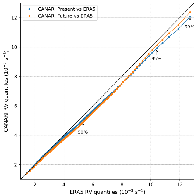
Figure 4. Comparison of the distribution of track-maximum relative vorticity in ERA5 ( x -axis; 1980–2010) and the CANARI present (blue; 1980–2010) and future (orange; 2070–2100) for all cyclones that reach peak intensity within the North-Atlantic-European region displayed in Fig. 3 ( 60^{\circ}\text{W} – 20^{\circ}\text{E} , 30^{\circ} – 70^{\circ}\text{N} ) between the months of September and April.
