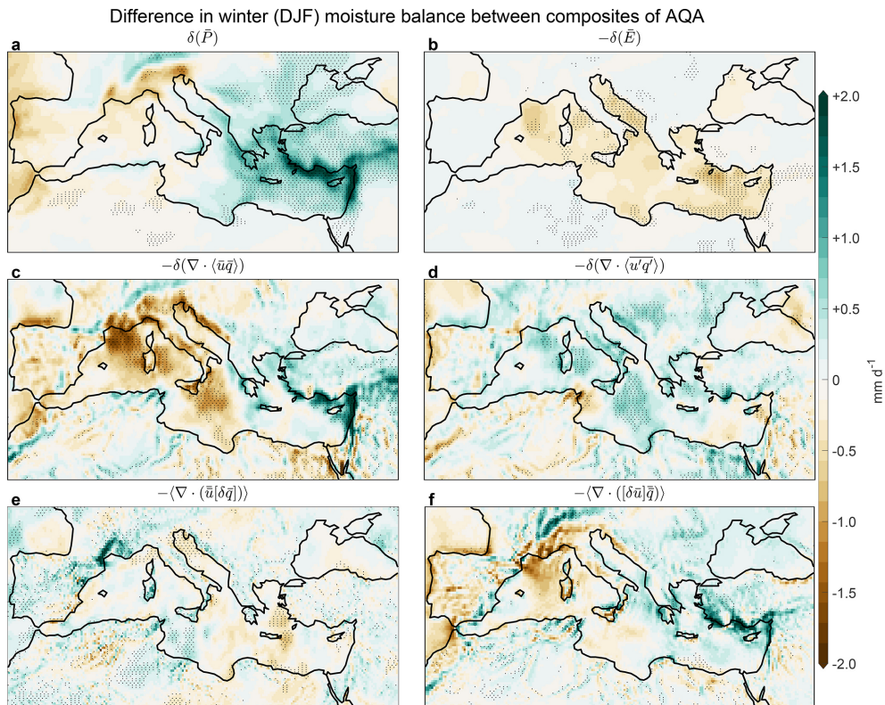
Figure 6. The decomposed hydrological balance in the Mediterranean region. Bars denote monthly means, and primes denote transient variations. Dotted regions are 95 % statistically significant using a bootstrapping test. (a) Changes in precipitation between negative and positive AQA index winter composites, respectively; (b) Changes in evaporation between composites; (c) Changes in the mean vertically integrated moisture balance; (d) Changes in the transient-eddy component of the moisture flux; (e) Changes in the mean thermodynamic component; (f) Changes in the mean dynamic component.
