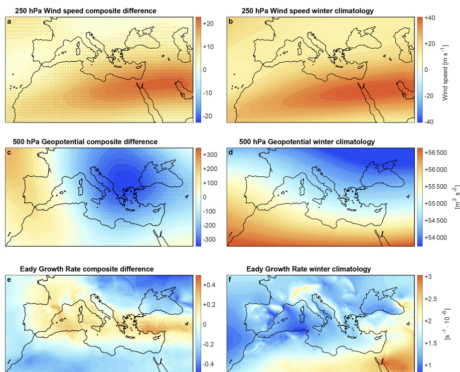
Figure 8. Composite difference between winters (December–February) preceded by negative and positive August AQA values in (a) 250 hPa wind during winter, (c) geopotential height at the 500 hPa pressure level, and (e) Eady Growth Rate. Right column panels show the respective winter climatology. Data taken from ERA5 for 1979–2023. Stippling indicates 95 % confidence estimated using a bootstrap test.
