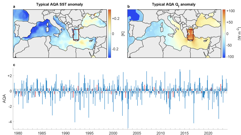
Figure 3. Aegean Q_f anomaly Index (AQA), defined as the detrended anomaly from climatology of Q_f in the Aegean Sea ( 23.5\text{--}26.5^\circ\text{E} , 32.5\text{--}35^\circ\text{N} , red rectangles in panels a and b ), normalized by the standard deviation of the anomaly timeseries. The typical difference between (a) SST and (b) Q_f positive and negative AQA months (taken as months above or below \pm 0.5 the standard deviation of AQA). (c) Monthly AQA values from January 1979 to December 2023. August months, which are the most strongly correlated with winter Levant land precipitation, are shown in red. Gray dashed horizontal lines denote \pm 0.5 the standard deviation of August AQA values.
