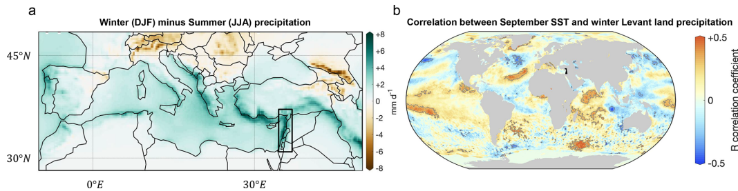
Figure 1. (a) Winter (December–February) minus summer (June–August) precipitation in the Mediterranean region; a black rectangle demarcates the Levant region considered in this study. (b) Pearson correlation coefficient of winter land precipitation in the Levant region and global sea surface temperature (SST) in the preceding September, for the period 1979–2023 (correlation 95 % confidence bounds are shown in gray contours). Data taken from the ERA5 reanalysis (Hersbach et al., 2020, see Sect. 2.1).
