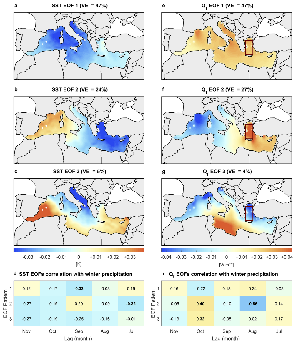
Figure 2. The first three EOF patterns of Mediterranean monthly (a–c) SST and (e–g) heat uptake ( Q_f ) anomalies. The variance explained (VE) by each pattern is shown in the panel titles. (d, h) Lagged correlation of the principal component of each monthly SST and Q_f EOF pattern, respectively, during the months July–November with mean Levant winter (DJF) land precipitation. Statistically significant (5% significance level) correlations are bolded. Data taken from ERA5 for 1979–2023 (Hersbach et al., 2020).
