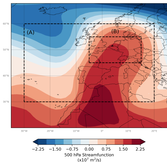
Figure 1. The 500 hPa streamfunction for the Southerly Flow event on 29 June 2019. Box (A) shows the domain used to select analogues. Box (B) shows the area over which trends for Western Europe are averaged.
