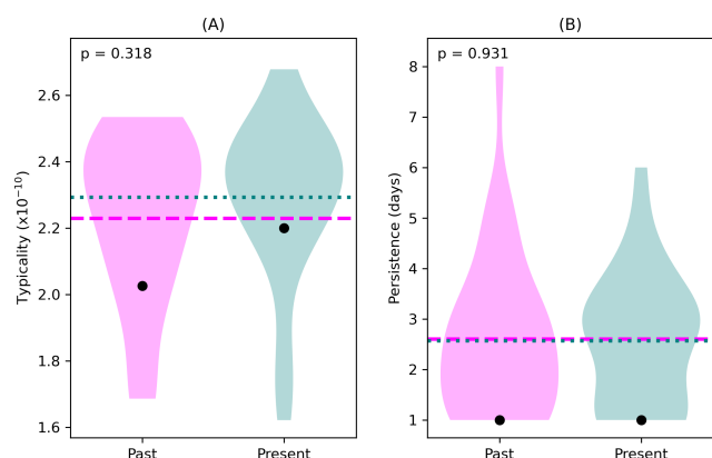
Figure 3. The changes in typicality (A) and persistence (B) for spring between the past (1950–1979) and present (1994–2023) periods. Black dots indicate the typicality and persistence of the event. The violins show the distribution of the t_{\text{analogue}} and p_{\text{analogue}} values, whose means are represented by dashed lines for the past period and dotted lines for the present period. The p -value indicates the statistical significance of the difference between these means.
