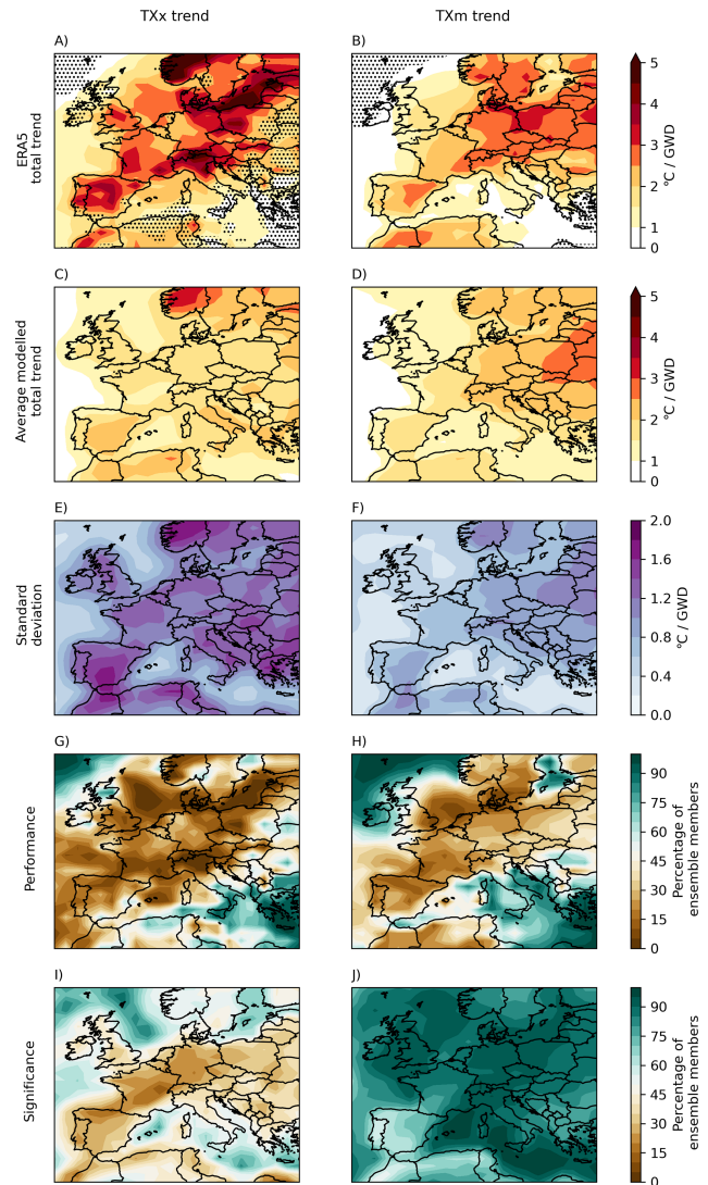
Figure 7. The ERA5 total temperature trends in the maximum (TXx) and the mean (TXm) of the daily maximum spring temperatures up to 2014, the mean trends found by the 105 model ensemble members from the HadGEM3 and MIROC6 models, the standard deviation of the modelled trends, the percentage of the ensemble members that find a trend as high as the ERA5 trend or higher, and the percentage of the ensemble members that find a trend that is statistically significant on a 95 % confidence level.
