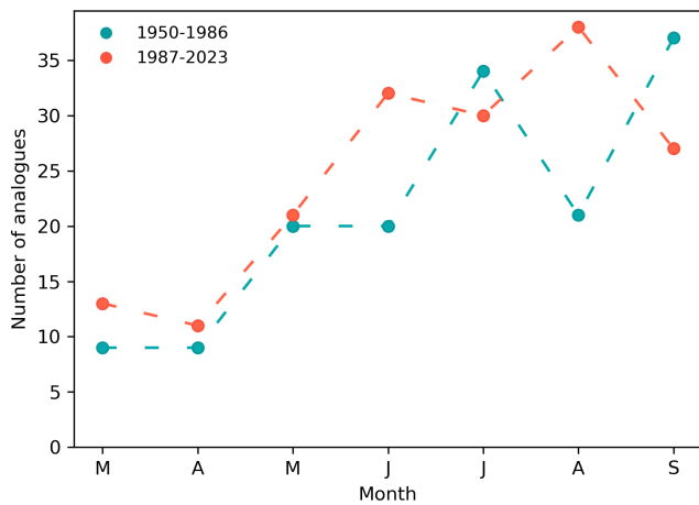
Figure 6. The distribution of analogues within the fifth percentile of Euclidean distances over different months, for two time periods.
