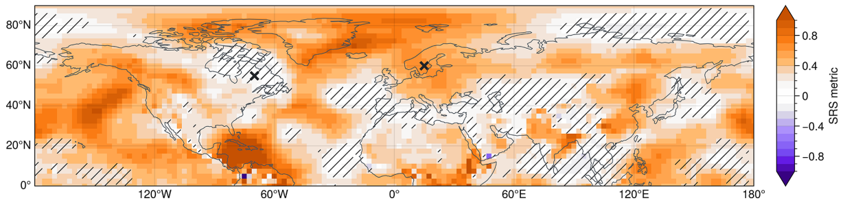
Figure 3. SRS metric computed as the slope of the linear fit to the z1000 spread-error curve at each point in the northern hemisphere. Shown are results for 50-member ensembles. Hatched areas indicate regions where the SRS metric (derived from the regression of bin-mean error on spread) is not statistically different from zero at the 99 % confidence level. Crosses indicate two example locations (eastern Canada at 55° N/70° W and northern Europe at 60° N/15° E) further analysed below.
