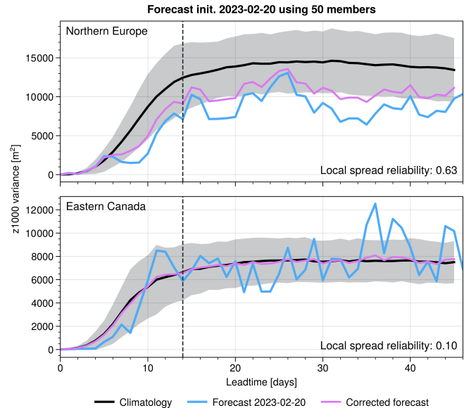
Figure 10. Evolution of z1000 ensemble variance as function leadtime at points in (a) northern Europe (60° N/15° E) and (b) eastern Canada (55° N/70° W). Black line shows climatological mean with shading indicating one standard deviation around the mean. Blue line shows variance of the example forecast initialised 20th February 2023. Pink line shows the corrected ensemble variance for that example forecast by post-processing to achieve perfect reliability.
