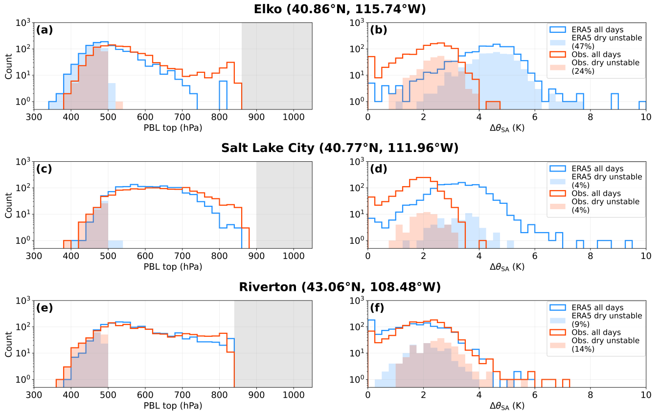
Figure S2. Characteristics of dry adiabatic bound exceedances at three sounding stations. (a, b) As in Fig. 3c. (c,d) and (e, f) As in (a, b) for the Salt Lake City and Riverton locations, respectively.
