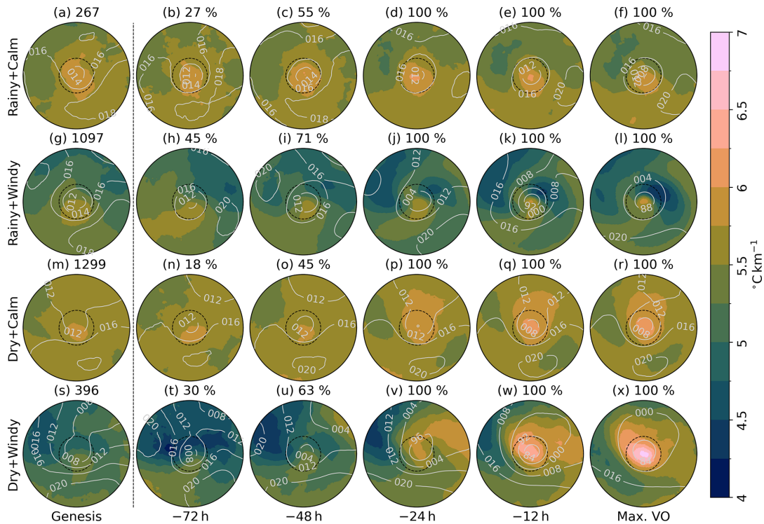
Figure 11. As in Fig. 7, with the shading showing GAMMA, defined as -[T(850\text{ hPa}) - T(500\text{ hPa})]/[Z(850\text{ hPa}) - Z(500\text{ hPa})] , where T is temperature and Z geopotential height.
