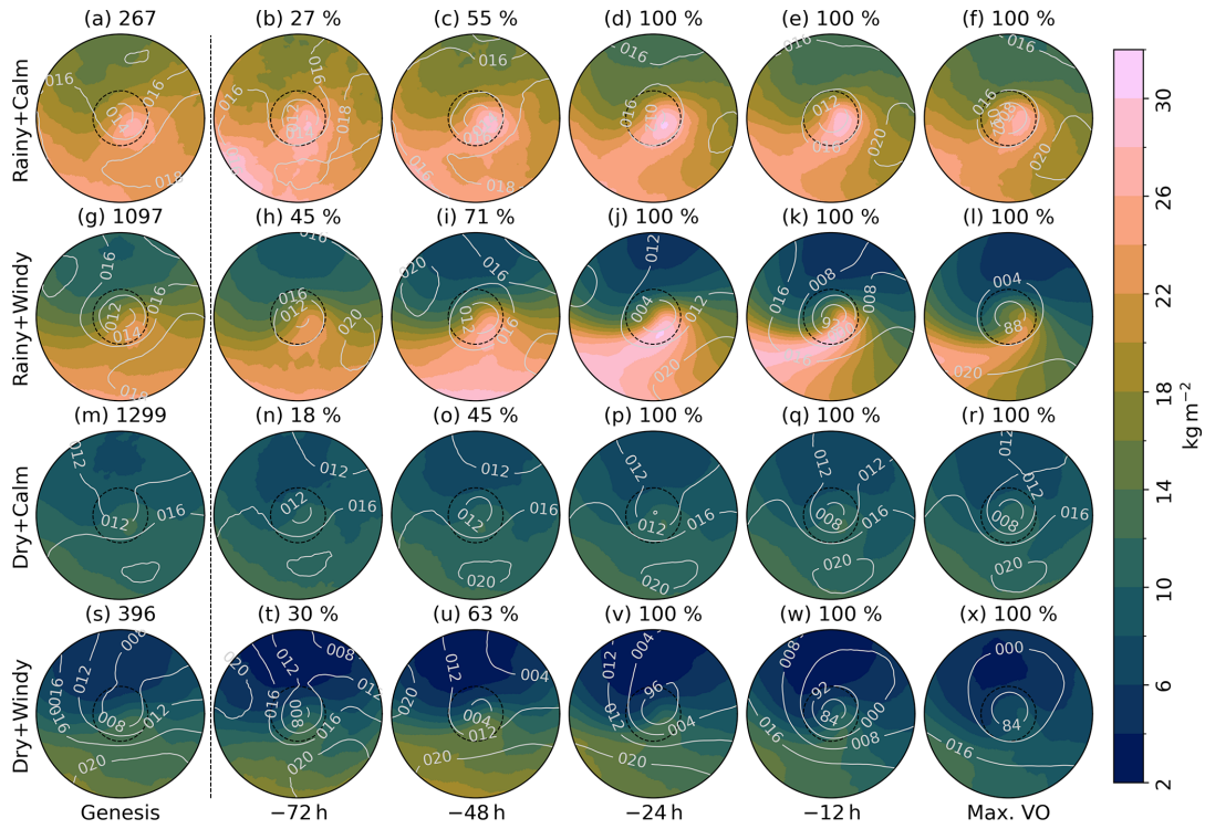
Figure 10. As in Fig. 7, with the shading showing TCWV.
