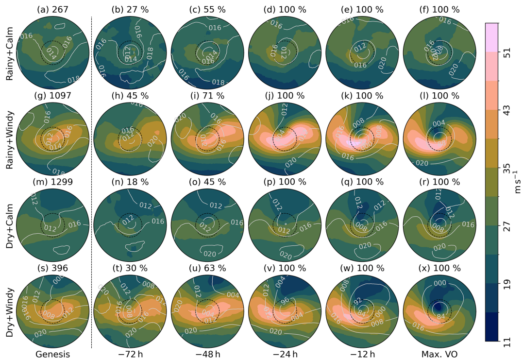
Figure 7. Composite evolution of WS300 (shading) in the four intensity groups (rows). MSLP composite is shown in the contours in hPa with the leading digit (1 or 9) omitted. The dashed black circle denotes a radius of 6^\circ geodesic and the radius of the whole circle is 18^\circ geodesic. The numbers on top of panels in the first column indicate the total size of each group. The percentages on top of other panels indicate the proportion available to sample from these sizes at a given time relative to the time of maximum VO (columns).
