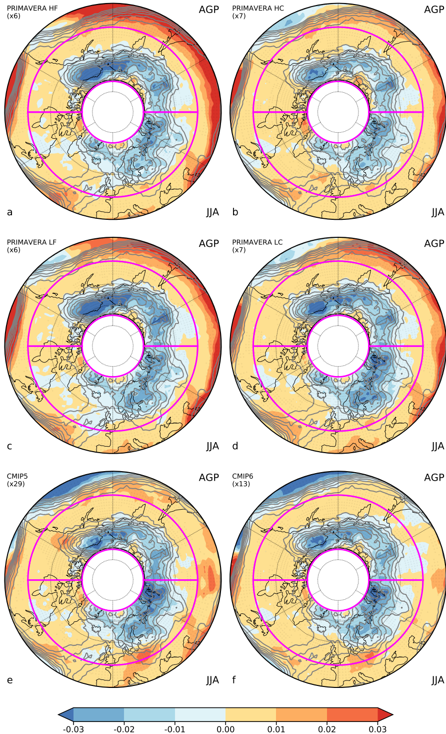
Figure 2. As Fig. 1 but for boreal summer. (Blocking frequency bias for the AGP index and (a) high-resolution forced, (b) high-resolution coupled, (c) low-resolution forced, (d) low-resolution coupled PRIMAVERA simulations, and (e) CMIP5, (f) CMIP6 simulations. Stippling shows agreement on the sign of the bias by at least (a,c) 6 of 6, (b,d) 6 of 7, (e) 19 of 29, and (f) 10 of 13 simulations. Grey contour lines show the reanalysis blocking frequency, at contour intervals of 0.01 and starting from 0.01. ATL and PAC evaluation domains are shown by magenta lines.)
