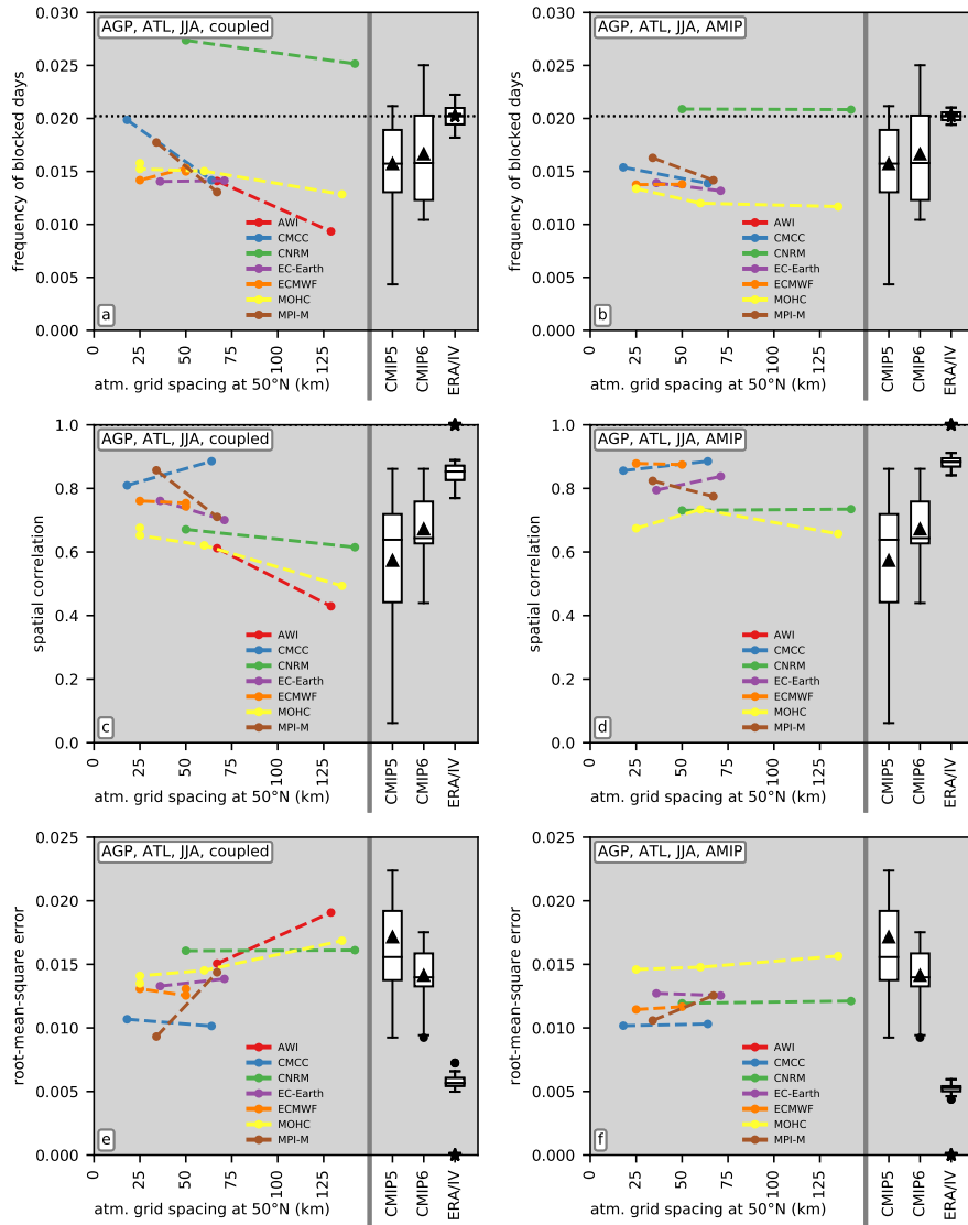
Figure 4. As Fig. 3 but for boreal summer. (Metrics of blocking performance (a,b - blocking frequency, c,d - spatial correlation, e,f - root-mean-square error) for the AGP index, for the ATL domain (-90-90E, 50-75N). The left-hand side of each panel shows metrics for PRIMAVERA simulations at different grid spacings (resolutions). Boxplots on the right-hand side show distributions of the metric across CMIP5 and CMIP6 simulations. The ‘*’ symbol in the column ‘ERA/IV’ shows the reanalysis estimate and the boxplot is an estimate of the expected agreement given internal variability (see text).)
