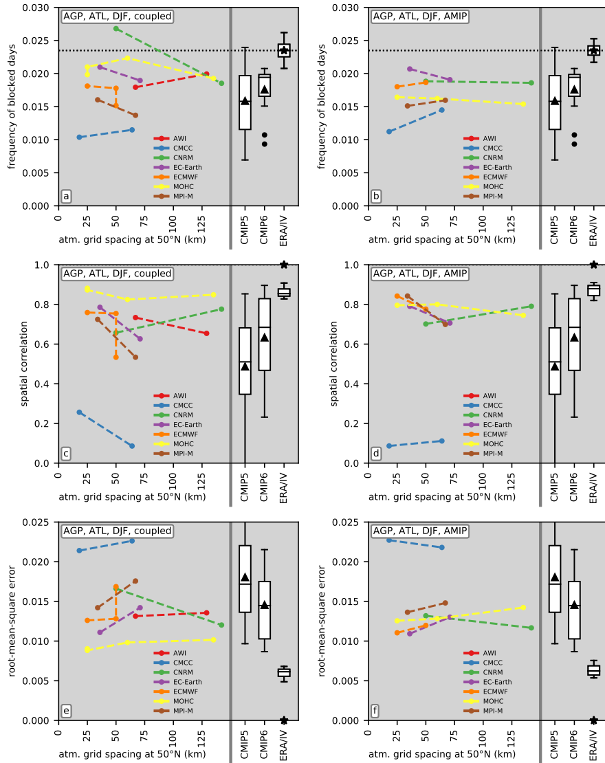
Figure 3. Metrics of blocking performance (a,b - blocking frequency, c,d - spatial correlation, e,f - root-mean-square error) for the AGP index and boreal winter, for the ATL domain (-90-90E, 50-75N). The left-hand side of each panel shows metrics for PRIMAVERA simulations at different grid spacings (resolutions). Box-and-whisker plots (boxplots hereinafter) on the right-hand side show distributions of the metric across CMIP5 and CMIP6 simulations in terms of the median, mean (triangle), interquartile range (box, IQR = Q3 - Q1 ), top whiskers extending to the last datum less than Q3 + 1.5 \times IQR , and analogously for bottom whiskers. The ‘*’ symbol in the column ‘ERA/IV’ shows the reanalysis estimate and the boxplot is an estimate of the expected agreement given internal variability (see text).
