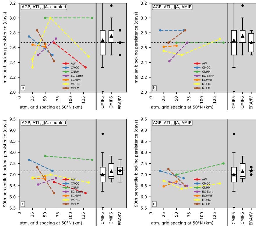
Figure 6. As Fig. 5 but for boreal summer. (Persistence of blocking events (a,b - median, c,d - 90th percentile) for the AGP index, for the ATL domain (-90-90E, 50-75N). The left-hand side of each panel shows metrics for PRIMAVERA simulations at different grid spacings (resolutions). Boxplots on the right-hand side show distributions of the persistence metric across CMIP5 and CMIP6 simulations. The '*' symbol in the column 'ERA/IV' shows the reanalysis estimate and the boxplot is an estimate of the expected agreement given internal variability (see text).)
