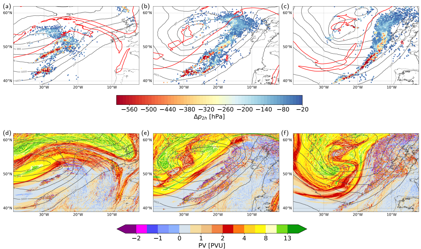
Figure 2. Overview of the WCB ascent for cyclone Vladiana : (a-c) locations of WCB air parcel ascent (circles; colors indicate centered 2-h pressure change ( \Delta p_{2h} ) along all ascending WCB trajectories, in hPa), SLP (grey contours, in hPa) and 2-PVU at 320 K (red line) for (from a to c) 22 UTC 22 Sep, 10 UTC 23 Sep, and 22 UTC 23 Sep. (d-f) PV at 320 K and SLP (grey contours, in hPa) for the same times as (a-c).
