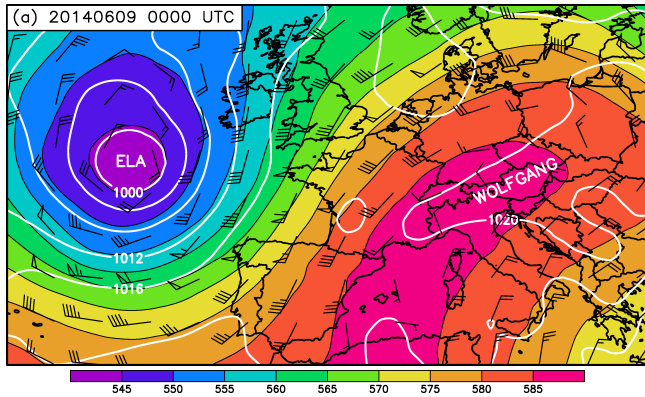
Figure 1. Global Forecast System analyses at 9 June 00:00 UTC showing 500 hPa geopotential height (gpm, shading), sea-level pressure (hPa, white contours), and 500 hPa wind barbs.
