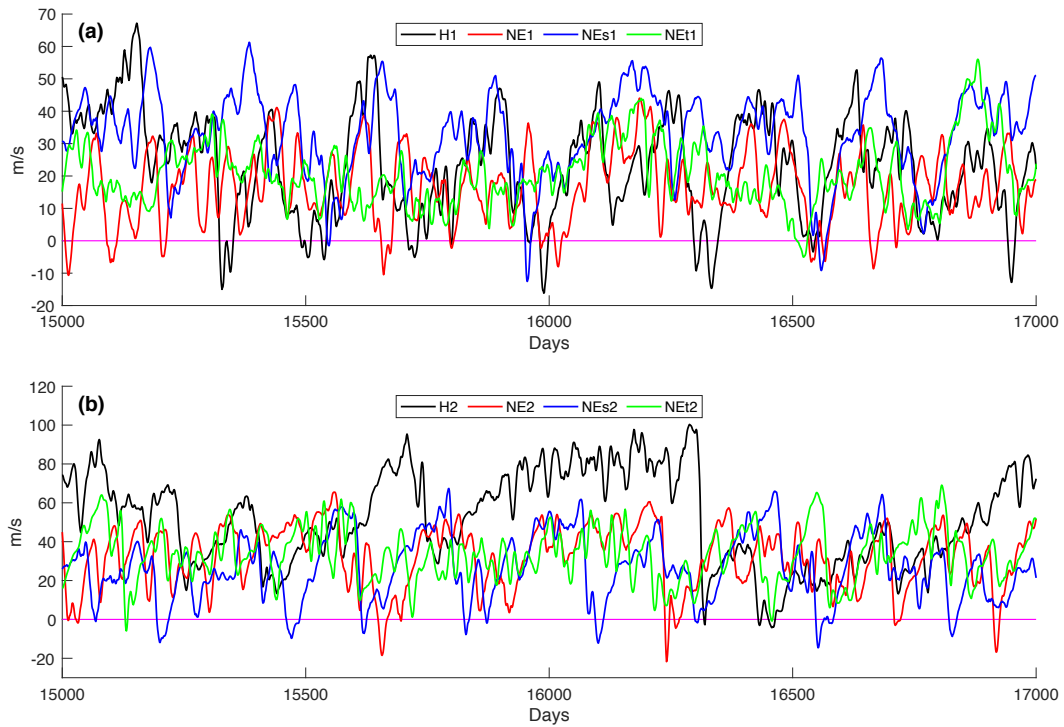
Figure 7. Zonal mean zonal wind at 10 hPa and 60° N for H1/H2 (black), NE1/NE2 (red), NEs1/NEs2 (blue) and NEt1/NEt2 (green) for model runs with wave 1 (a) and wave 2 (b) heating. The data has been smoothed with a 10 day filter. The magenta line marks 0 \text{ms}^{-1} .
