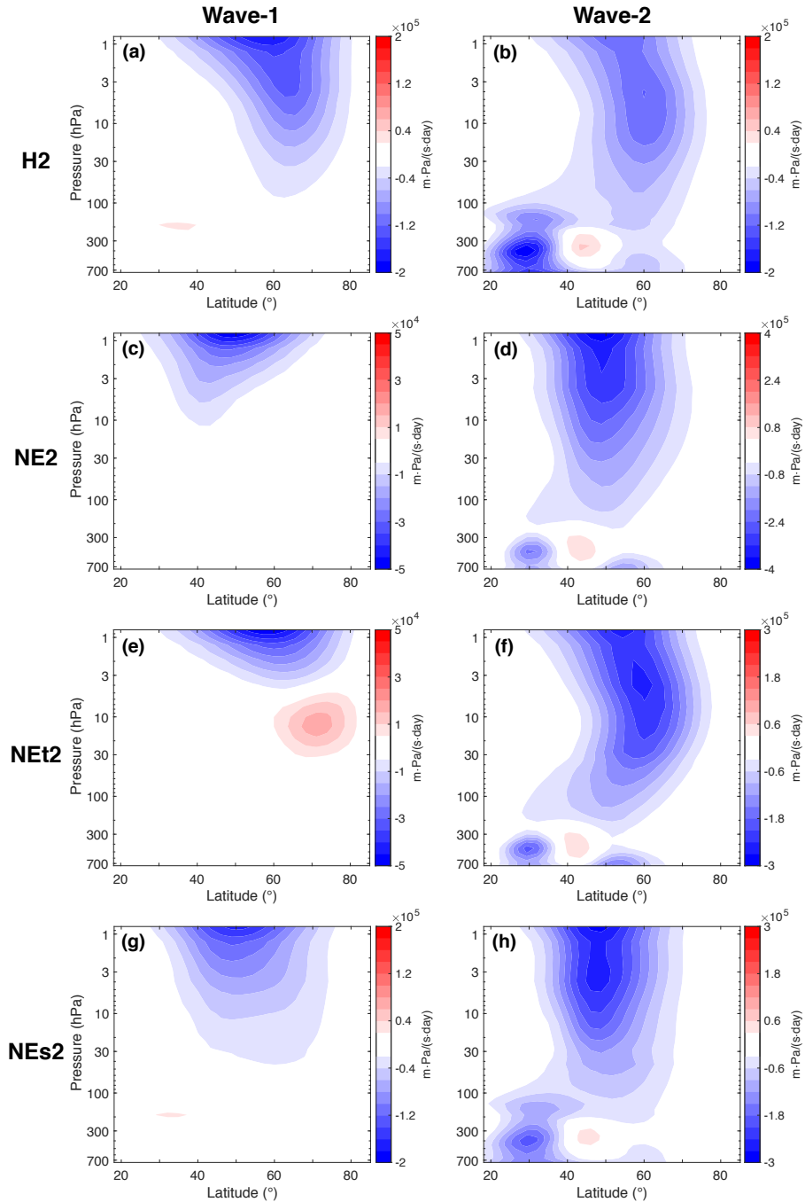
Figure 6. Vertical component of EP flux ( F_p ) for H2 (a and b), NE2 (c and d), NET2 (e and f) and NES2 (g and h). The left column shows wave 1 components, right column shows wave 2 components. Values are scaled by p_0/p , where p_0 = 1000 hPa. Contour intervals are 20 (a, b and g), 5 (c and e), 40 (d), and 30 (f and h) \text{km}\cdot\text{Pa}(\text{s}\cdot\text{day})^{-1} .
