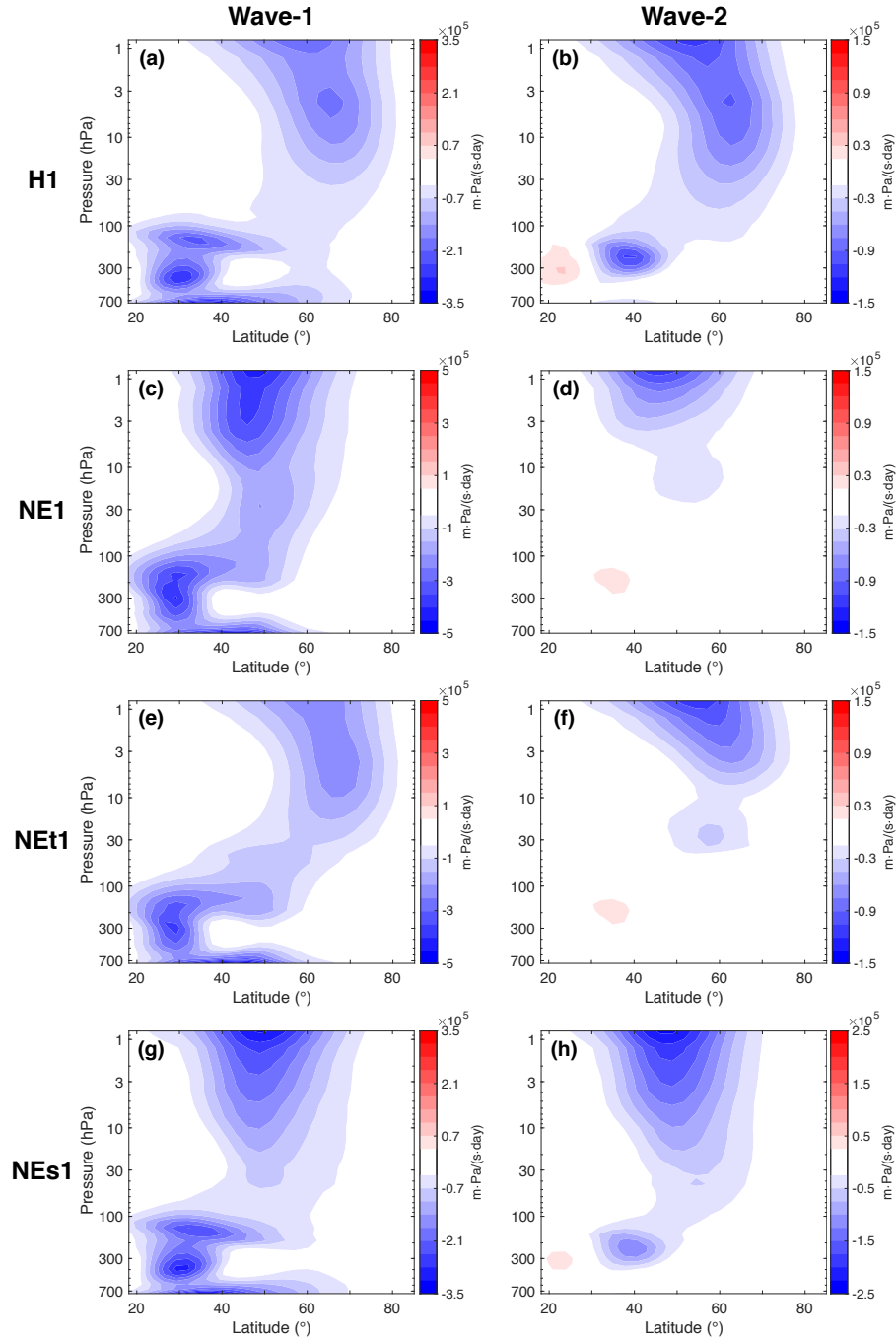
Figure 5. Vertical component of EP flux ( F_p ) for H1 (a and b), NE1 (c and d), NET1 (e and f) and NES1 (g and h). The left column shows wave 1 components, right column shows wave 2 components. Values are scaled by p_0/p , where p_0 = 1000 hPa. Contour intervals are 35 (a and g), 15 (b, d and f), 50 (c and e), and 25 (h) \text{km}\cdot\text{Pa}(\text{s}\cdot\text{day})^{-1} .
