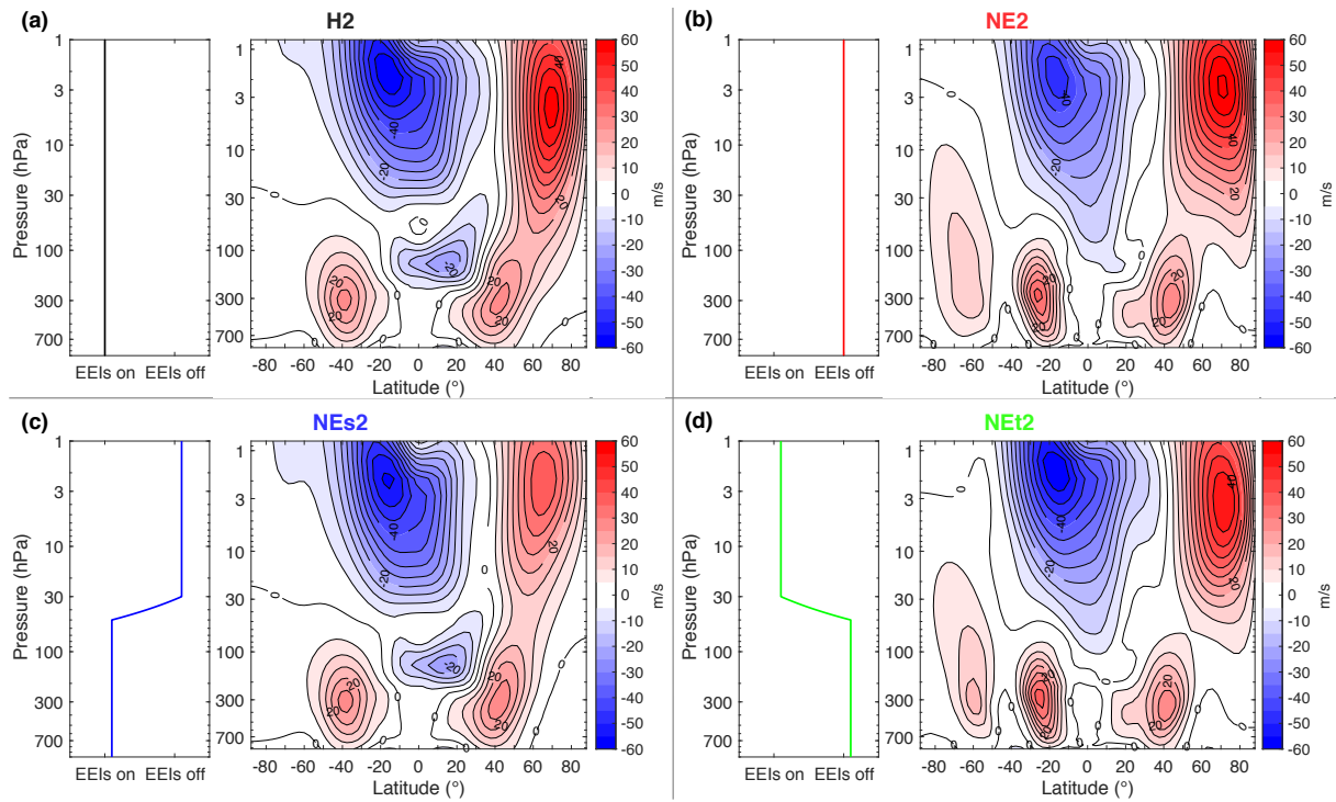
Figure 2. Zonal mean zonal winds for H2 (a), NE2 (b), NEs2 (c) and NEt2 (d), with panels showing the pressure levels where EEIs are allowed. The contour interval is 5 \text{ ms}^{-1} .
