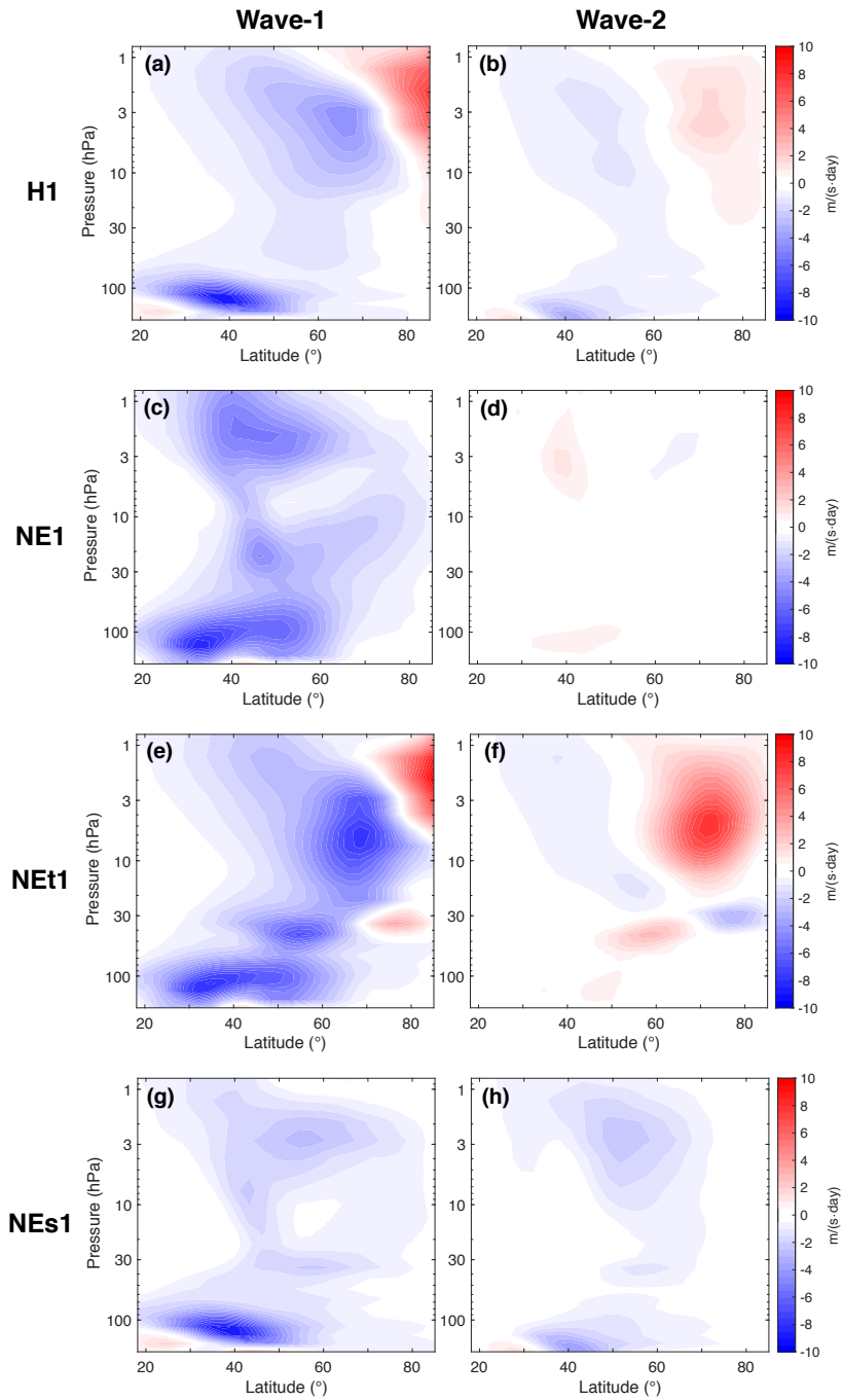
Figure 3. Divergence of EP flux for H1 (a and b), NE1 (c and d), NEt1 (e and f) and NEs1 (g and h). The left column shows wave 1 components, right column shows wave 2 components. The contour interval is 0.5 \text{ m}(\text{s}\cdot\text{day})^{-1} .
