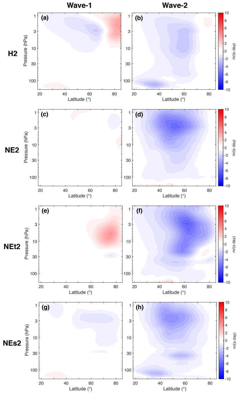
Figure 4. Divergence of EP flux for H2 (a and b), NE2 (c and d), NET2 (e and f) and NES2 (g and h). The left column shows wave 1 components, right column shows wave 2 components. The contour interval is 0.5 \text{ m}(\text{s}\cdot\text{day})^{-1} .
