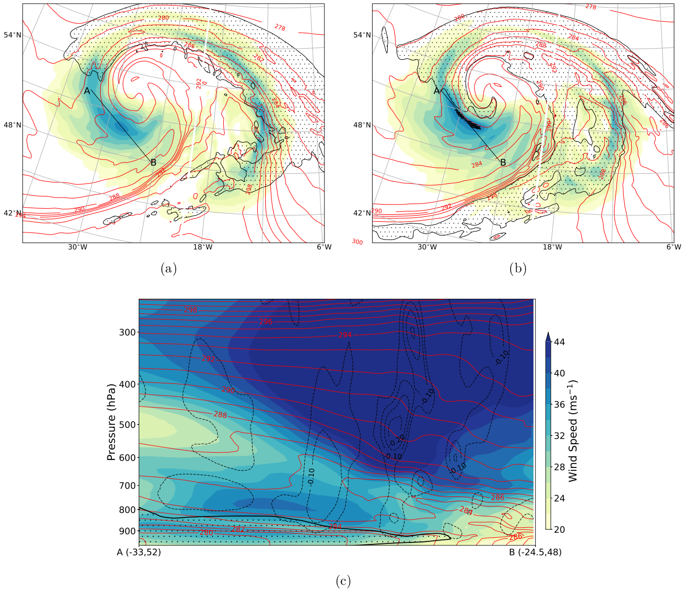
Figure 3. (a) Wind speed at 850 hPa (shading, \text{m s}^{-1} ), \theta_w at 850 hPa (K, red lines) and cloudy regions at 700 hPa ( \text{RH}_{ice} > 80\% , black lines and dotted regions) after 94 hours from the start of the control simulation (as all the other panels in this figure). Note that the model domain (whose original zonal extension goes from 20°W to 25°E with periodic E-W boundary conditions) is repeated zonally to facilitate visualisation but only data between 45°W and 5°W are shown here. (b) Same as (a) but at 805 hPa for all fields. Black dots show the horizontal locations of SJ trajectories. (c) Cross section (transect AB in panel (a)) of wind speed (green filled contours), negative vertical velocity (dashed black lines, \text{m s}^{-1} ), \theta_w (red lines, K) and cloudy regions ( \text{RH}_{ice} > 80\% , thick black lines).
