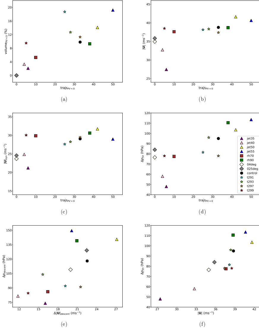
Figure 12. Scatterplots showing, for all the sensitivity experiments: (a) volume_{PV<0} against trajSPV<0 , (b) |U| against trajSPV<0 , (c) |U|_{sys} against trajSPV<0 , (d) \Delta p_{5h} against trajSPV<0 , (e) \Delta p_{descent} against \Delta|U|_{descent} and (f) \Delta p_{5h} against |U| . trajSPV<0 is the maximum number of trajectories of the 100 selected with negative PV at any instant within 15 hours from the time when the trajectories are selected (i.e. identification time) and volume_{PV<0} indicates the maximum percentage of grid points with negative PV, evaluated in the same time window as trajSPV<0 , in a volume centred on the location of the median of trajectories and extending for 20 grid points in latitude, 40 grid points in longitude and 3 vertical pressure levels (note that the symbols for the reduced resolution simulations overlie at point (0,0) in panel (a)). |U| is the maximum Earth-relative speed, |U|_{sys} is the system-relative speed at the time when |U| is reached, \Delta p_{5h} is the maximum five-hour pressure increase in a period ending by identification time. \Delta p_{descent} and \Delta|U|_{descent} indicate, respectively, total pressure increase and speed increment during the whole SJ descent, whose end is taken at identification time and whose start has to be not more than twelve hours before. All these kinematic quantities refer to the median of trajectories.
