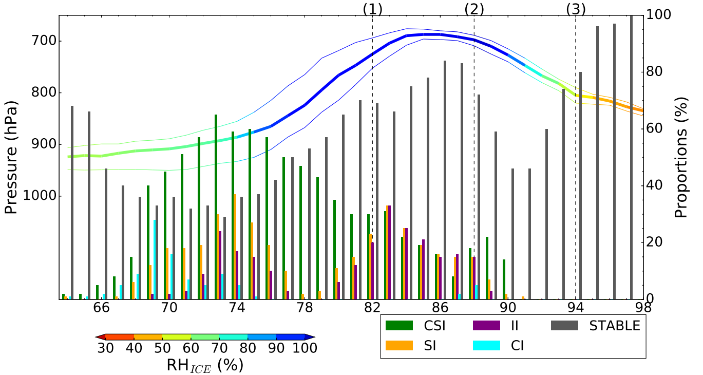
Figure 5. Timeseries (hours since start of run) of pressure (colours indicate relative humidity w.r.t. ice) and diagnosis of instability conditions along the trajectories in coloured bars. See section 2.2 for details on instability diagnostics.
