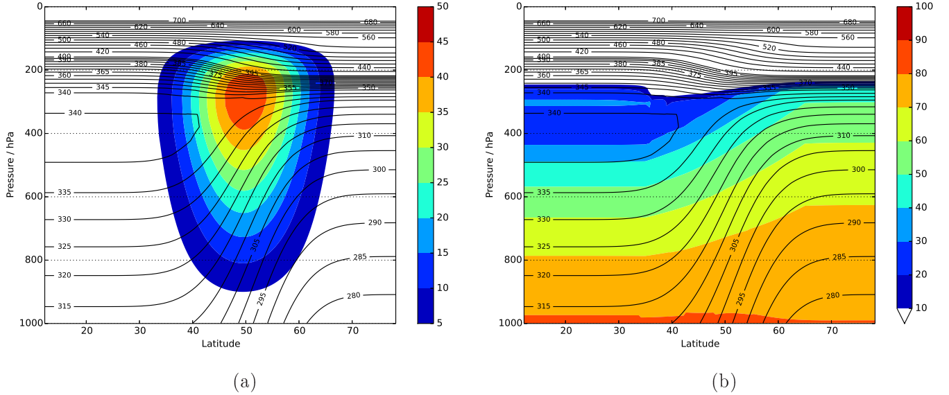
Figure 1. Initial potential temperature and (a) zonal wind, (b) relative humidity using setup according to Baker et al. (2014) but with m_v = 10^{-8} in the stratosphere and \Gamma_S = 0.025 , and our revised profile correction method. Note \theta contour interval changes from 5 K to 20 K at 400 K.
