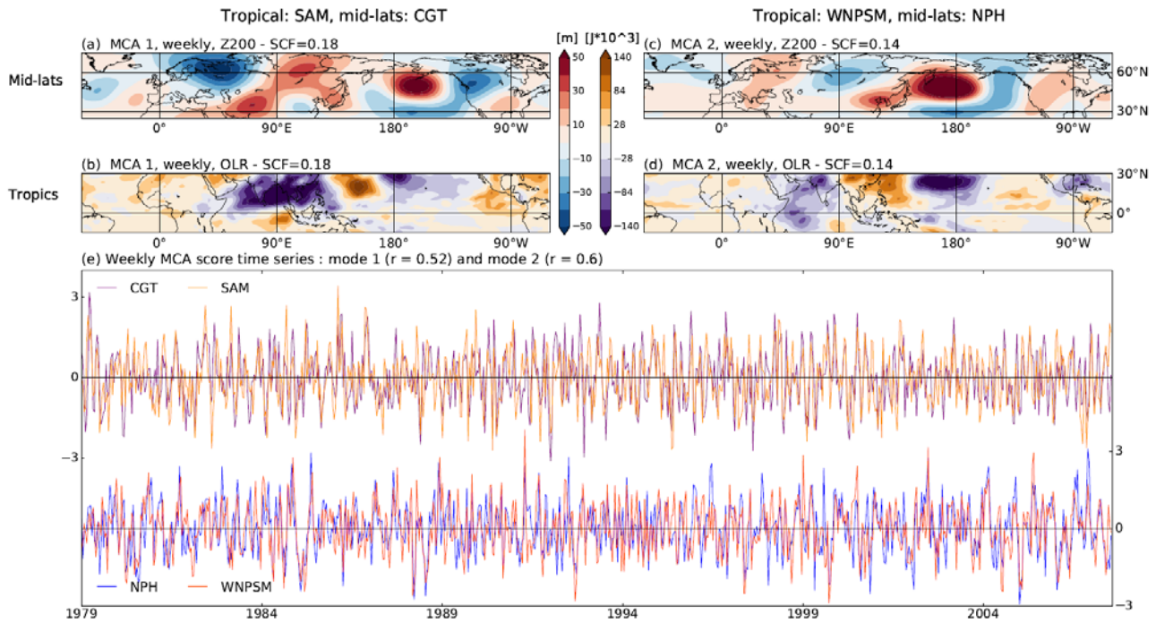
Figure 2: MCA of mid-latitude Z200 and tropical OLR at intraseasonal timescales. Panels (a) and (b) show the first MCA mode for mid-latitude Z200 (25-75° N) and tropical OLR (15°S-30°N), respectively, at the weekly timescale. The first MCA highlights the circumglobal teleconnection (CGT) pattern in the mid-latitudes and the South Asian monsoon (SAM) in the tropical belt. Panels (c) and (d): Same as for panel (a) and (b) but for the second MCA mode. This mode depicts the North Pacific High (NPH) in the mid-latitudes and the western North Pacific summer monsoon (WNPSM) in the tropical belt. The squared covariance fraction (SCF) of each MCA mode is given on top of the panels. Panel (e) shows the time series of MCA scores for the two MCA modes at weekly timescale. Each MCA pattern has its own time series, i.e. one for tropical OLR and one for mid-latitude Z200 (note that different y-axes are used).
