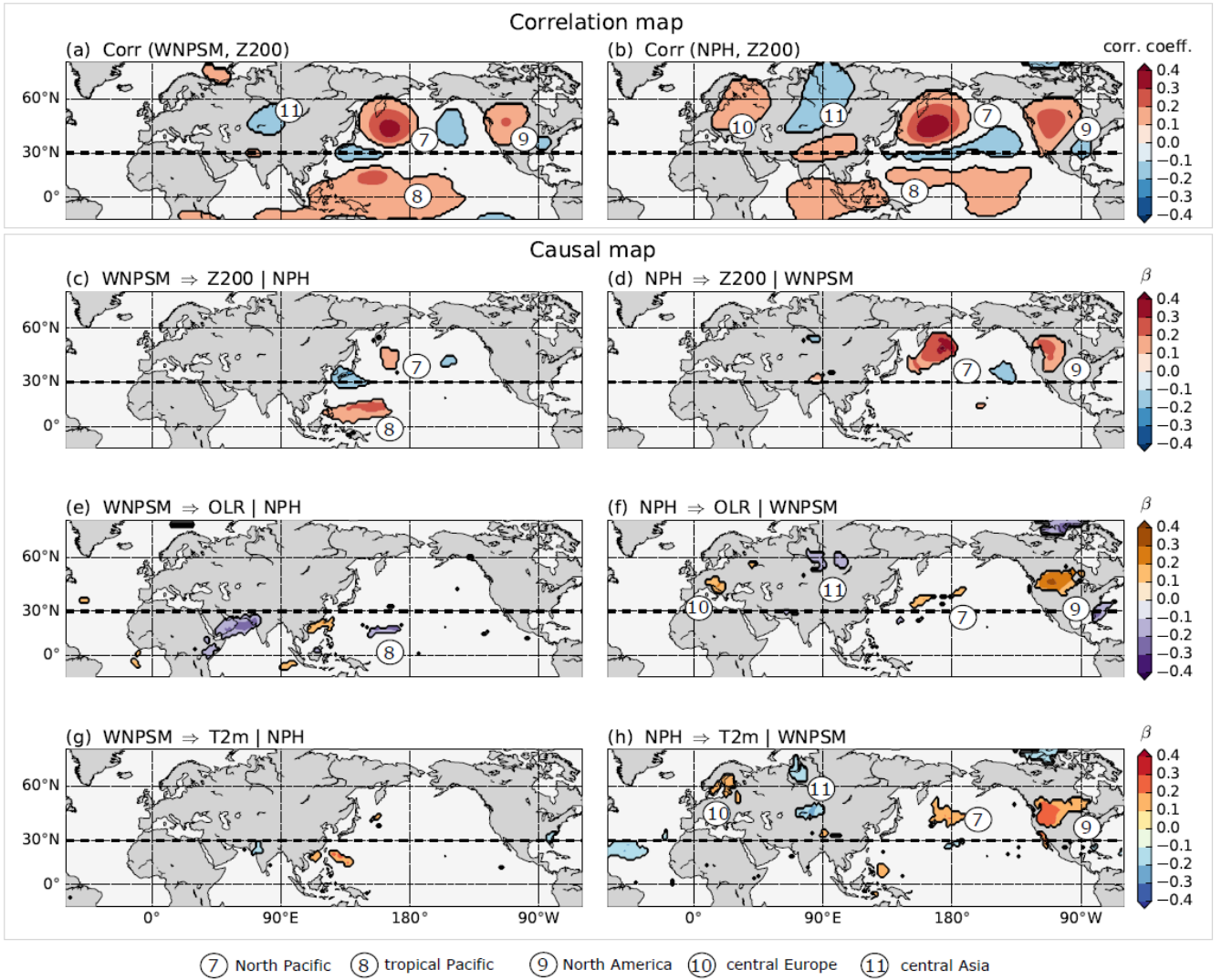
Figure 4: Influence of MCA mode 2 on Northern Hemisphere circulation. Panel (a): Correlation between the weekly WNPSM time series and the Z200 field. Panel (b): Same as panel (a) but for the correlation between weekly NPH time series and the Z200 field. Panel (c): Path coefficient \beta for the link \text{WNPSM}_{\tau=-1} \rightarrow \text{Z200}_{\tau=0} in a 3-actors CEN built with WNPSM, NPH and Z200. Here, the “|” denotes the conditioned-out actor: NPH. Panel (d): Same as panel (c) but for the link \text{NPH}_{\tau=-1} \rightarrow \text{Z200}_{\tau=0} . Here, the “|” denotes the conditioned-out actor: WNPSM. Panels (e) and (g): Same as panel (c) but for the influence of WNPSM on OLR and T2m fields respectively. Panels (f) and (h): Same as panel (d) but for the influence of NPH on OLR and T2m fields respectively. Only path coefficients \beta with p < 0.05 (accounting for the effect of serial correlations) and the robustness mask (see Fig. S9 in the Supplementary Material) are shown. The dashed black line located at 30^\circ\text{N} shows the border between the tropical and the mid-latitude belt which separates OLR and Z200 analysis.
